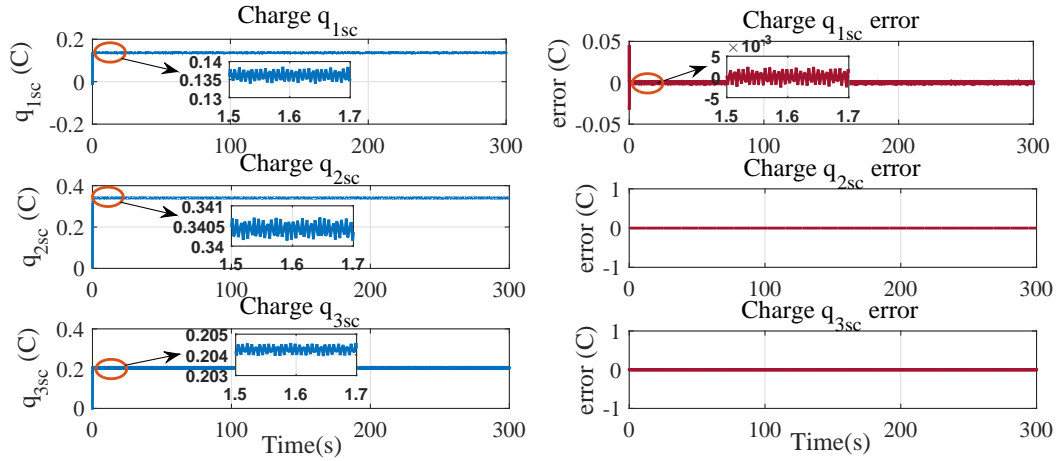
Figure A.2.4: Charge states of the capacitors C_{1sc} , C_{2sc} and C_{3sc} of the Split-Pi converter in function of the flat outputs generated by the algorithm in (3.3.28). The error between the charge states of (3.3.29c), (3.3.42c), (3.3.42d), (3.3.42e) and of (3.3.32c), (3.3.32d), (3.3.32e) is depicted.
