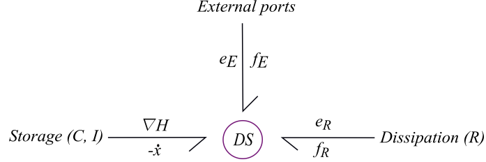
Figure 2.3.12: Dirac structure of a port-Hamiltonian system.
