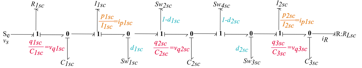
Figure 2.4.7: Bond graph of the Split-Pi converter.
