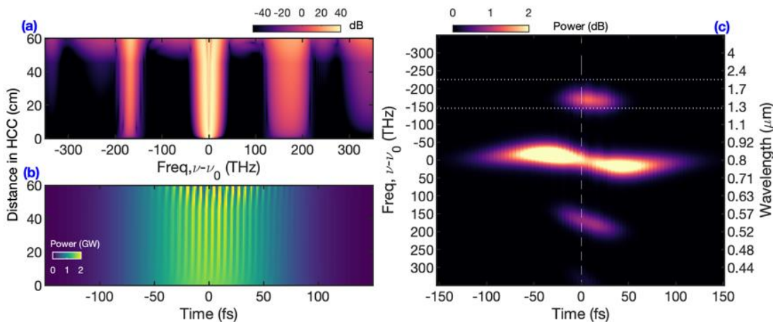
Fig. 4.16 a), b) Spectral and temporal evolution in a 60 cm-long HCC filled with an argon gas at 1.2 bar. c) Spectrogram of the output pulse of the 60 cm long HCC filled with 1.2 bar argon.
