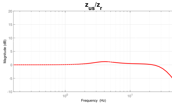
Figure 6.14: Transfer \|z_{us}/z_r\| -Passive damper
