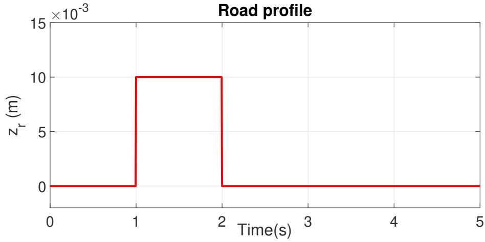
Figure 6.18: Road profile
