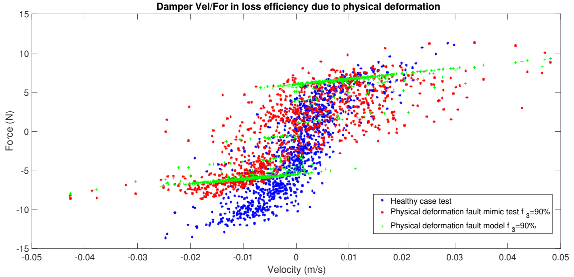
Figure 6.9: Physical deformation: Force vs. Velocity diagram - measurement vs. model
