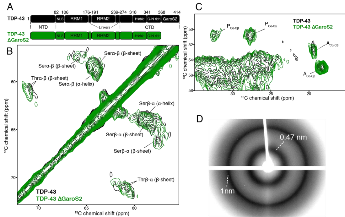
Figure 3.9 (A) Sequence construction strategy of TDP-43 \Delta GaroS2 that corresponds to TDP-431–366. (B-C) overlaid ^{13}\text{C} - ^{13}\text{C} PDS correlation spectra of TDP-43 \Delta GaroS2 (in green) and TDP-43 (in black) highlighted for the Ser/Thr \text{C}\alpha - \text{C}\beta region (B) and Ala \text{C}\alpha - \text{C}\beta (C) region recorded at a ^1\text{H} frequency of 600 MHz, 11 kHz MAS frequency, and a mixing time of 50 ms at 278 K, with the calculated secondary structure of the residue in the bracket. (D) X-ray diffraction pattern of TDP-43 \Delta GaroS2 filaments showing characteristic cross- \beta diffraction pattern in amyloid fibrils. Reflections at 4.7 Å and 10 Å are highlighted, corresponding to the inter-strand and inter-sheet spacing, respectively.
