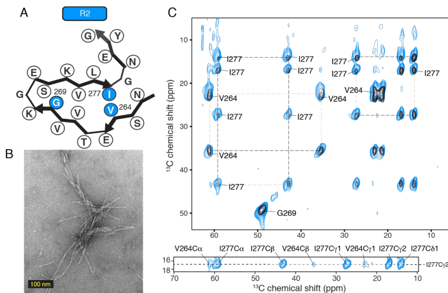
Figure 4.5 R2 repeat forms amyloid fibrils and adopts b-solenoid fold. A) Schematic representation of R2 labeling strategy, made of three 13 C-labeled amino acids (Val264, Gly269, and Ile277). B) Negatively stained electron micrographs of R2 fibrils, scale bar, is 100 nm. C) On top: two-dimensional solid-state
