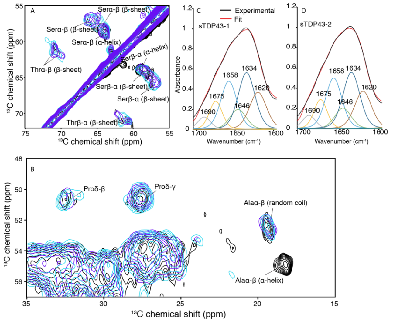
Figure 3.21 Overlaid ^{13}\text{C} - ^{13}\text{C} PDS correlation spectra of sTDP43-1 (cyan), sTDP43-2 (violet) and TDP-43 (black) highlighted for the A) Ala \text{C}\alpha - \text{C}\beta B) Ser/Thr \text{C}\alpha - \text{C}\beta region. FTIR spectra of C) sTDP43-1 D) sTDP43-2 aggregates in the amide I and II range showing the experimental (black) and theoretically fitted curve (red).
