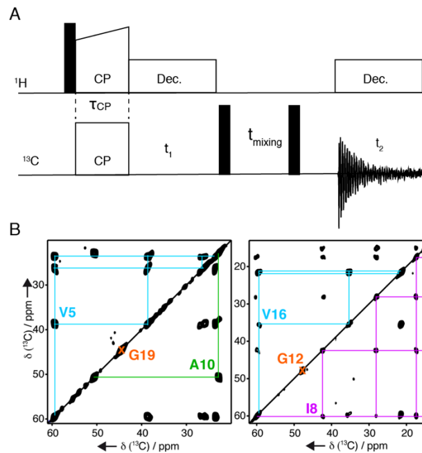
Figure 2.2 A) The 2D ^{13}\text{C} - ^{13}\text{C} PDSD pulse sequence with the mixing time t_{mix} used for the ^{13}\text{C} - ^{13}\text{C} transfer, here we used the PDSD scheme. The black rectangle represents the 90^\circ pulse, and an open rectangle represents the 180^\circ pulse. B) Two-dimensional solid-state NMR ^{13}\text{C} - ^{13}\text{C} correlation spectra of NWD2(3–23) fibrils, isotopically ^{13}\text{C} labeled on Val5, Ala10, Gly19 (left) and Ile8, Gly12, Val16 (right), intra-residue correlations are shown. (Figure adapted from Daskalov et al. 317 )
