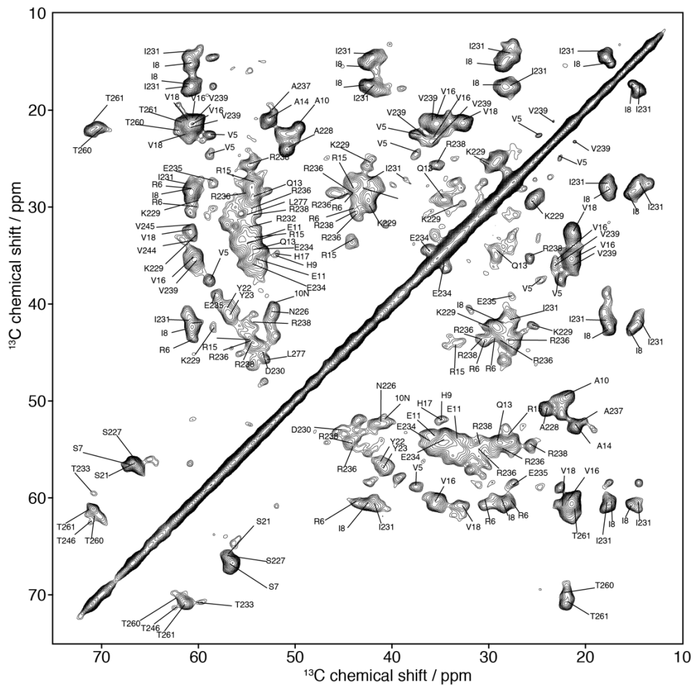
SI Figure 4.4 Solid-state NMR ^{13}\text{C} - ^{13}\text{C} correlation experiment of the aliphatic region of R0-R1 fibrils recorded at a ^1\text{H} frequency of 600 MHz, 11 kHz MAS, with a PSD mixing time of 50 ms at 278K.
