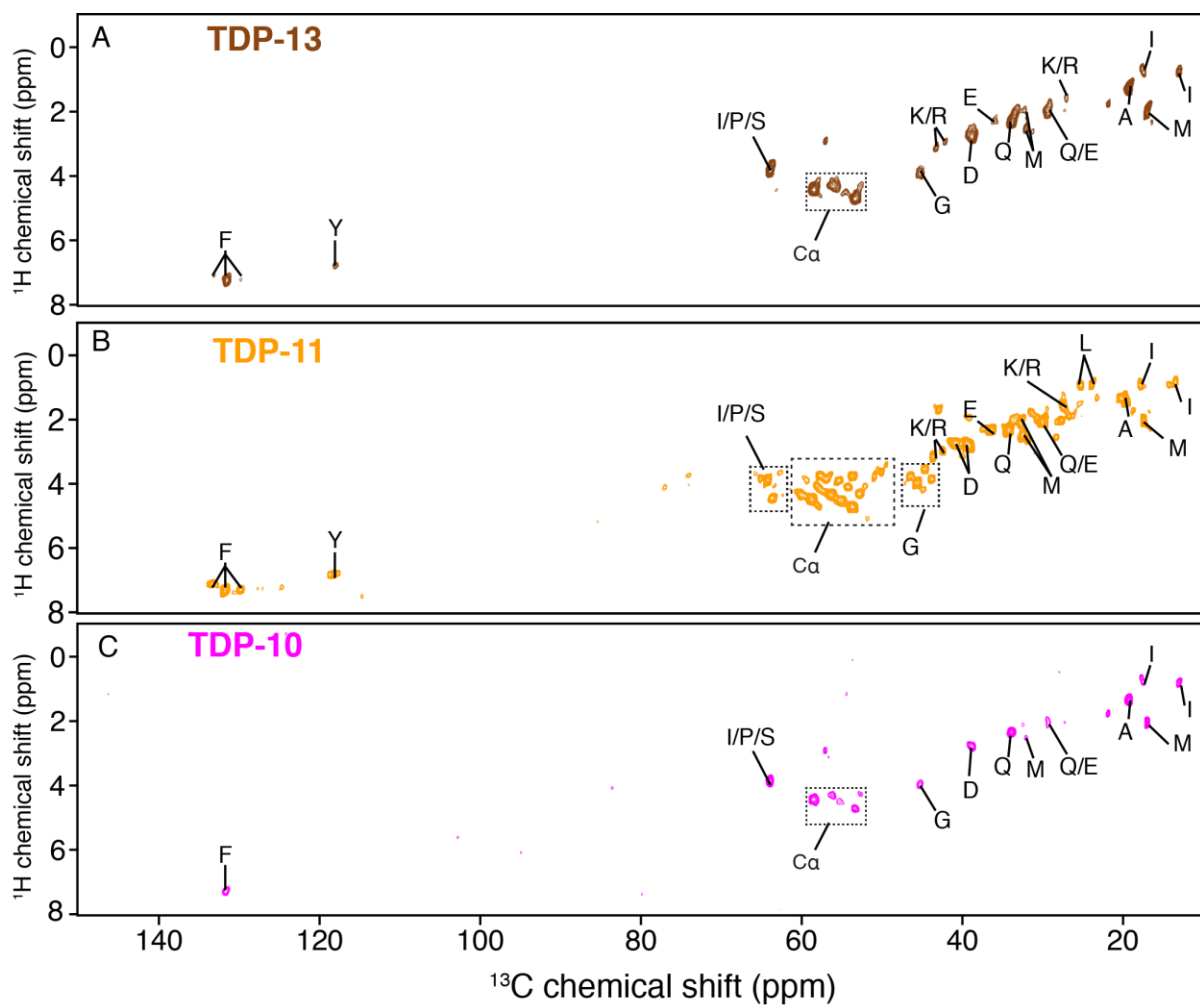
Figure 3.12 SSNMR ^1\text{H} - ^{13}\text{C} INEPT spectra of A) TDP-13 (brown), B) TDP-11 (orange), and C) TDP-10 (pink) amyloid aggregates showing tentative assignments corresponding to residues in the
