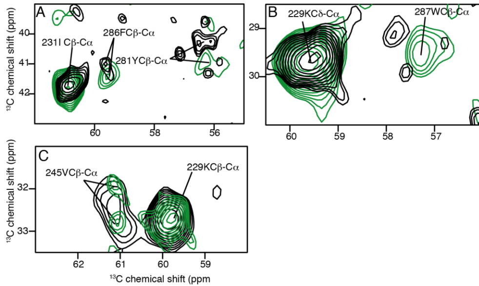
Figure 5.4 Representative excerpt of regions of 2D- ^{13}\text{C} - ^{13}\text{C} correlation spectra with PDS mixing time of 50ms, indicating CSP for ThT bound (green) and free (black) HET-s(218-289) fibrils.
