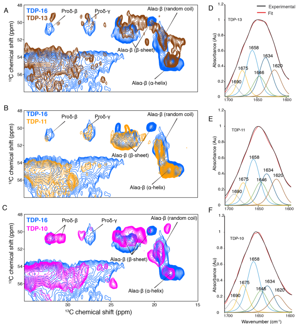
Figure 3.14 An excerpt from the overlay of the 2D ^{13}\text{C} - ^{13}\text{C} PDS correlation spectra with a mixing time of 50 ms PDS recoupling obtained on ( U - ^{13}\text{C} , ^{15}\text{N} )-labeled samples of (A) TDP-13(brown), (B) TDP-11(orange), and (C) TDP-10 (pink) compared with TDP-16 (blue) recorded at 278 K and a ^1\text{H} frequency of 600 MHz, 11 kHz MAS frequency, a mixing time of 50 ms. Labels indicate characteristic alanine \text{C}\alpha - \text{C}\beta and proline \text{C}\delta - \text{C}\beta correlations and chemical shift-dependent secondary structure in brackets. FTIR spectra of (D) TDP-13, (E) TDP-11, and (F) TDP-10 aggregates in the amide I and II range showing the experimental (black) and theoretically fitted curve (red).
