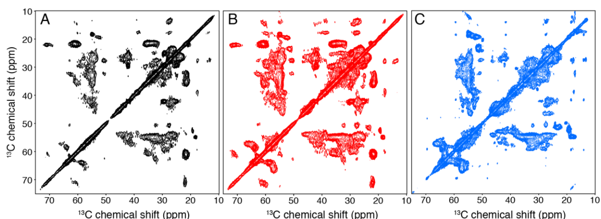
Figure 3.3 Solid-state nuclear magnetic resonance ^{13}\text{C} - ^{13}\text{C} correlation spectra of the different self-assembled [U-^{13}\text{C}, ^{15}\text{N}] -labeled TDP fibrillar assemblies, the carbon-carbon magnetization transfer is achieved by a proton-driven ^{13}\text{C} - ^{13}\text{C} spin diffusion. The aliphatic region of (A) full-length TDP-43 (black), (B) the TDP-35 construct (red), and (C) the TDP-16 construct (blue) recorded at 278 K at a ^1\text{H} Larmor frequency of 600 and 800 MHz, respectively, at 11 kHz MAS
