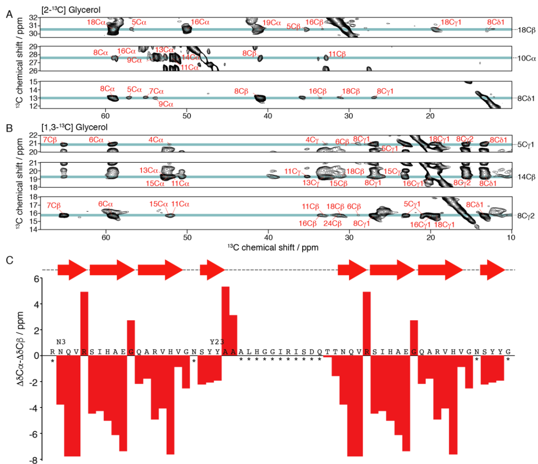
Figure 4.3 Secondary structure of the chimeric R0-R0 functional amyloids. A) Two-dimensional solid-state NMR ^{13}\text{C} - ^{13}\text{C} correlation experiment of ( 2\text{-}^{13}\text{C} )-glycerol labeled R0-R0 functional amyloids, inter-residue correlations are highlighted for Ile8, Ala10 and Val18 . B) Two-dimensional solid-state NMR ^{13}\text{C} - ^{13}\text{C} correlation experiment of ( 1,3\text{-}^{13}\text{C} )-glycerol labeled R0-R0 functional amyloids, inter-residue correlations are highlighted for Val5, Ile8, Ala14. C) Solid-state NMR secondary chemical shift analysis of R0-R0 functional amyloids, negative or positive
