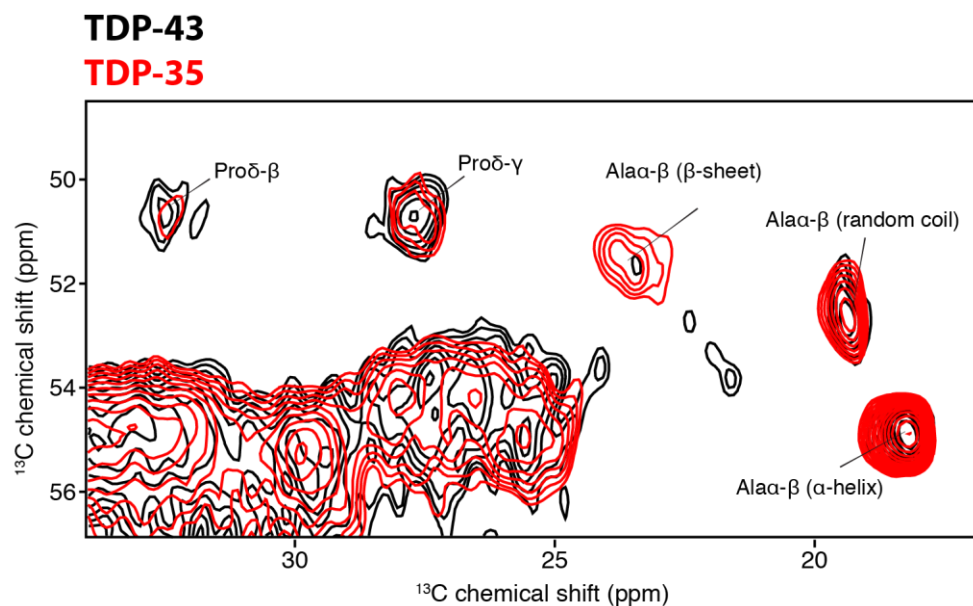
Figure 3.4 An excerpt from the overlay of the ^2\text{D} ^{13}\text{C} - ^{13}\text{C} PDS correlation spectra obtained on ( U - ^{13}\text{C} , ^{15}\text{N} )-labeled samples of full-length TDP-43 (black) and TDP-35 (red) recorded at 278 K and a ^1\text{H} frequency of 600 MHz, 11 kHz MAS frequency, a mixing time of 50 ms and 600 scans. Labels indicate characteristic alanine \text{C}\alpha - \text{C}\beta and proline \text{C}\delta - \text{C}\beta correlations and chemical shift-dependent secondary structure in brackets.
