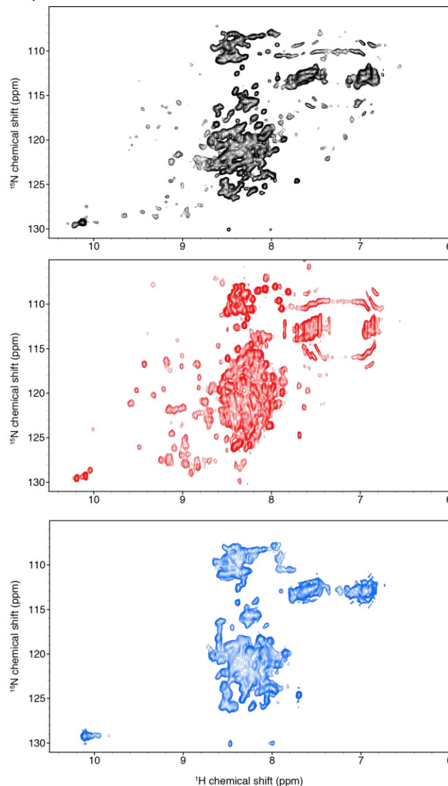
Figure 3.22 Solution NMR ^{15}\text{N} - ^1\text{H} spectra show recombinant TDP-43 (black, 36 scans) and TDP-35 (blue, 128 scans) proteins exhibiting a wide range of ^1\text{H} - ^{15}\text{N} chemical shift dispersion while TDP-16 (blue, 512 scans) with a limited ^1\text{H} - ^{15}\text{N} chemical shift dispersion. Proteins were ^{15}\text{N} labeled and prepared as described in the Materials and methods.
