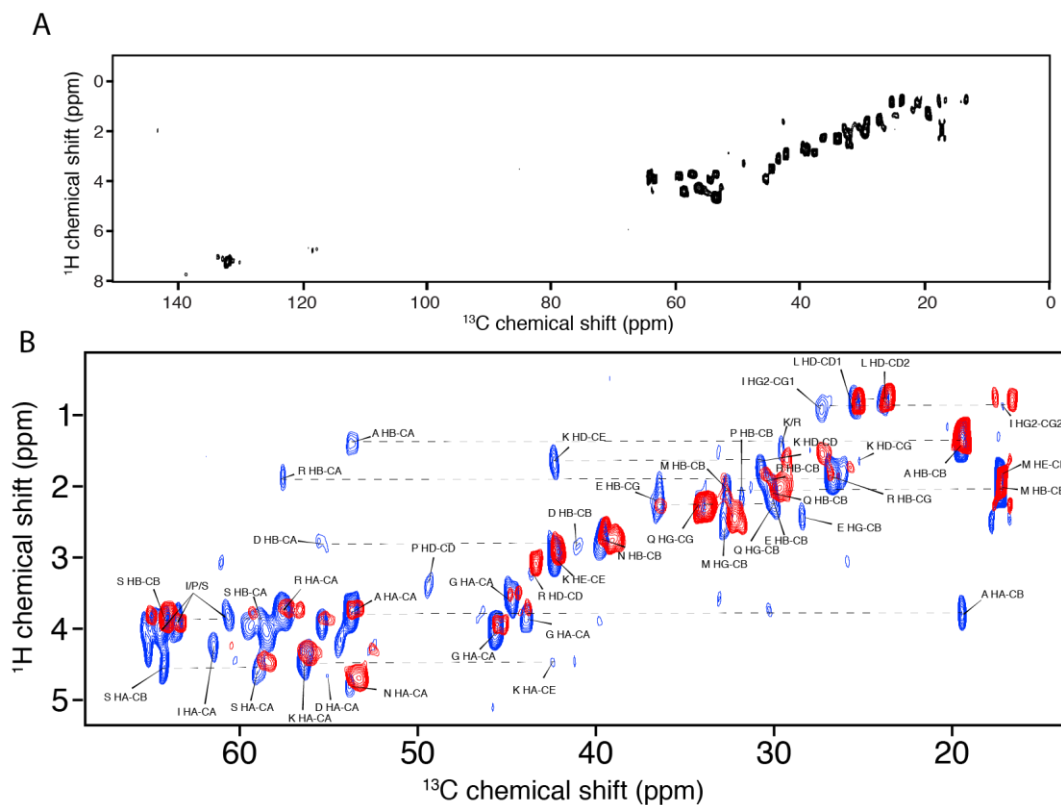
Figure 3.6 (A) ^1\text{H} - ^{13}\text{C} INEPT spectrum of TDP-35 recorded at a ^1\text{H} frequency of 600 MHz, at 278 K with 416 scans showing signals corresponding to residues in the flexible region of the fibrillar assembly. (B) SSNMR ( ^1\text{H} )- ^1\text{H} - ^{13}\text{C} INEPT-TOBSY (in blue, 2048 scans) and ^1\text{H} - ^{13}\text{C} INEPT (in red, 128 scans) spectra of TDP-16 fibrils recorded at a ^1\text{H} frequency of 600 MHz, at 278 K showing
