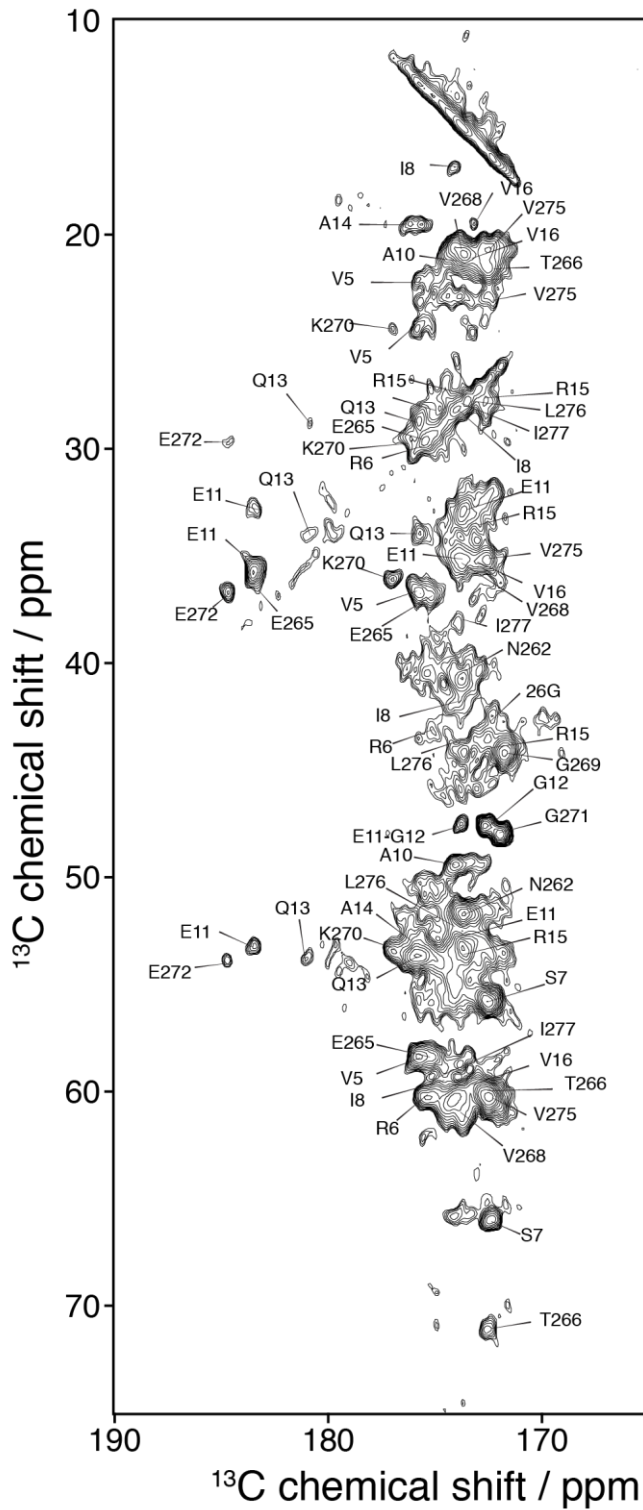
SI Figure 4.2 Solid-state NMR ^{13}\text{C} - ^{13}\text{C} correlation experiment of carbonyl region of R0-R2 fibrils recorded at a ^1\text{H} frequency of 600 MHz, 11 kHz MAS, with a PDSM mixing time of 50 ms at 278K.
