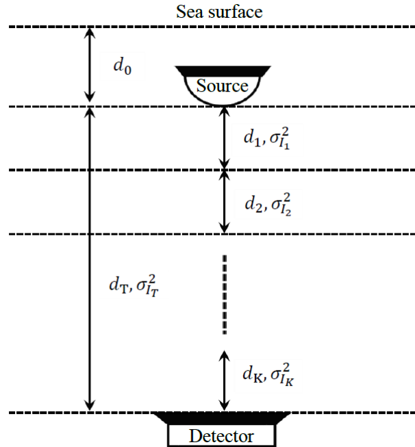
Figure 4.3: An inhomogeneous vertical underwater link subject to turbulence (reproduced from [20]).
