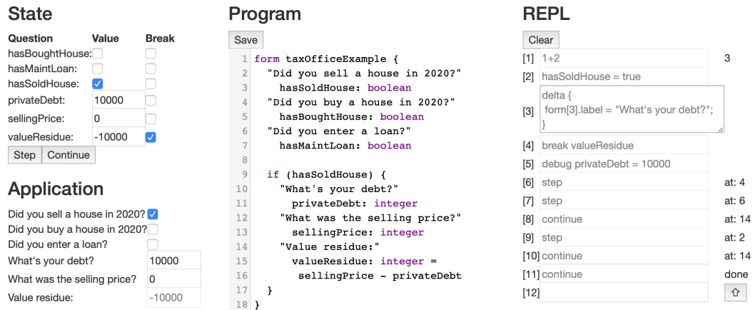
Figure 6.6 – Prototype IDE for QL: run-time view (left), source code (center), REPL (right)
