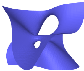
Figure 1.1: The semi-algebraic set defined by the polynomial system
