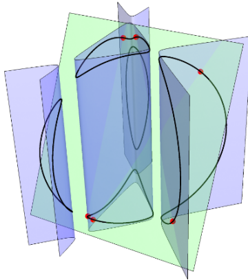
Figure 7.1: A real space curve of degree 6 with a totally real hyperplane section.
