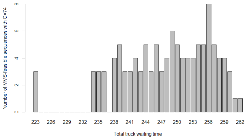
Figure 5.10 – Distribution of MMS-feasible sequences reaching C = 74 painting system purges for each value of achievable total truck waiting time
