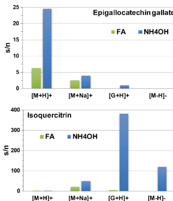
Fig. 4 Comparison of signal-to-noise ( s/n ) measured on the DEA column with the gradient method in Table 2a and mobile phase co-solvent containing 0.1% MSA. Make-up fluid contains either formic acid (FA, in green) or ammonium hydroxide and water ( NH_4OH , in blue)
