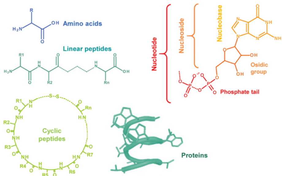
Fig. 1. Generic and representative structures of the target molecules reported in the literature reviewed in this paper.
