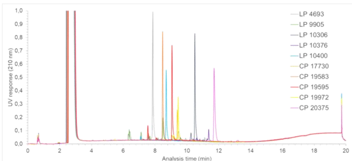
(b) Accucore HILIC with TFA
