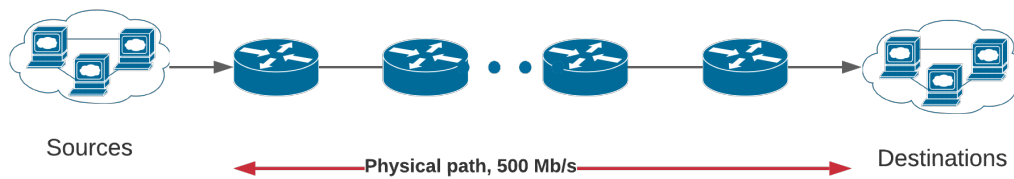
Figure 4.5: Network topology
