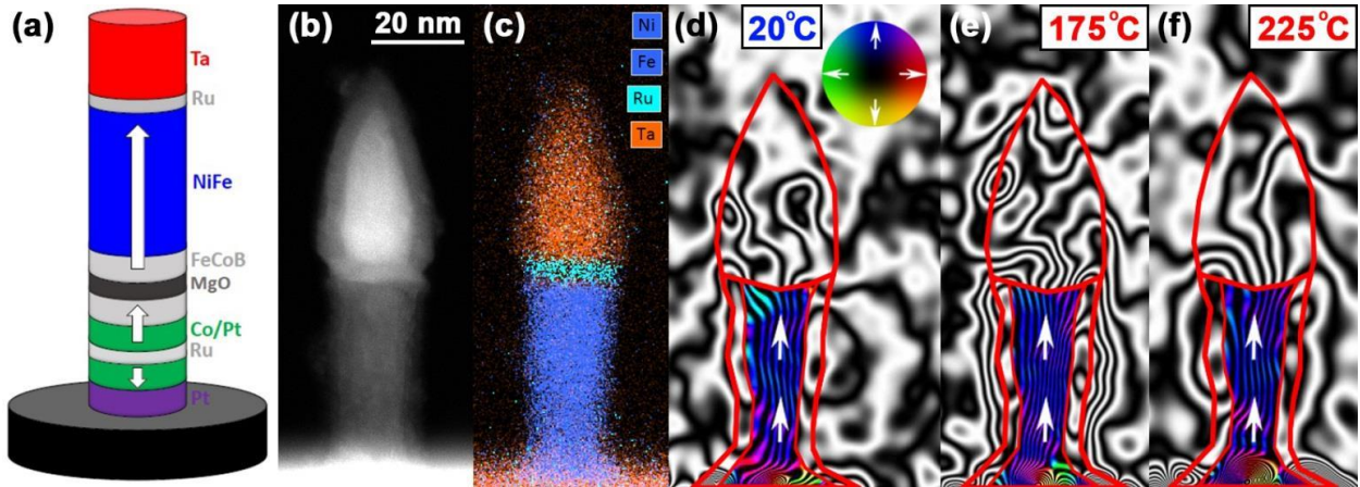
Fig. 4.2: Schematic of a PSA-STT-MRAM MTJ cell with a 60 nm thick NiFe free layer (a). STEM image of a PSA pillar with a diameter of \sim 20 nm (b); and the associated EDX chemical map showing the elemental distribution of Ta (hard mask-red), NiFe (storage layer-blue), and Ru (RIE etch stop layer-turquoise) (c). Magnetic induction maps reconstructed from electron holograms acquired during in-situ heating at (d) 20°C; (e) 175°C; and (f) 225°C. The magnetization direction is shown using white arrows, as depicted in the color wheel. From [184].
