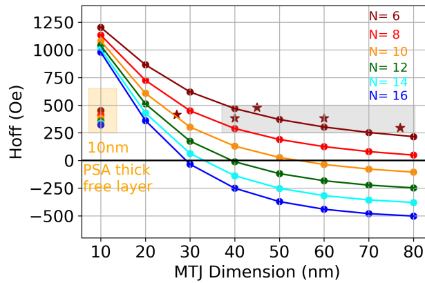
Fig. 5.17: Simulated stray field of Co/Ni SAF into the free magnetic layer of an MTJ as a function of the number of repeats comprising the bottom SAF structure: N \times ([\text{Co} \ 0.18/\text{Ni} \ 0.55])/\text{Co} \ 0.5/\text{Ru} \ 0.9 / \text{Co} \ 0.5/3 \times ([\text{Co} \ 0.18/\text{Ni} \ 0.55]) / \text{Ta} \ 0.3 / \text{FeCoB} \ 1.2/\text{MgO} \ 1.2/\text{FeCoB} \ 1.5 (thickness in nm). Experimental data corresponding to Figure 5.16 a is represented by a dark red star symbol.
