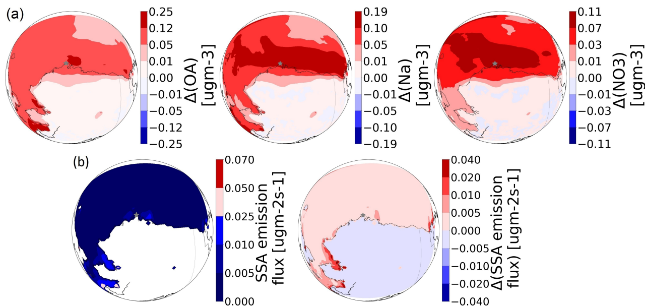
Figure 4.9: Average differences in mass concentrations of (a) sub- micron \text{Na}^+ , \text{OA} , \text{NO}_3^- , in \mu\text{g m}^{-3} , at the surface between \text{SSA\_WS\_DEP\_FEB} and \text{LOC\_ORG\_FEB} . Grey star indicates the location of Utqiagvik. (b) The map on the left shows the average value of SSA emission fluxes in \mu\text{g m}^{-2} \text{s}^{-1} during February campaign and the map on the right shows average differences between \text{SSA\_WS\_DEP\_FEB} and \text{LOC\_ORG\_FEB} in \mu\text{g m}^{-2} \text{s}^{-1} .
