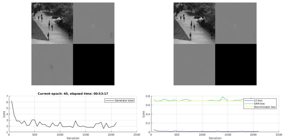
FIGURE A.6 – Illustration of training CGAN-2 on Ped1 dataset. We achieve good loss convergences at E = 40 , M = 128 and A = eLU .
