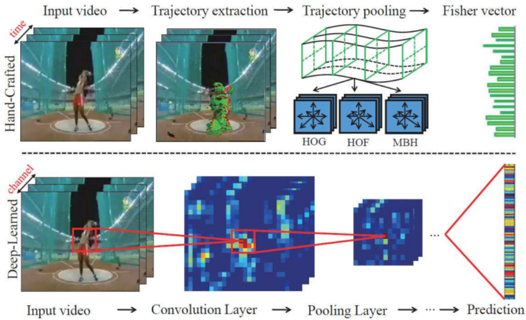
FIGURE 2.3 – Two types of features in action recognitions : Hand-crafted and Deep features [108].
