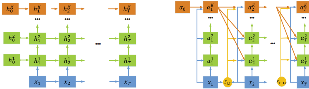
FIGURE 2.14 – Stack RCNN framework for anomaly detection proposed by Luo et al. [63]. The blue boxes represent the input of stacked RNNs. The green and orange boxes represent coding vectors. The yellow circles are similarities between neighbouring frames.
