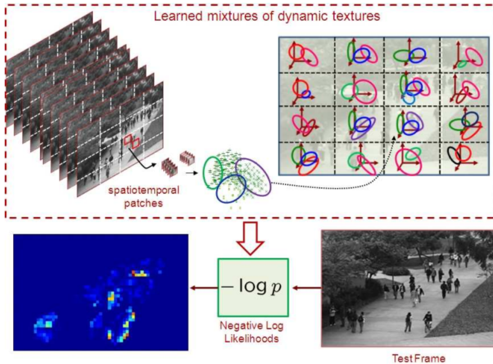
FIGURE 2.11 – Learning MDTs for temporal abnormality detection by Mahadevan et al. [66].
