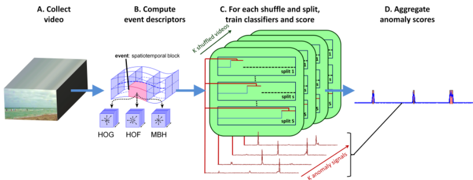
FIGURE 2.12 – Discriminative framework combining HOG, HOF, MBH for anomaly detection proposed by Giorno et al. [22].
