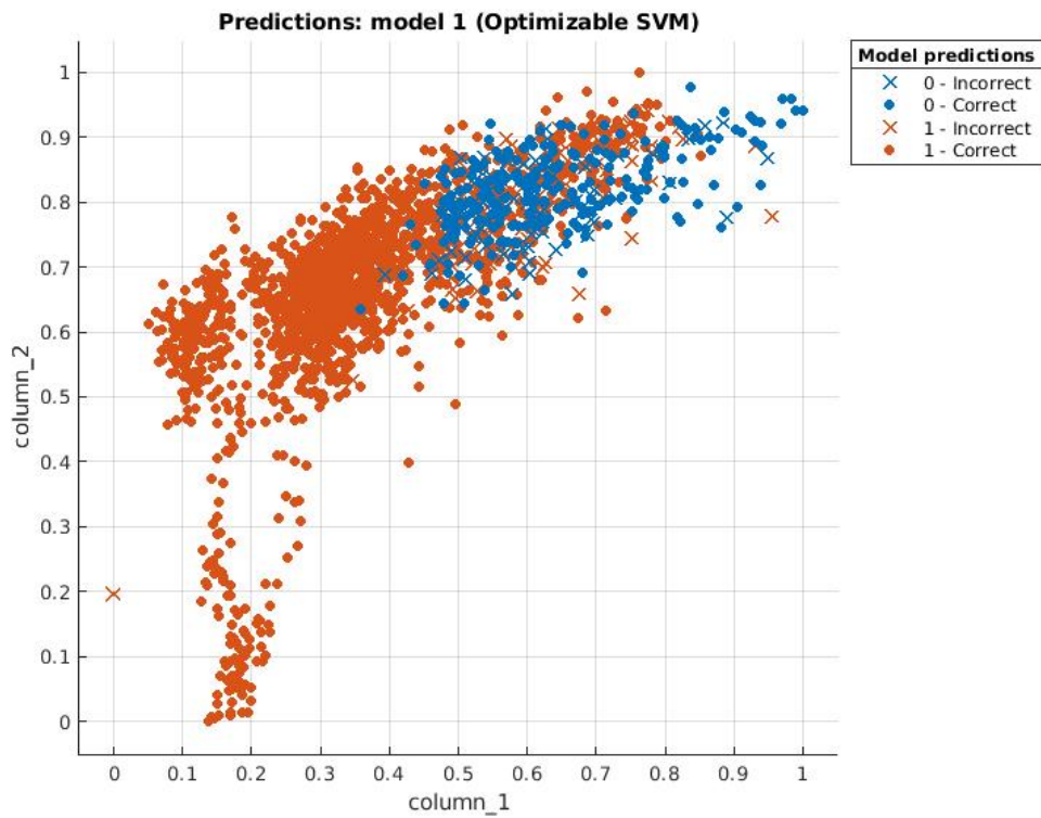
FIGURE 4.32 – Illustration of sample distribution achieved with optimized SVM model on ped2 dataset. Almost all of the normal samples situate in higher values than abnormal ones. This distribution corresponds to the fact that PSNR techniques produce high scores if predicted images tend to similar source images.
