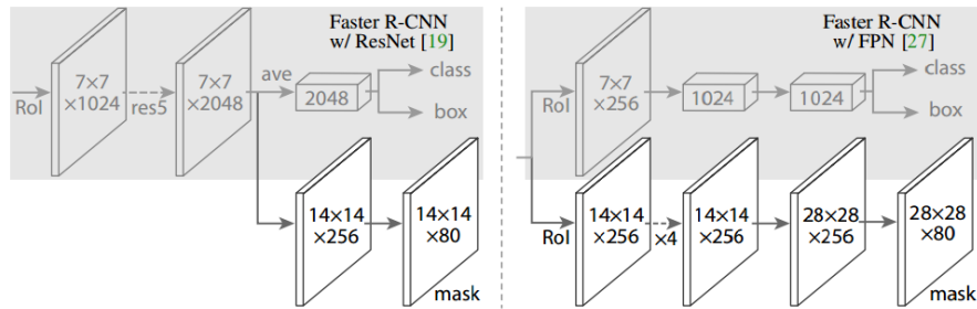
FIGURE 2.9 – Network architecture of Mask R-CNN based on very deep ResNet [29].
