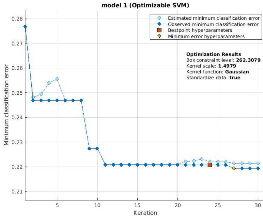
FIGURE 4.21 – Illustration of optimization process when we train SVM binary classifier on Ped1 dataset. The minimum classification error is sharply decreased after 11 iterations then becomes stable. We achieve optimized parameters at box constraint level 262.3 with Gaussian kernel.
