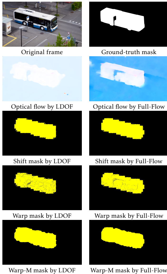
FIGURE 3.12 – Qualitative performance of generating object segmentation for bus class along forward direction. Optical flow is estimated by Full flow and LDOF. Warp-M denotes the Warp translation with Morphological operator. Despite the obvious out-performance of Full Flow over LDOF in optical flow estimation, the performance of generating new segmentation is almost stable. We draw that the performance of generating new segmentation depends on how we use the flow vector, not the type of flow. On the other hands, the importance of morphological operators integrating in Warp translation is confirmed by filling in all holes in Wrap mask.
