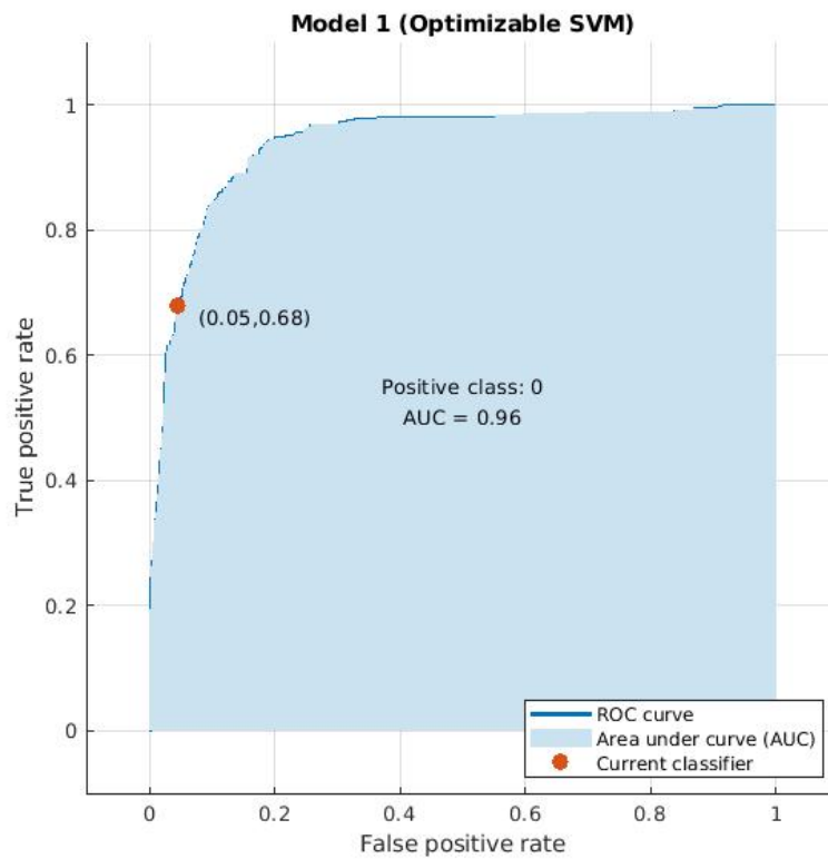
FIGURE 4.30 – Illustration of optimization performance achieved with optimized SVM model on ped2 dataset. The ROC is rapidly asymptotic to 1 while False positive rate is still very small. It means that our model achieves good performance.
