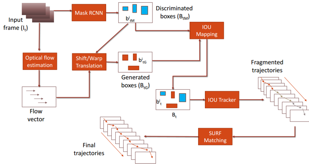
FIGURE 3.8 – Improving IOU-Tracker with generated information and SURF features. To combine the two sets : generated set B_{tG} and Mask R-CNN instances set B_{tM} , we compare the overlapping region with a threshold \sigma_{IOU} . After this step, we have only one set B_t containing the box b_t^i of frame I_t . Then Each box b_t^i is compared with all boxes of L previous frames. If we find two boxes associated to two different classes but with their IOU value and the number of matching SURF points greater than threshold \sigma_{IOU} and \sigma_{SURF} , respectively, we associate them together.
