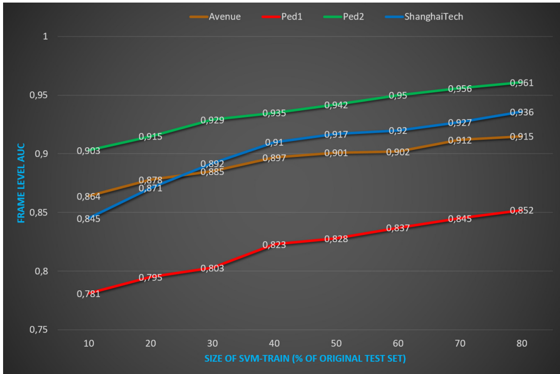
FIGURE 4.19 – Evolution of AUC performance according to the size of the SVM-train set. The vertical axis shows the AUC performances and the horizontal axis shows the size of the SVM-train set corresponding to how many samples of original test set are taken. By sequentially increasing the SVM-train set size from 10% of the original test set size up to 80%, we report the evolution of performance. Obviously, the larger the size of the SVM-train set we create, the better performance we obtain. Considering the effect of the supervised scenario, we show that from 50% of the original test set size, we surpass state-of-the-art performance on Avenue, Ped1 and ShanghaiTech. Best viewed in color.
