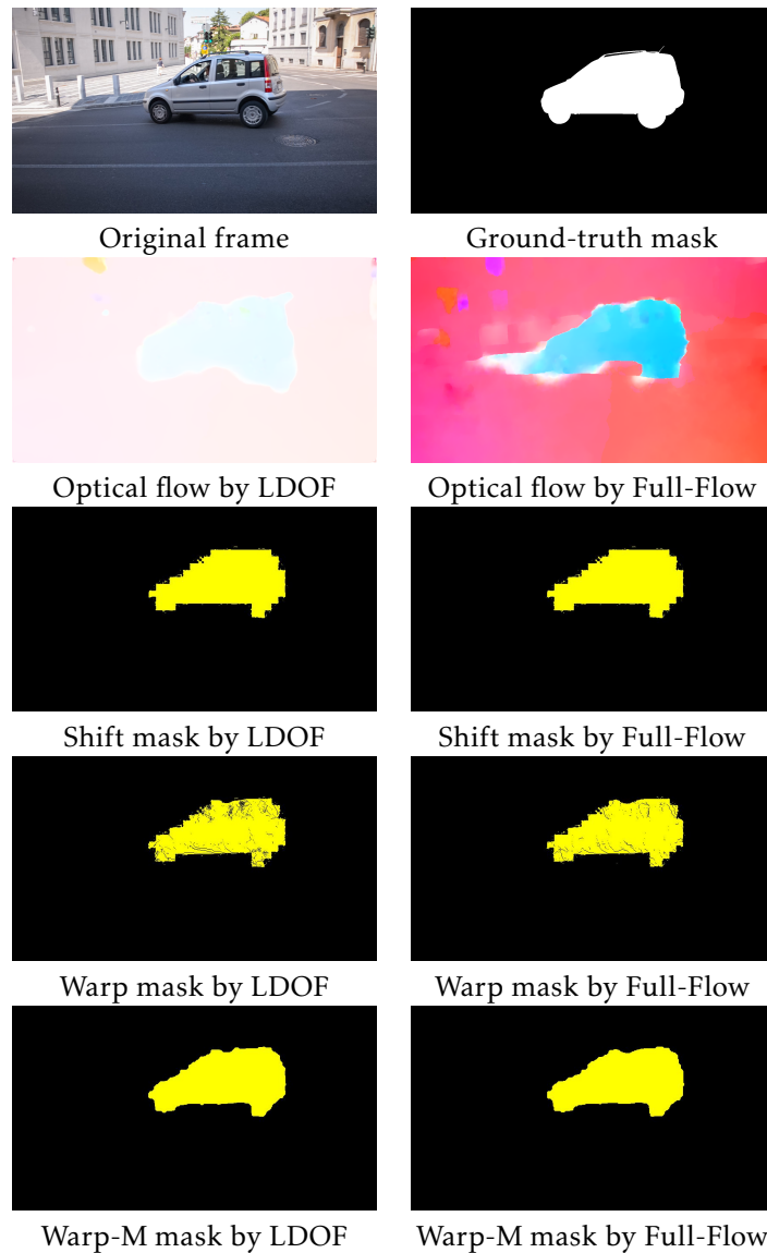
FIGURE 3.13 – Qualitative performance of generating object segmentation for car class along forward direction. Optical flow is estimated by Full flow and LDOF. Warp-M denotes the Warp translation with Morphological operator. Despite the obvious out-performance of Full Flow over LDOF in optical flow estimation, the performance of generating new segmentation is almost stable. We draw that the performance of generating new segmentation depends on how we use the flow vector, not the type of flow. On the other hands, the importance of morphological operators integrating in Warp translation is confirmed by filling in all holes in Wrap mask.
