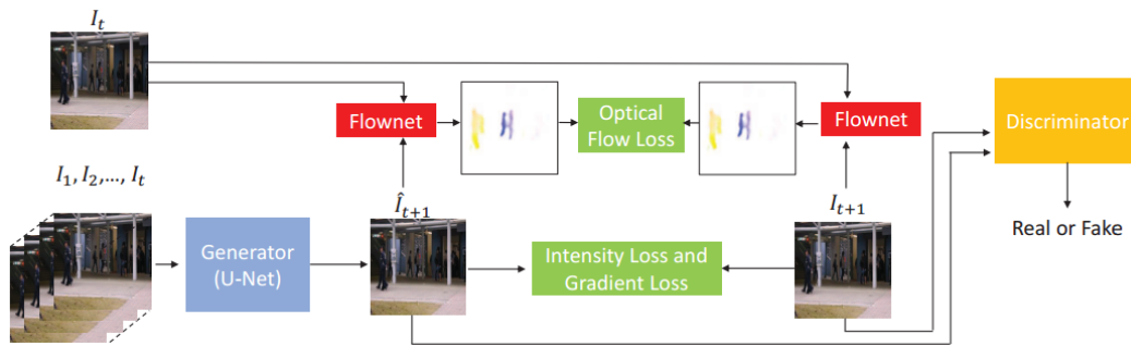
FIGURE 2.16 – Anomaly detection based on future frame prediction proposed by Liu et al. [53].
