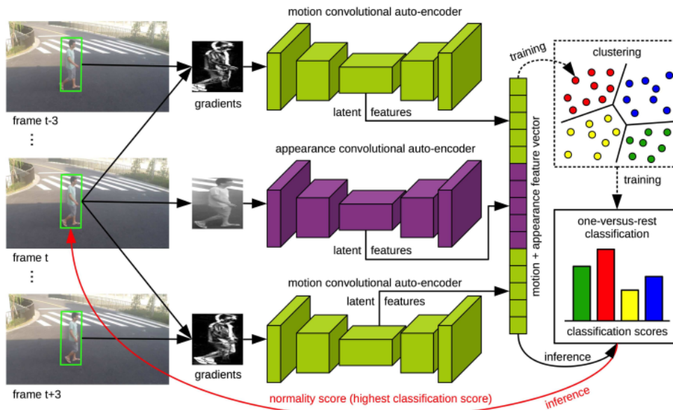
FIGURE 2.17 – Object-centric framework for anomaly detection proposed by Ionescu et al. [36].
