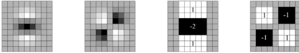
FIGURE 3.6 – Basic of Laplacian of Gaussian with Box Filter in SURF detector with Hessian matrix [5]. Left to right : The (discretized and cropped) Gaussian second order partial derivatives in y-direction and xy-direction, and approximations thereof using box filters. The grey regions are equal to zero.
