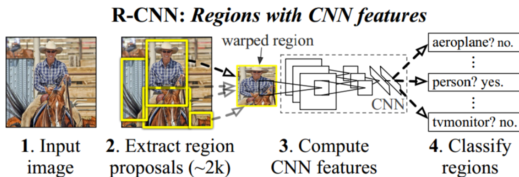
FIGURE 2.4 – The pipeline of R-CNN [24]. This is the first successful deep learning model for object detection.
