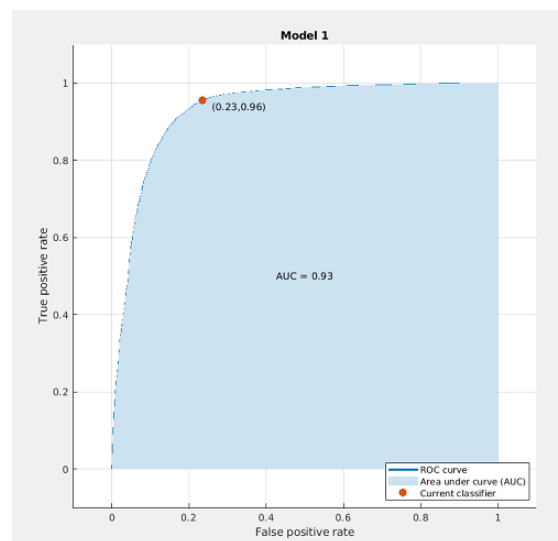
FIGURE 4.18 – An illustration of AUC-ROC. This performance belong to a good model based on AUC metric. The ROC curve is rapidly asymptotic to 1 while FPR is still small.
