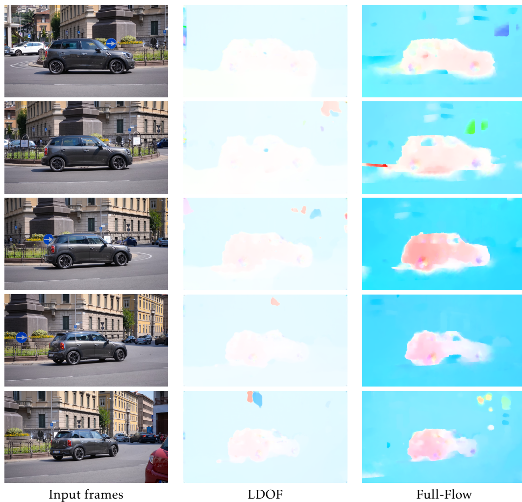
FIGURE 3.11 – Comparison of optical flow estimation performance between LDOF and Full-Flow. Results are reported on car class of DAVIS dataset. Obviously, the difference of quality between two methods is significant, not only for flow localization but also flow intensity and direction. Best viewed in color
