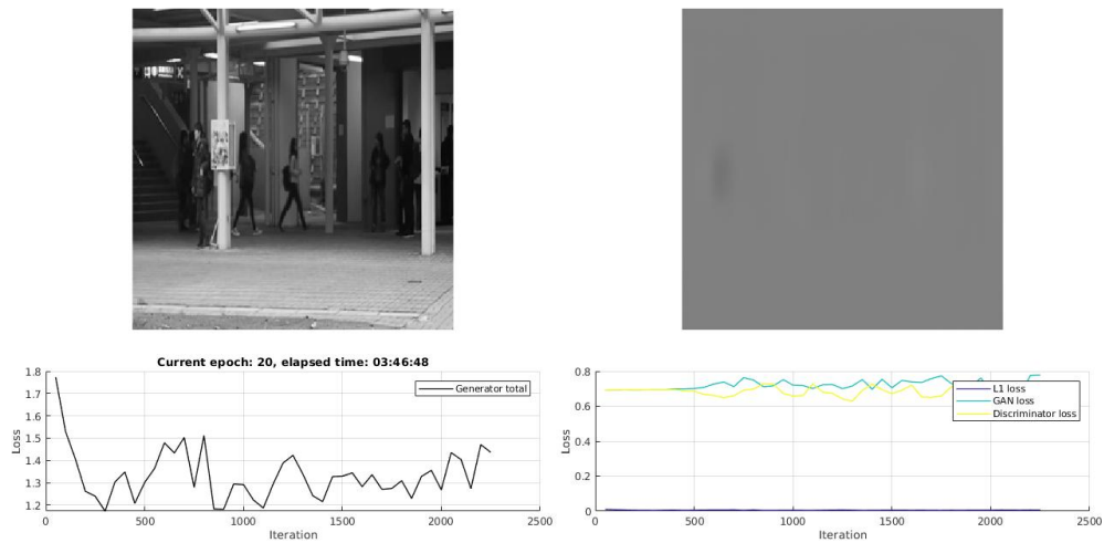
FIGURE 4.7 – Illustration of training CGAN-1 on Avenue dataset. We achieve good loss convergences for epoch E = 20 , mini batch size M = 128 and activation function A = eLU . The total loss gets rapidly small and each loss is convergent from early iterations.
