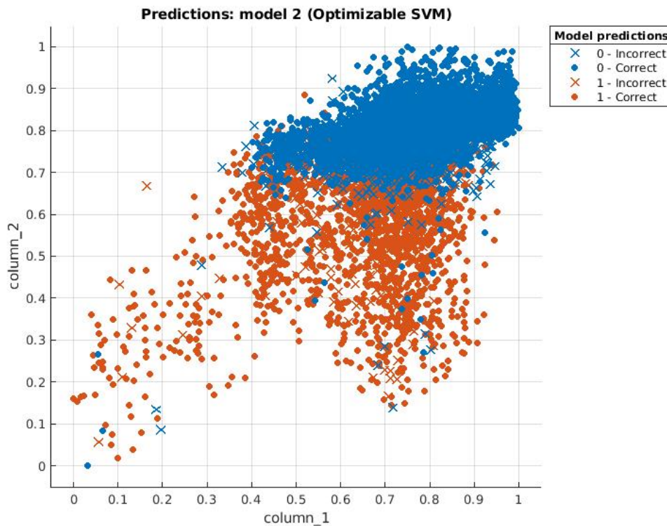
FIGURE 4.26 – Illustration of sample distribution achieved at optimized SVM model on Avenue dataset. Almost all of the normal samples situate in higher values than abnormal ones. This distribution corresponds to the fact that PSNR techniques produce high scores if predicted images tend to be similar to the source images.
