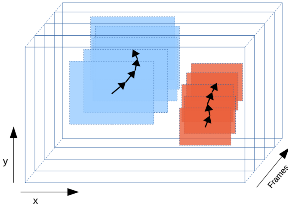
FIGURE 2.10 – IOU Tracker principle : Associating detections by their spatial overlap between time steps based on high accuracy detections at high frame rates [7].
