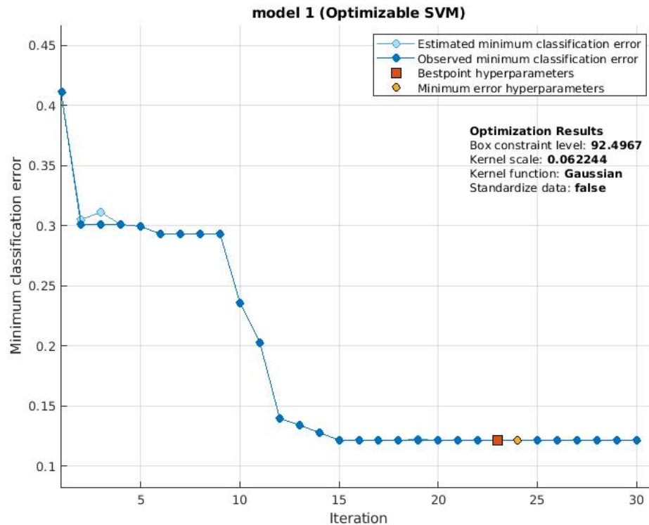
FIGURE 4.23 – Illustration of optimization process when we train SVM binary classifier on ShanghaiTech dataset. The minimum classification error is sharply decreased after 15 iterations then becomes stable. We achieve optimized parameters at box constraint level 92.50 with the Gaussian kernel.
