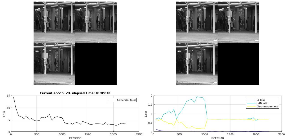
FIGURE 4.9 – Illustration of training CGAN-3 on Avenue dataset. We achieve good loss convergences at E = 20 , M = 128 and A = eLU . We find that the total loss is stable and each loss is almost convergent from the 1000^{th} iteration.
