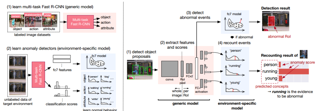
FIGURE 2.13 – Environment-dependent anomaly detectors proposed by Hinami et al. [33]. The left part illustrates learning procedures of two types of models : generic and environment-specific models, and right part shows testing procedure of joint detection and recounting abnormal events.
