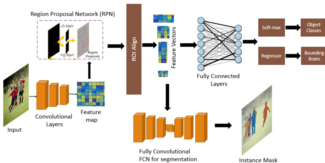
FIGURE 3.1 – General pipeline of Mask R-CNN. It contains two stages : First, it generates region proposals where there might be an object based on the input image. Second, it predicts the object classes, refines the bounding box and generates a mask at the pixel level of the object based on the first stage proposal.
