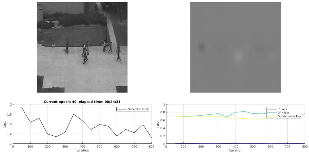
FIGURE A.9 – Illustration of training CGAN-1 on Ped2 dataset. We achieve good loss convergences at E = 40 , M = 128 and A = eLU .
