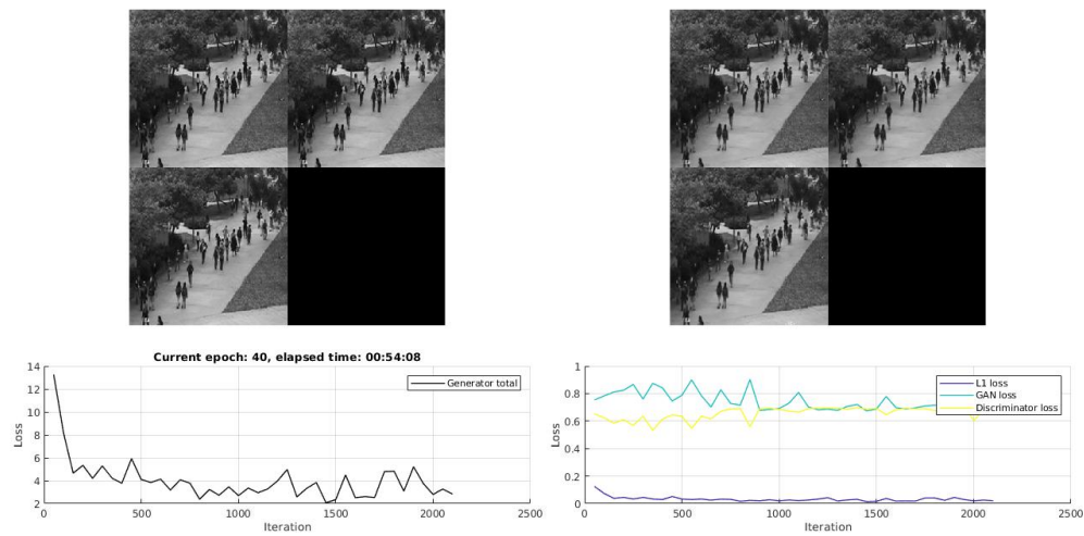
FIGURE A.7 – Illustration of training CGAN-3 on Ped1 dataset. We achieve good loss convergences at E = 40 , M = 128 and A = eLU .
