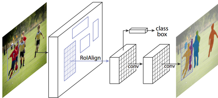
FIGURE 2.6 – The Mask R-CNN framework for instance segmentation [29].
