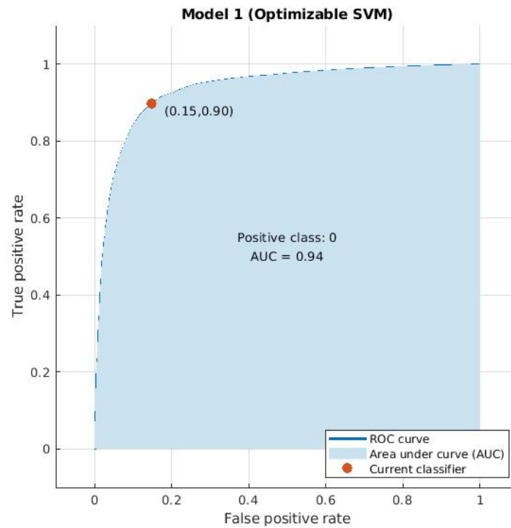
FIGURE 4.33 – Illustration of optimization performance achieved with optimized SVM model on ShanghaiTech dataset. The ROC is rapidly asymptotic to 1 while False positive rate is still very small. It means that our model achieves good performance.
