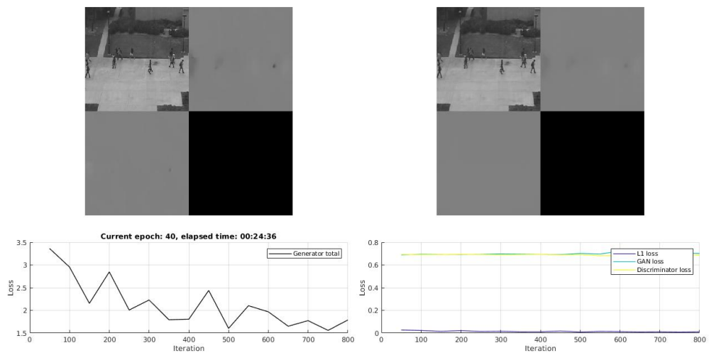
FIGURE A.10 – Illustration of training CGAN-2 on Ped2 dataset. We achieve good loss convergences at E = 40 , M = 128 and A = eLU .
