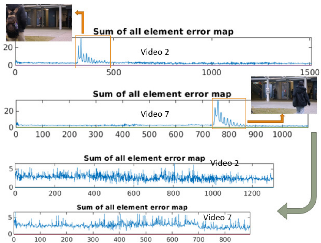
FIGURE 4.11 – Example of outliers removing on Avenue dataset. In order not to do it manually, we train CGAN-2 on training set to produce output images. Then we accumulate MSE values between output and ground-truth images for all of the 3 channels and we draw the corresponding values. We can easily observe some peaks occurring at the abnormal frames on training videos. We remove the outlier images corresponding to the peaks to obtain a new clean Avenue training set. Best viewed in color.
