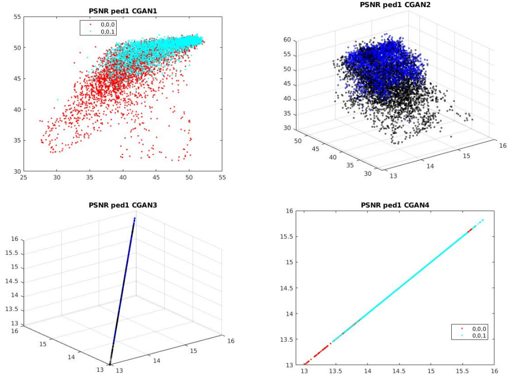
FIGURE 4.13 – Distribution of normal and abnormal samples in Ped1 dataset. The axes of each figure denote the value of PSNR before normalization. For CGAN-2 and CGAN-3, normal points are blue and abnormal points are black. For CGAN-1 and CGAN4, normal = light blue and abnormal = red.
