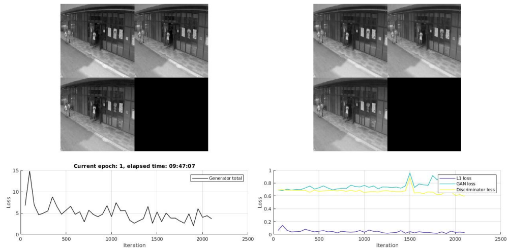
FIGURE A.15 – Illustration of training CGAN-3 on ShanghaiTech dataset. We achieve good loss convergences at E = 1 , M = 128 and A = eLU .
