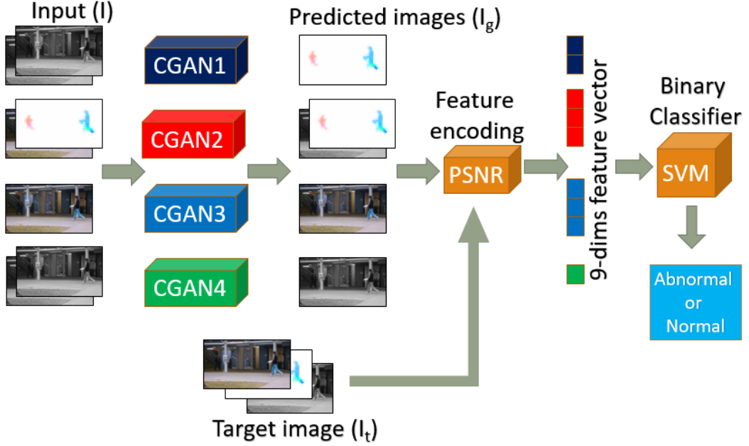
FIGURE 4.1 – Our multi-channels pix2pix-CGANs framework for anomaly detection. In each CGAN stream, the number of channels and the type of each channel for input image ( i.e. source image I ) and output image ( i.e. generated or predicted image I_g ) are different. CGAN1 takes 2 grayscale channels as input and generates 2-dimensional optical flow channels as output. CGAN2 takes 1 grayscale channel and a 2-dimensional optical flow channel as input and generates 1 grayscale channel and 2-dimensional optical flow channel as output. CGAN3 takes a 3-dimensional RGB channels as input and 3-dimensional RGB channel as output. CGAN4 takes 2-dimensional grayscale channels as input and generates 1-dimensional grayscale channel as output. The configuration is described in detail in Table 4.1. The channels of generated images are similar to the channels of ground-truth images ( i.e. target images I_t ). Best viewed in color.
