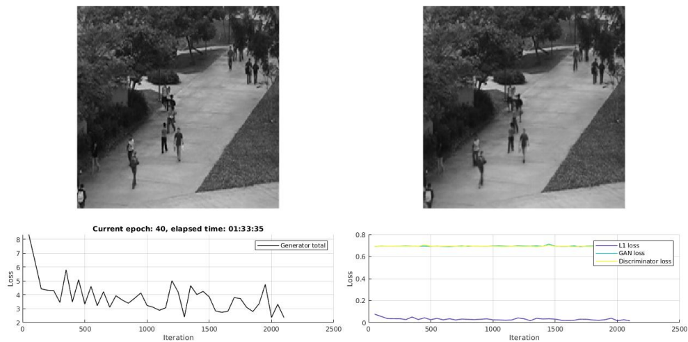
FIGURE A.8 – Illustration of training CGAN-4 on Ped1 dataset. We achieve good loss convergences at E = 40 , M = 128 and A = eLU .
