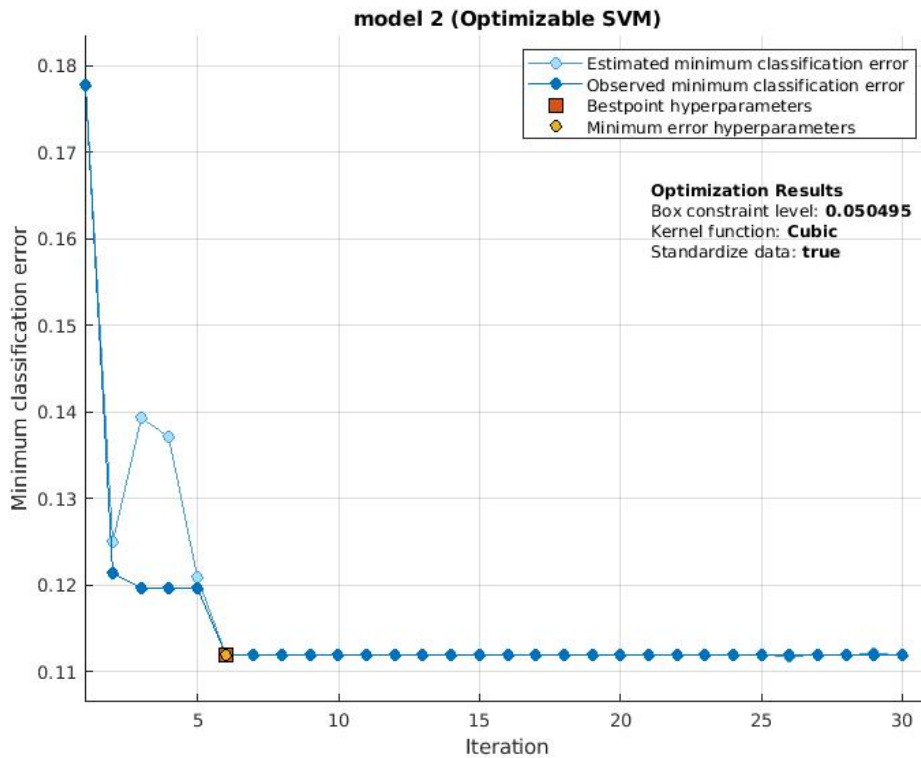
FIGURE 4.20 – Illustration of optimization process when we train SVM binary classifier on Avenue dataset. The minimum classification error is sharply decreased after 6 iterations then becomes stable. We achieve optimized parameters at box constraint level 0.05 with the cubic kernel.
