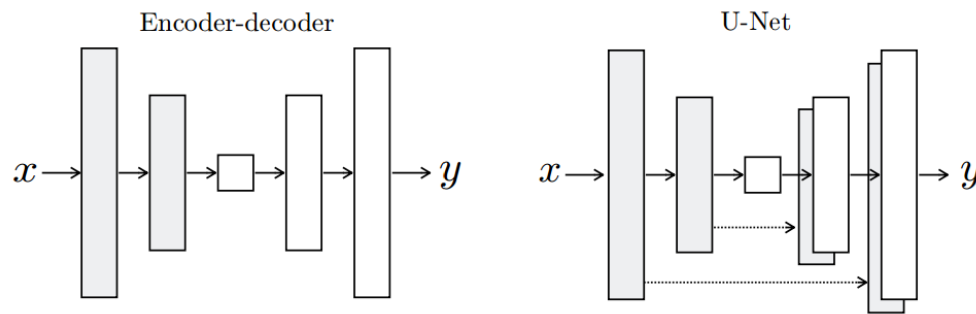
FIGURE 4.2 – Two possible network architecture of CGAN generator : Encode-Decode and U-Net with skip connection [39].
