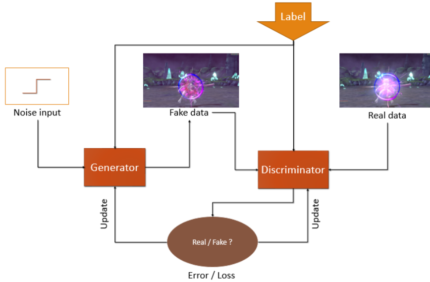
FIGURE 4.3 – Conditional-GAN principle : The generator - Given a label and random noise as input, this model generates data with the same structure as the training data observations corresponding to the same label. The discriminator - Given batches of labeled data containing observations from both the training data and the generated data from the generator, this network attempts to classify the observations as "real" or "fake".
