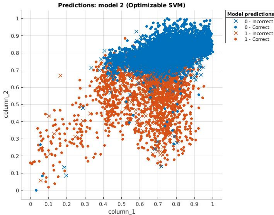
FIGURE 4.29 – Illustration of sample distribution achieved with optimized SVM model on ped1 dataset. Almost all of the normal samples situate in higher values than abnormal ones. This distribution corresponds to the fact that PSNR techniques produce high scores if predicted images tend to be similar to the source images.
