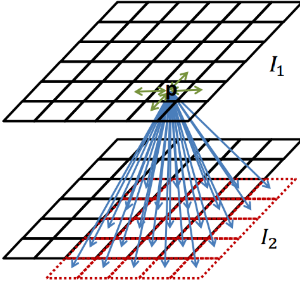
FIGURE 3.4 – Optical flow over regular grid in Full Flow method [13]. Each pixel p in I_1 is spatially connected to its four neighbors in I_1 and temporally connected to (2\zeta + 1)^2 pixels in I_2 .
