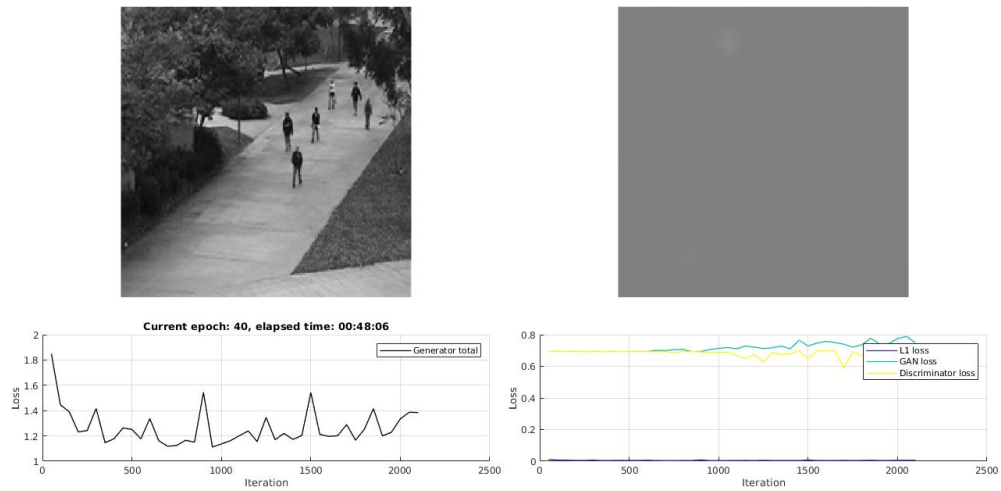
FIGURE A.5 – Illustration of training CGAN-1 on Ped1 dataset. We achieve good loss convergences at E = 40 , M = 128 and A = eLU .
