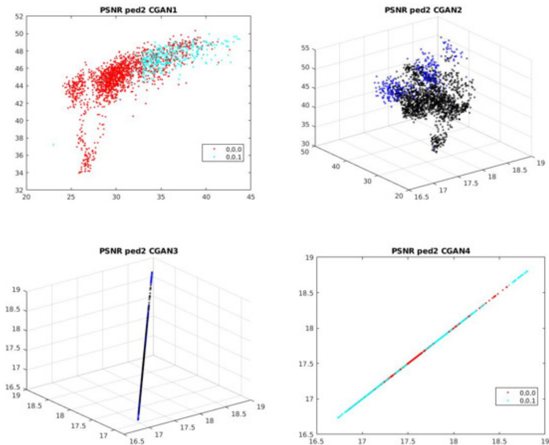
FIGURE 4.14 – Distribution of normal and abnormal samples in Ped2 dataset. The axes of each figures denote the value of PSNR before normalization. For CGAN-2 and CGAN-3, normal points are blue and abnormal points are black. For CGAN-1 and CGAN4, normal = light blue and abnormal = red.
