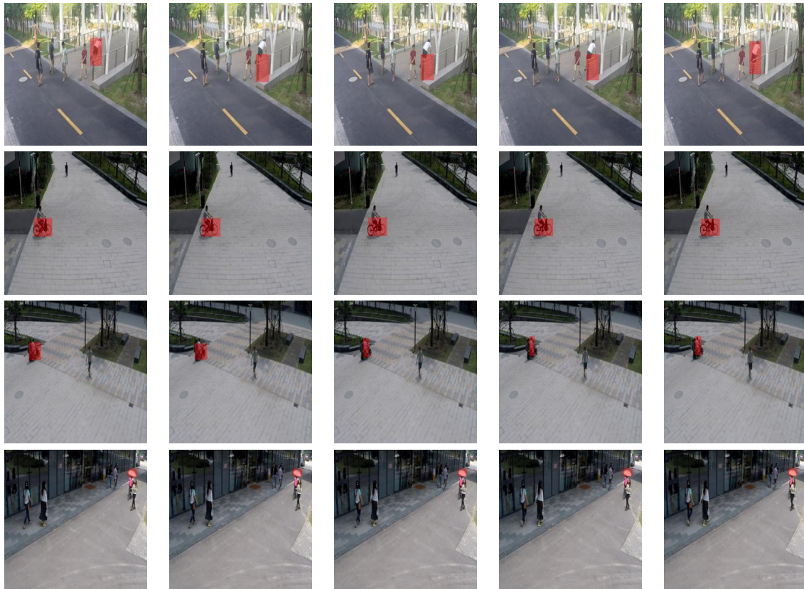
FIGURE 4.38 – Qualitative results of single abnormal object localization on ShanghaiTech dataset. There are two types of abnormality illustrated in this figure : jumping (first row) and wrong vehicles (all other rows). All abnormal objects are detected, but there are still some flaws due to the drawback of Mask R-CNN, especially in the last row. Instead of localizing all the persons with a bicycle, our algorithm chooses only the umbrella.
