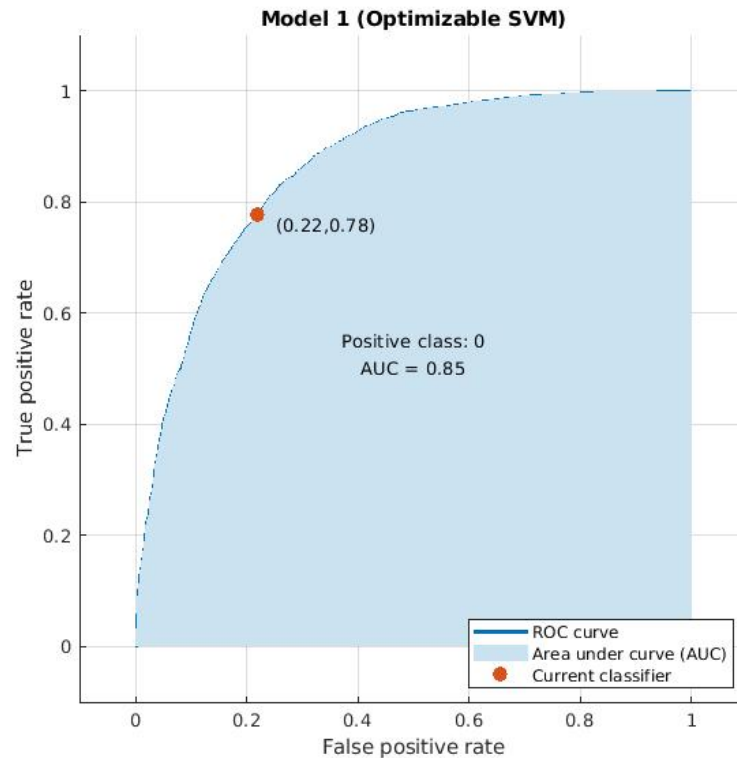
FIGURE 4.27 – Illustration of ped1 performance achieved with optimized SVM model on Avenue dataset. The ROC is rapidly asymptotic to 1 while False positive rate is still very small. It means that our model achieves good performance.
