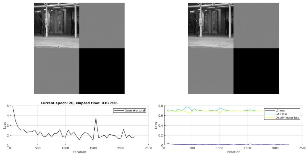
FIGURE 4.8 – Illustration of training CGAN-2 on Avenue dataset. We achieve good loss convergences at E = 20 , M = 128 and A = eLU . We find that the total loss is stable from the 1700 th iteration while each loss is almost convergent from early iterations.
