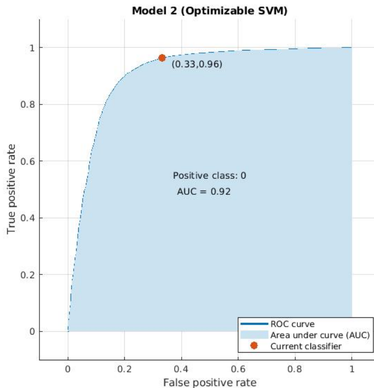
FIGURE 4.24 – Illustration of AUC performance achieved at optimized SVM model on Avenue dataset. The ROC is rapidly asymptotic to 1 while False positive rate is still very small. It means that our model achieves good performance.
