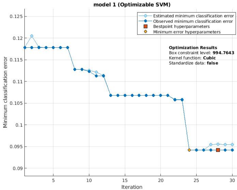
FIGURE 4.22 – Illustration of optimization process when we train SVM binary classifier on Ped2 dataset. The minimum classification error is sharply decreased after 24 iterations then becomes stable. We achieve optimized parameters at box constraint level 994.76 with the cubic kernel.
