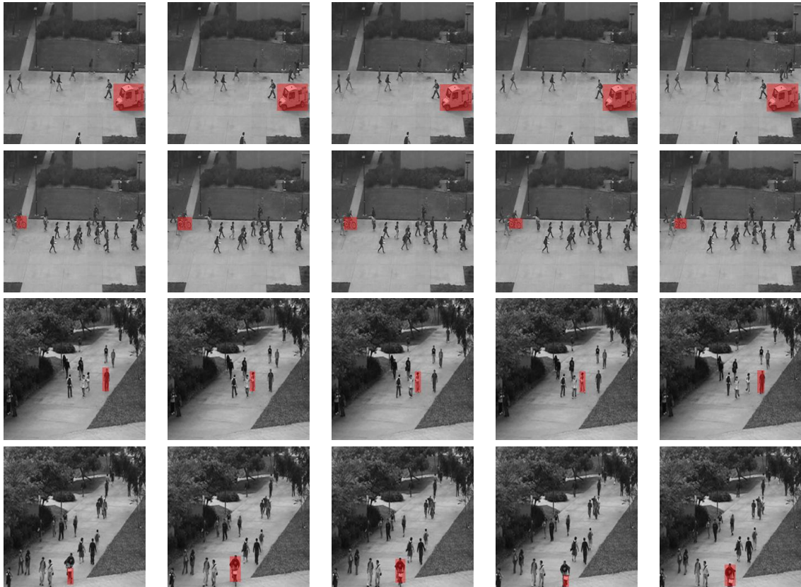
FIGURE 4.37 – Qualitative results of single abnormal object localization on Ped1 and Ped2 datasets. There are two typical types of abnormality in Pedestrian datasets : wrong vehicles (car, bicycle, etc. ) and moving to wrong direction. Generally, the abnormal vehicles are easier (to detect) than the wrong moving direction. While all abnormal vehicles are localized in the first, second and fourth row, there are some false positive errors in the third row where the abnormal persons are crossing the road. The same drawback of Mask R-CNN bounding boxes still happens as in Avenue dataset.
