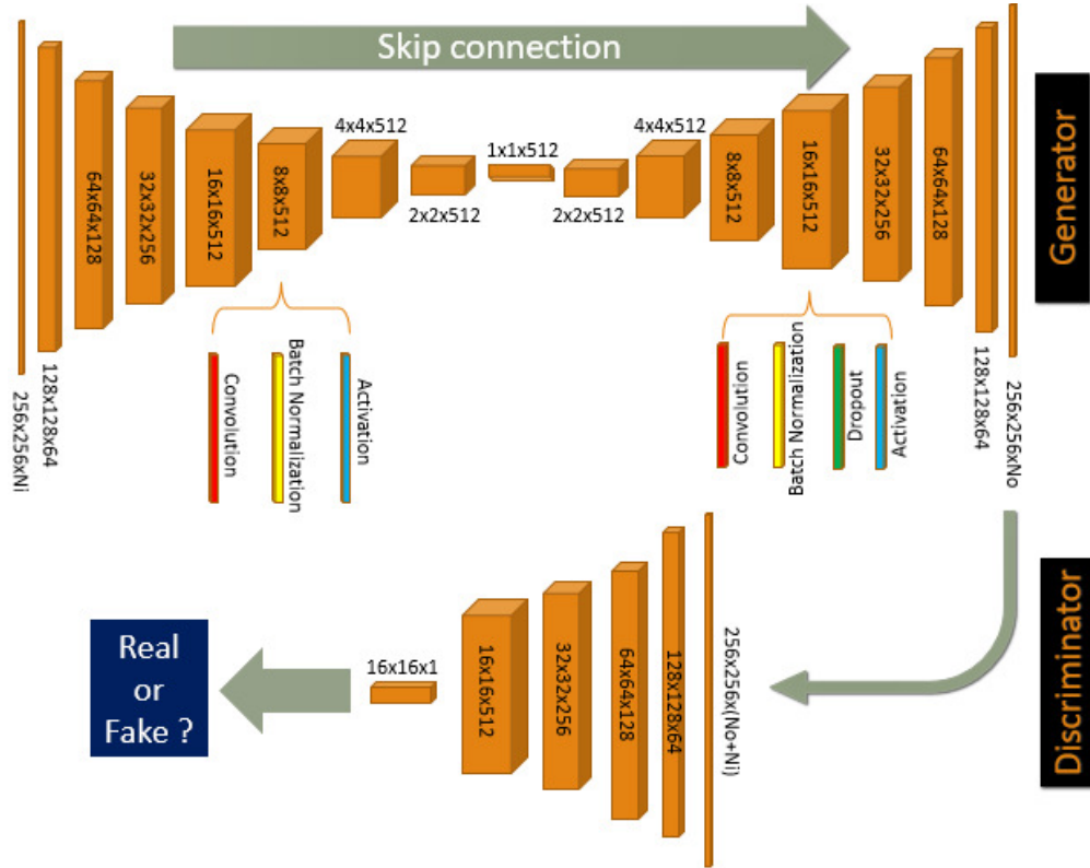
FIGURE 4.4 – Our pix2pix-CGAN architecture. Encoder blocks CE_k are from first block 256 \times 256 \times N_i to bottleneck block 1 \times 1 \times 512 of Generator. Decoder blocks CD_k are from bottleneck block 1 \times 1 \times 512 to last block 256 \times 256 \times N_o of Generator. N_i, N_o denote the number of input and output image channels of Generator. Discriminator blocks C_k are from block 256 \times 256 \times (N_i + N_o) to block 16 \times 16 \times 1 . Because of the skip connection, the total channels pass to Discriminator is N_i + N_o . Best viewed in color.
