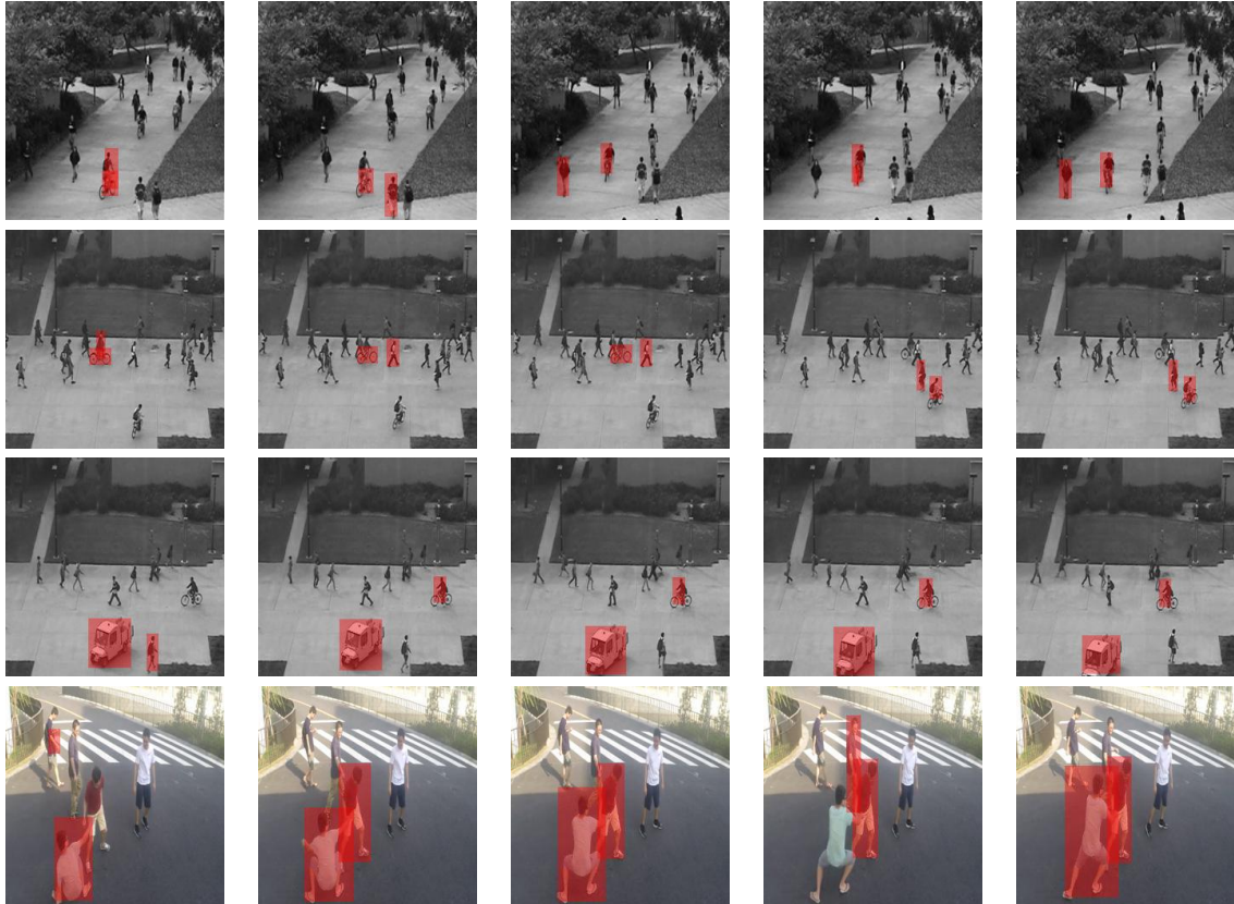
FIGURE 4.39 – Qualitative results of multiple abnormal objects localization on Pedestrian and ShanghaiTech datasets. We set the number of abnormal object to 2. While the first object ( i.e. obtaining minimum PSNR score) is almost always true, the second object ( i.e. obtaining the second minimum PSNR score) is false positive when its is near the first object. This drawback comes from the accumulated errors of the optical flow in estimating and generating steps. Besides, overlapped objects are detected by Mask R-CNN at the same location, e.g. bicycle and person in pedestrian samples. Obviously, both objects usually obtain lower PSNR score than the rest. Therefore, our algorithm chooses the two objects at the same location instead of searching for a new position.
