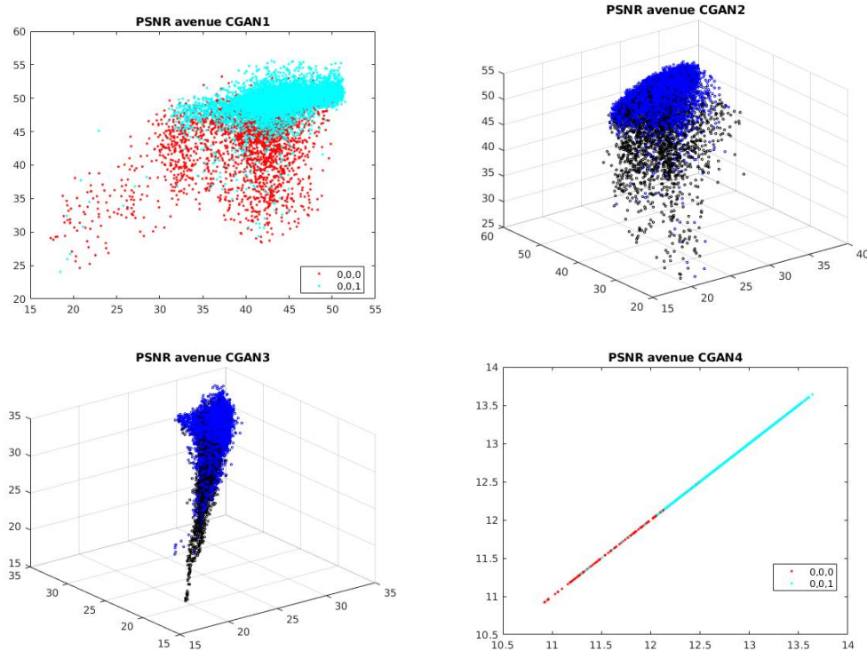
FIGURE 4.12 – Distribution of normal and abnormal samples in Avenue dataset. The axes of each figure denote the value of PSNR before normalization. For CGAN-2 and CGAN-3, normal points are blue and abnormal points are black. For CGAN-1 and CGAN4, normal = light blue and abnormal = red.
