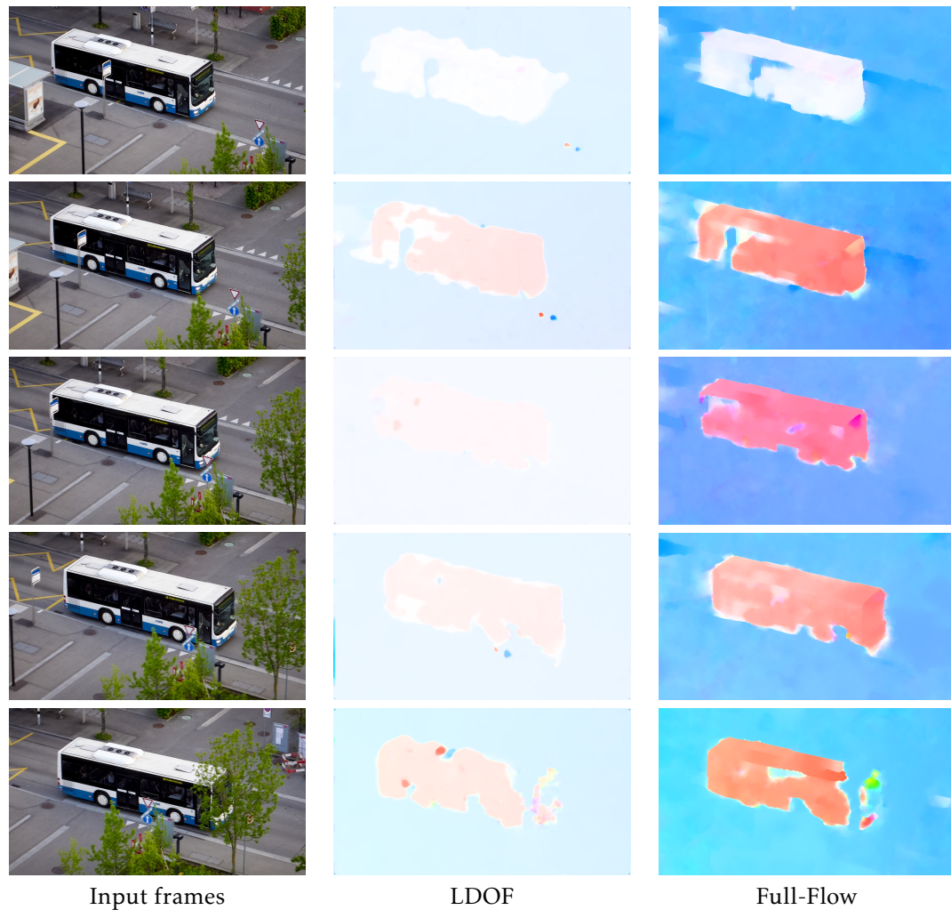
FIGURE 3.10 – Comparison of optical flow estimation performance between LDOF and Full-Flow. Results are reported on bus class of DAVIS dataset. Obviously, the difference of quality between two methods is significant, not only for flow localization but also for flow intensity and direction. Best viewed in color
