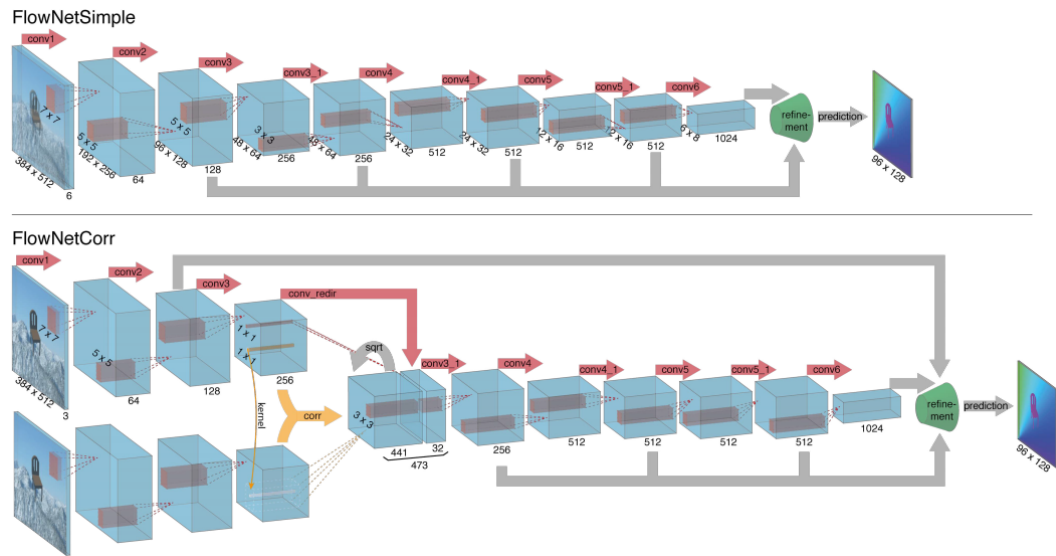
FIGURE 2.7 – Network architecture of Flow-Net [19]. This is the first successful deep learning model for optical flow estimation.
