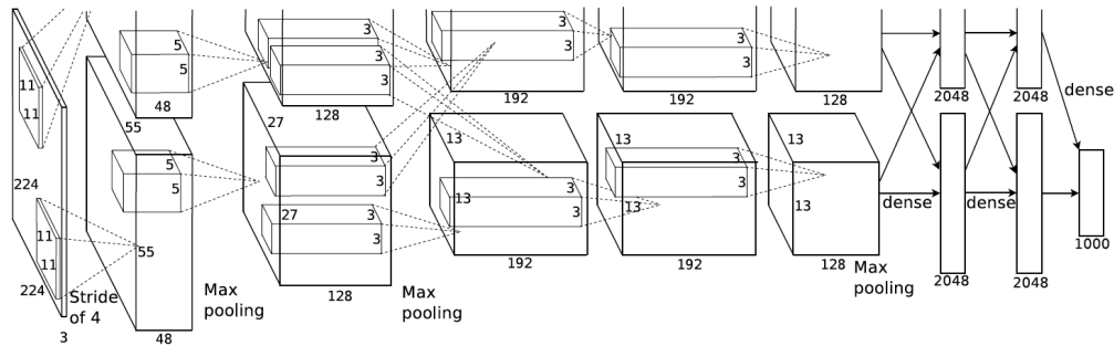
FIGURE 2.1 – AlexNet architecture [43] - The first successful CNN model with 7 layers. This architecture is a basic model for most of the recent innovative CNN architectures.
