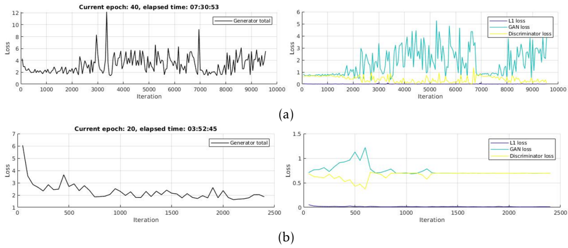
FIGURE 4.6 – Comparison of loss convergence between different parameters for CGAN-2 on Avenue dataset. Figure (a) shows the case where the loss are not convergent after 40 epochs, Minibatch size 64 and leakyReLU activation function while Figure (b) illustrates a good set of parameters E = 20, M = 128, A = eLU corresponding to a good loss convergence. We find that the total loss is stable from the 1000 th iteration and each loss is almost convergent. Best viewed in color.
