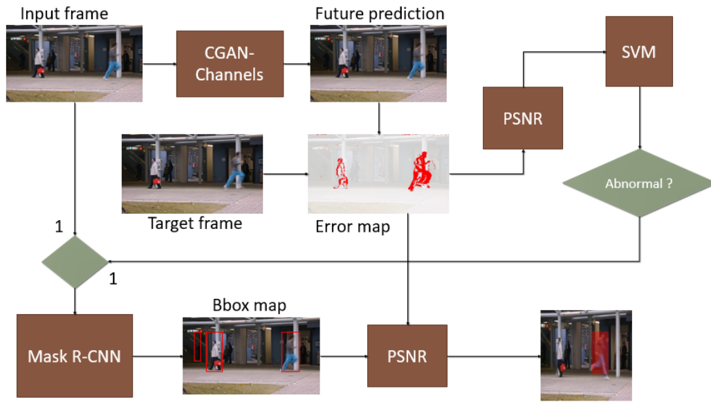
FIGURE 4.17 – The pipeline of abnormality object localisation framework. After the frame-level anomaly detection stage, we obtain the labels for each frame. For each abnormal frame, we run a fast detector to compute bounding boxes (BB) for each object in the sequence and we directly apply each BB to the error maps. PSNR scores are computed for each one by taking the normal sum of 9 PSNR scores and BBs yielding minimum values for PSNR scores refer to the abnormality objects.
