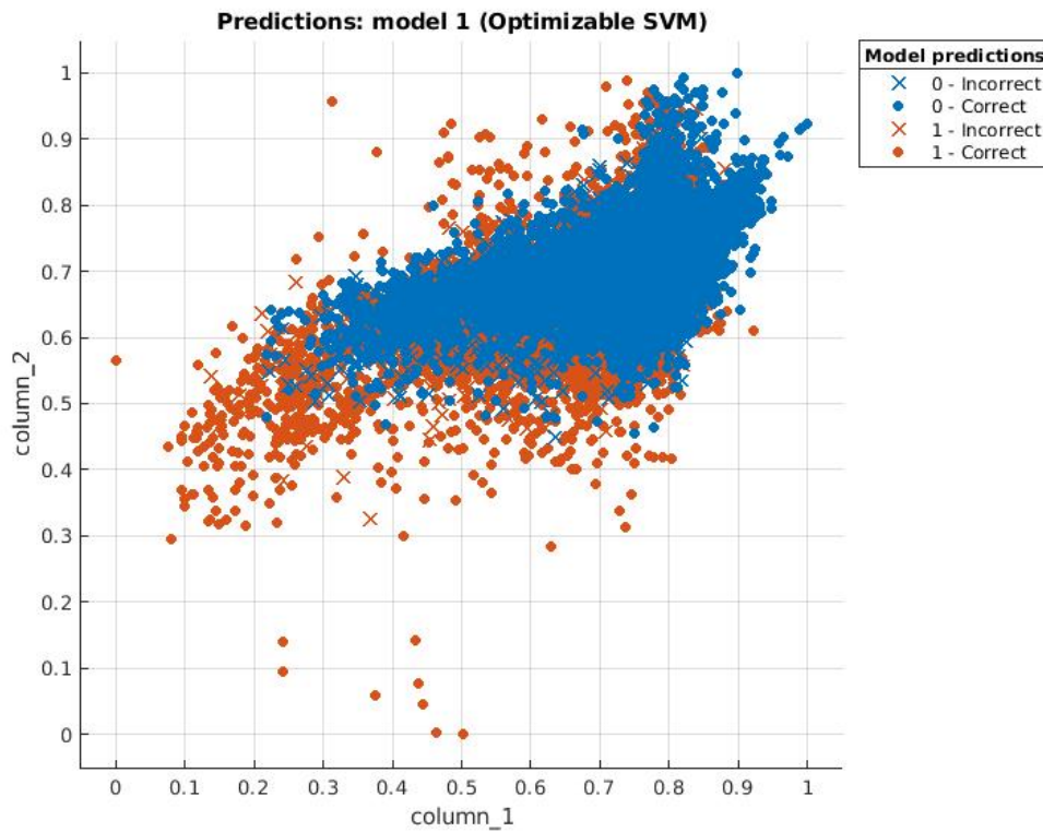
FIGURE 4.35 – Illustration of sample distribution achieved with optimized SVM model on ShanghaiTech dataset. Almost all of the normal samples situate in higher values than abnormal ones. This distribution corresponds to the fact that PSNR techniques produce high scores if predicted images tend to be similar to the source images.
