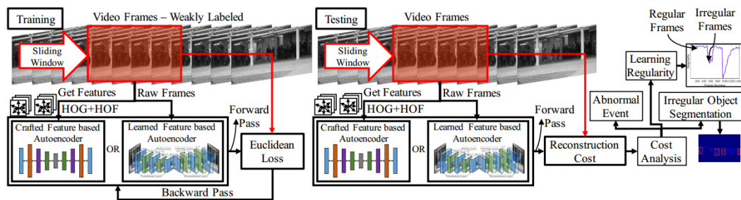
FIGURE 2.15 – Generative framework combining motion features or learned features with autoencoder to reconstruct the scene for anomaly detection proposed by Hasan et al. [27].
