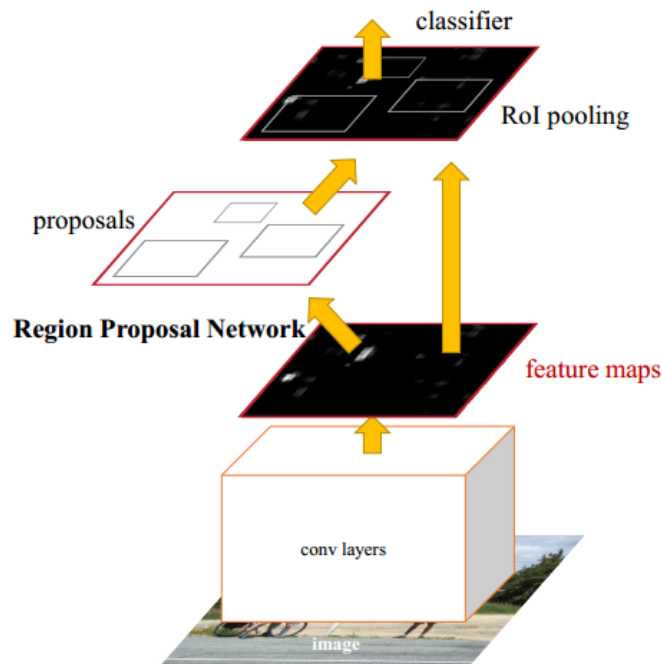
FIGURE 2.5 – Network architecture of Faster R-CNN [85]. RPN is a key module to construct an unified end-to-end model for object detection.
