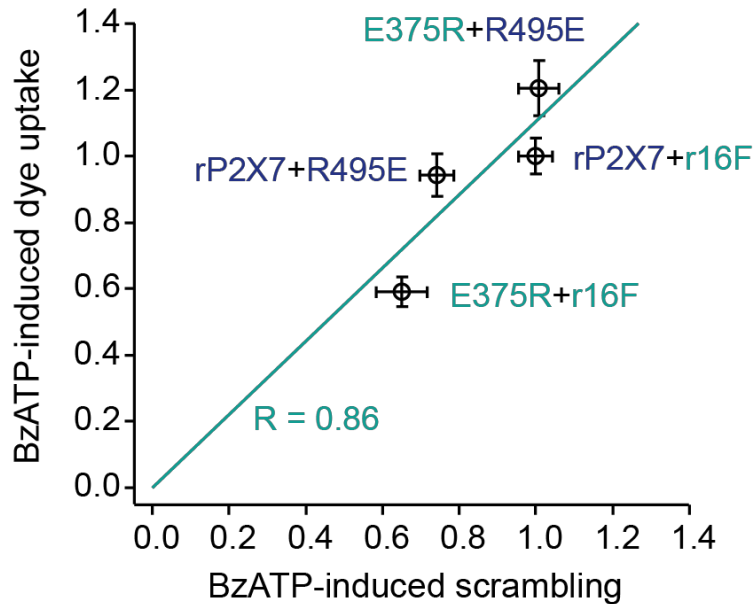
Figure 4.11: Correlation between pore formation and scramblase activity.
