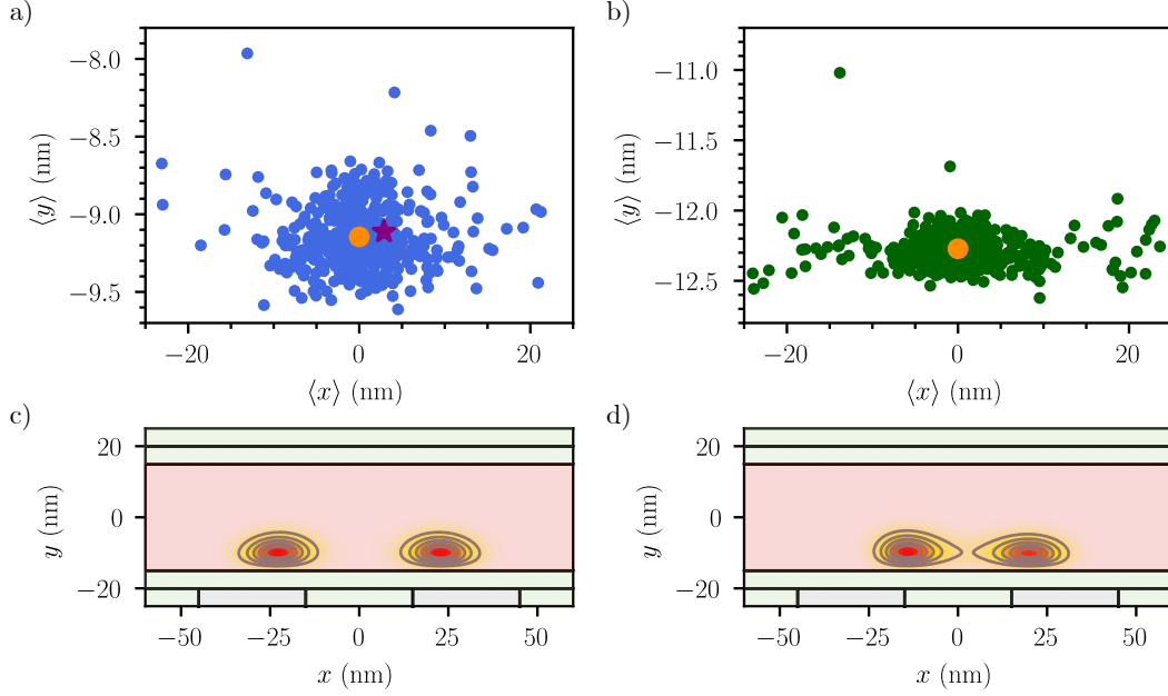
Figure 5.11: Variability in the double QD position. a) Average position in the (xy) plane of the double QD system for electrons. Orange point denotes the ideal device, whereas purple star shows the device whose ground state wavefunction is plotted in d). b) Average position in the (xy) plane of the double QD system for holes. Orange point denotes the ideal device. c) Cross-section of the ground state wavefunction for the electrons' pristine device. d) Cross-section of the ground state wavefunction for a particular realization of disorder in an electron device.
