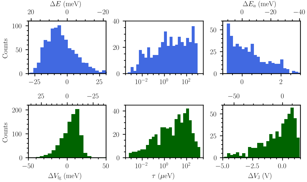
Figure 5.10: Distribution of the front gate corrections \Delta V_{\text{fg}} , \tau , and J -gate corrections \Delta V_J for electrons (in blue) and holes (in green). Top x-axes show the equivalent energy shift \Delta E computed using the ideal device lever-arm \alpha_{\text{fg}}^{0,e} = 0.72 for electrons and \alpha_{\text{fg}}^{0,h} = 0.75 for holes, and barrier height shift \Delta E_a extracted using the fits given in Figure 5.9.
