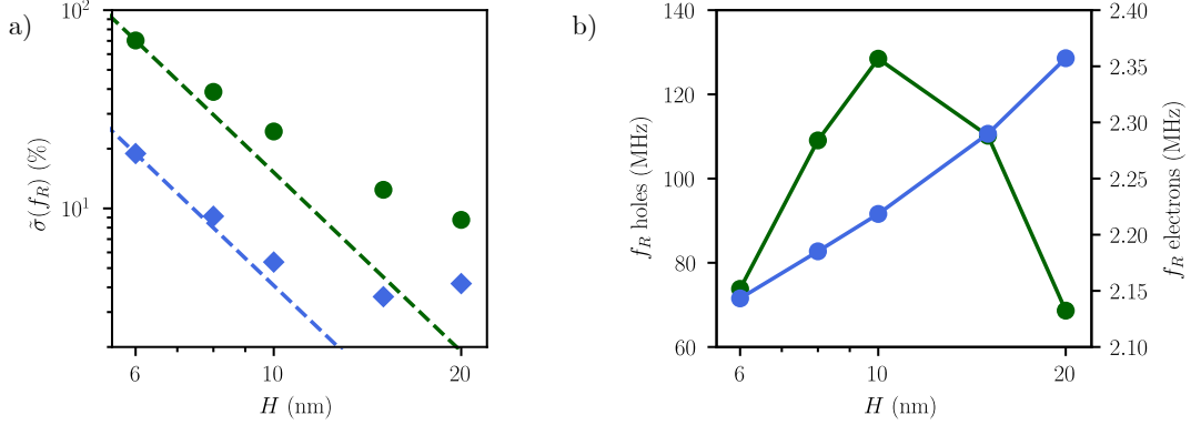
Figure 4.6: a) Dependence of the RSD \tilde{\sigma}(f_R) of the Rabi frequency of electrons (in blue) and hole (in green) qubits on the channel thickness H (interface roughness disorder with \Delta = 0.4 nm and L_c = 10 nm; V_{fg} = +50 mV for electrons and V_{fg} = -50 mV for holes). The dashed lines are \propto 1/H^3 extrapolations from H = 6 nm. b) Dependence of the Rabi frequency of electrons (in blue) and hole (in green) qubits for the pristine device on the channel thickness H .
