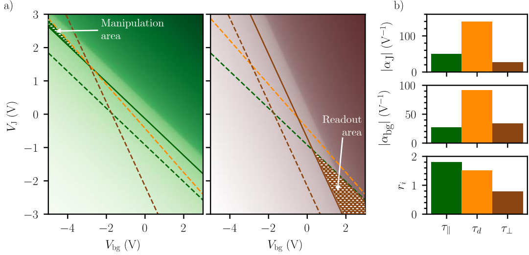
Figure 5.6: Properties of a device with optimized geometry. a) Tunnel maps for \tau_{\parallel} (left panel) and \tau_{\perp} (right panel). Color code as in Figure 5.4. b) Efficiency and selectivity on the control of \tau_{\parallel} (green), \tau_{\perp} (brown), and \tau_d (orange) with the back gate and the J-gates.
