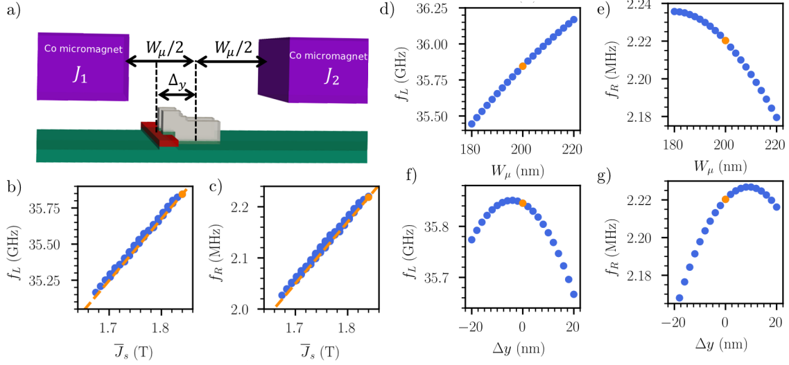
Figure C.6: a) Sketch of the device with the definition of the width W_\mu and misalignment \Delta y of the trench between the micro-magnets. b) Larmor and c) Rabi frequency of the pristine electron qubit as a function of the average magnetic polarization \bar{J}_s = (J_1 + J_2)/2 of the two micro-magnets. The plots collect data for different \Delta J = J_1 - J_2 ranging from -0.17 to 0.17 T. The orange lines are simple linear models f_R \propto \bar{J}_s and f_L \propto \bar{J}_s + J_0 , where J_0 accounts for the static magnetic field. d) Larmor and e) Rabi frequency as a function of the width W_\mu of the trench between the two magnets. f) Larmor and g) Rabi frequency as a function of the misalignment \Delta y between the channel and the trench. In all panels, V_{fg} = 50 mV and the orange point is the nominal device ( \bar{J}_s = 1.84 T, W_\mu = 200 nm, and \Delta y = 0 ).
