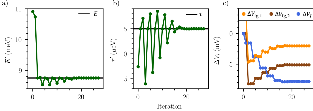
Figure B.2: Example of the convergence pattern of a disordered device using the algorithm shown in Figure B.1. a) Convergence of the anticrossing energy. Horizontal black line denotes the target energy E_0 . b) Convergence of the tunnel coupling. Horizontal black line denotes the target \tau_0 . c) Evolution of the gate corrections during the algorithm steps.
