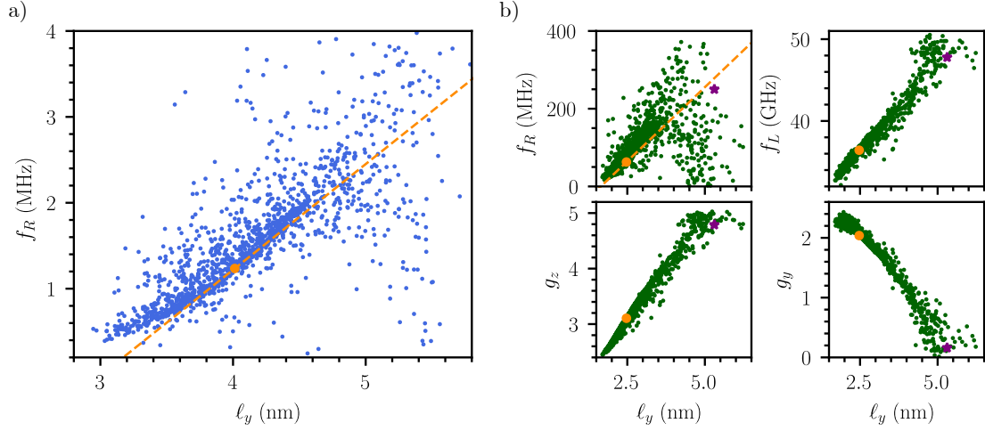
Figure 4.9: a) Correlations between the Rabi frequency f_R of the electron qubits and the extension \ell_y of the dots along \mathbf{y} . Each point is a particular realization of charge disorder at n_i = 5 \times 10^{10} \text{ cm}^{-2} and V_{\text{fg}} = 50 \text{ mV} . b) Correlations between the Rabi frequency f_R , the Larmor frequency f_L , the gyromagnetic factors g_y and g_z of the hole qubits and the extension \ell_y of the dots along \mathbf{y} at n_i = 5 \times 10^{10} \text{ cm}^{-2} and V_{\text{fg}} = -50 \text{ mV} . The orange point is the pristine device, and the purple star the disordered device of Figure 4.7d. The dashed orange line \delta f_R/f_R^0 = 4\delta\ell_y/\ell_y^0 for electrons and \delta f_R/f_R^0 = 3\delta\ell_y/\ell_y^0 for holes is a guide to the eye.
