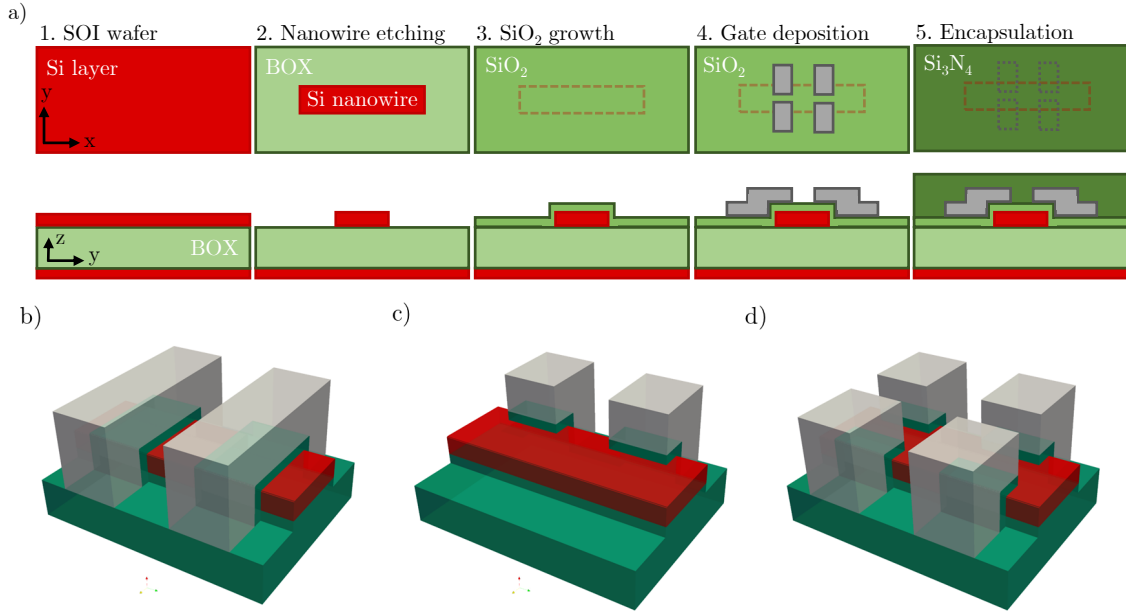
Figure 1.5: a) Schematic representation of the fabrication process of LETI devices. b) Illustration of a pump gates device. The BOX and SiO 2 are shown in green, the Si nanowire in red, and the gates in grey. The oxide covering the nanowire and the Si 3 N 4 are not shown for clarity. c) Illustration of a device with partly-overlapping gates. d) Illustration of a device with face-to-face gates.
