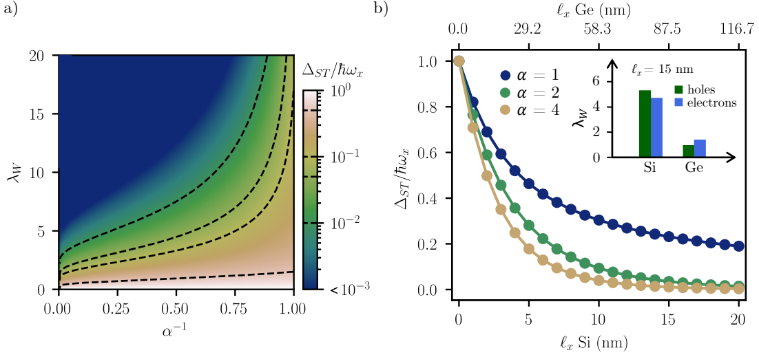
Figure 7.3: Singlet-triplet splitting \Delta_{ST} renormalization. a) Effect of Wigner ratio and anisotropy on \Delta_{ST} . b) Vertical cuts from a) at \alpha = 1, 2 , and 4 . The x axis has been translated from \lambda_W to dot size \ell_x for holes in Si and Ge using the relation given in the inset.
