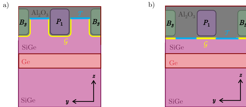
Figure E.1: Definition of the \mathcal{G} and \mathcal{T} areas of the devices in Figure 6.7 for a) the tips device and b) the planar device. We split the SiGe/Al 2 O 3 interface in the area below the gates (and surrounding them for the tips device), and the area in the space left without any overlapping gate.
