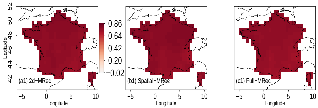
Figure S11. Order 1 Pearson autocorrelation for temperature using WFDEI reference during winter over the 1979-2016 period for the seasonal BC. Results are shown for MRec outputs for 2d-, Spatial- and Full-versions.
