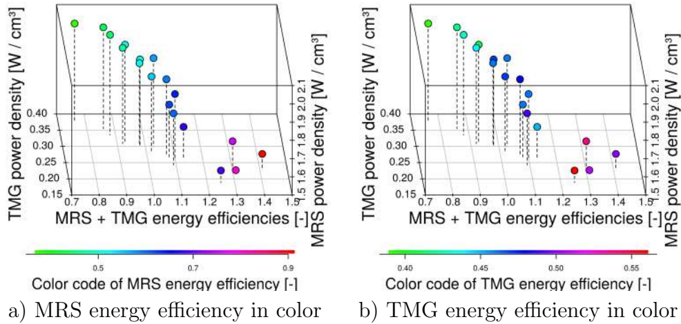
Figure 6.13: Pareto Fronts.
