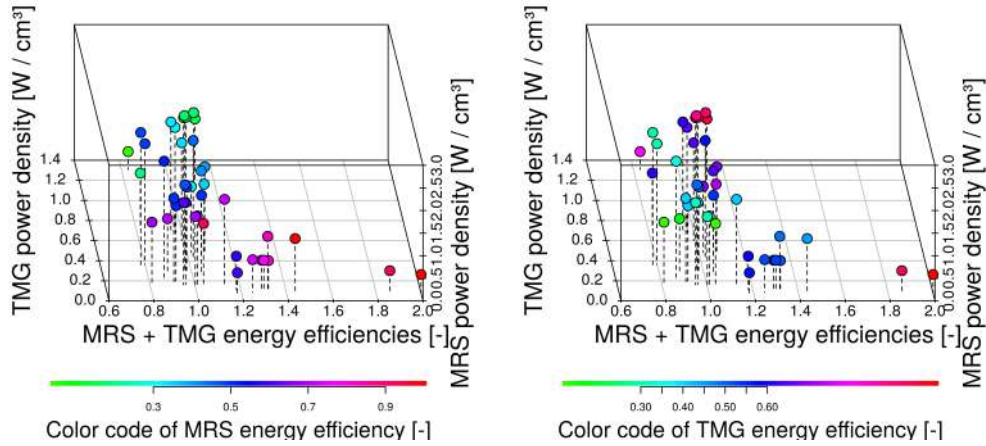
Figure 6.15: Pareto Fronts.
