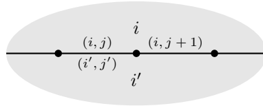
Figure 3.10: case 2 of Lemma 3.19
