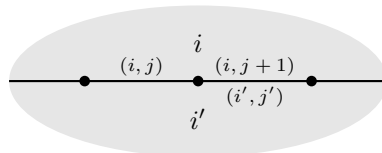
Figure 3.11: case 3 of Lemma 3.19
