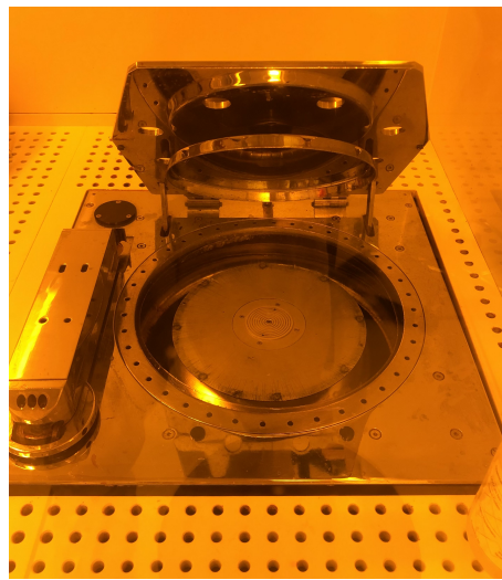
Figure 2.3: Spin coater.
