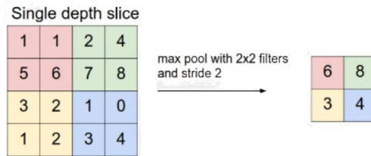
Figure 1.9: An example of a Max-Pooling process [23]
