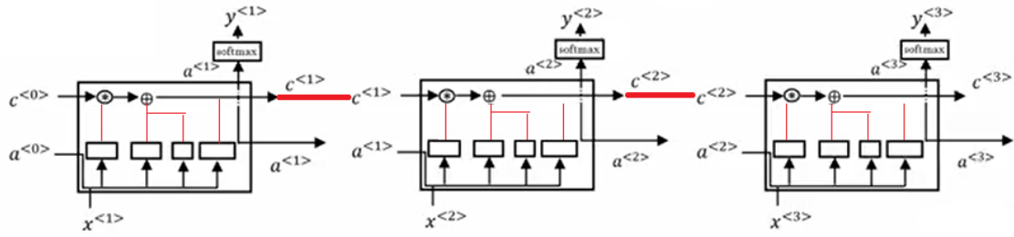
Figure 1.13: An example of LSTM architecture [24]
