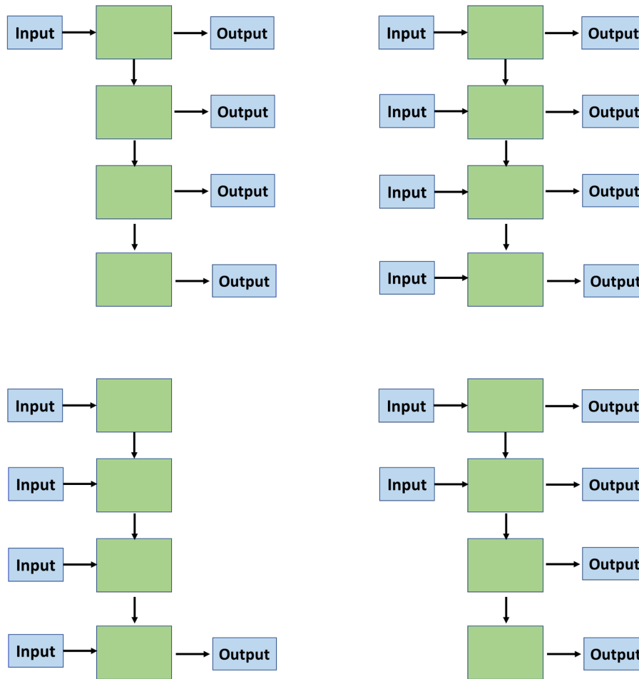
Figure 1.12: The different types of RNN
