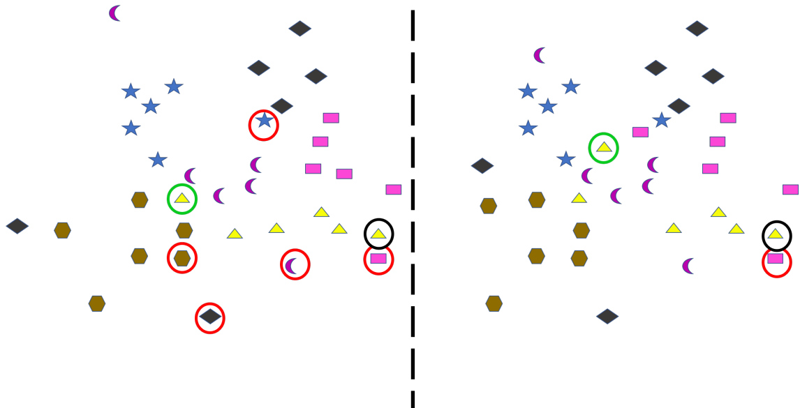
Figure 4.11: Iteration 2; Steps 1+2 (Multipler loss on the left and Triplet loss on the right)
