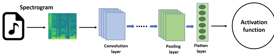
Figure 3.4: Emotion recognition using CNN
