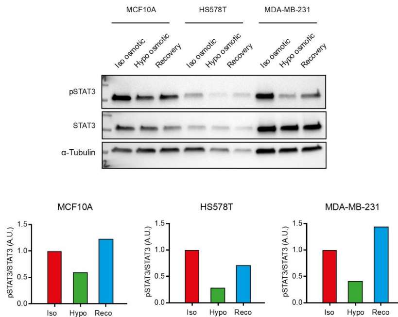
Figure 30: IFN- \alpha -induced STAT3 activation in breast cancer cells upon hypo-osmotic shock
