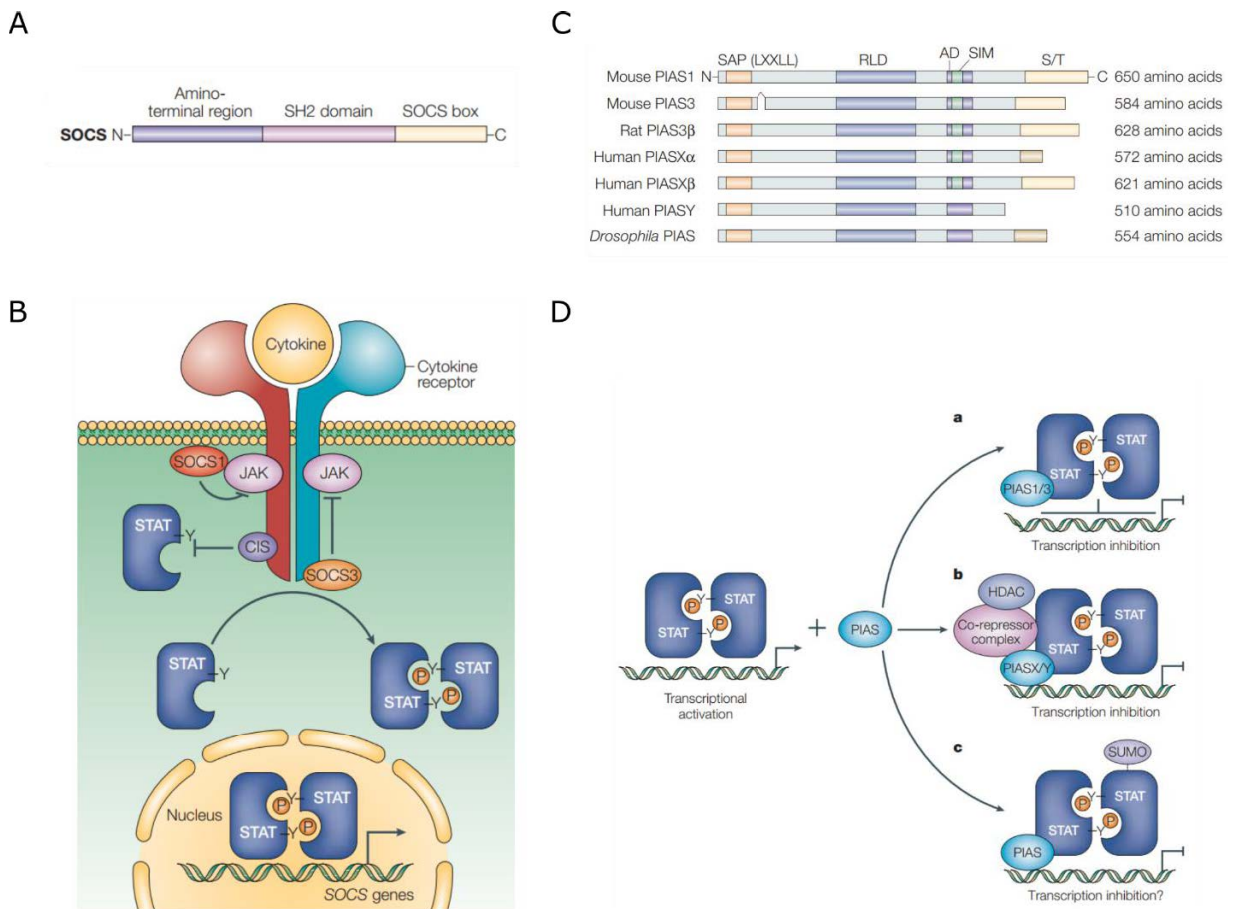
Figure 20: SOCS and PIAS family of JAK-STAT regulators
