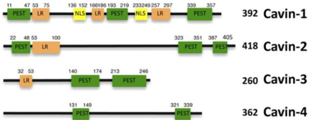
Figure 7: The cavin family of proteins
