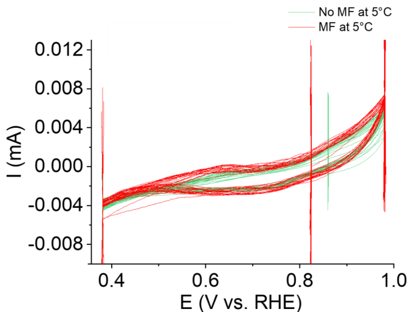
Appendix 5. Cyclic voltammograms of empty microelectrode at 5 °C in O 2 -saturated 0.1 M KOH without magnetic field (green) and with magnetic field (red).
