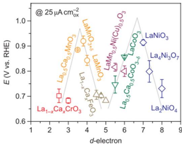
Figure 9. ORR activity of perovskite transition-metal-oxide catalysts. Potentials at 25 \mu\text{A cm}^{-2}_{\text{ox}} of the perovskite oxides as a function of the average d-electron number of B-site cations. Data symbols vary with type of B ions (Cr, red; Mn, orange; Fe, grey; Co, green; Ni, blue; mixed compounds, purple), where x = 0 and 0.5 for Cr, and 0, 0.25 and 0.5 for Fe. Errors bars represent standard deviations of at least three measurements. 47
