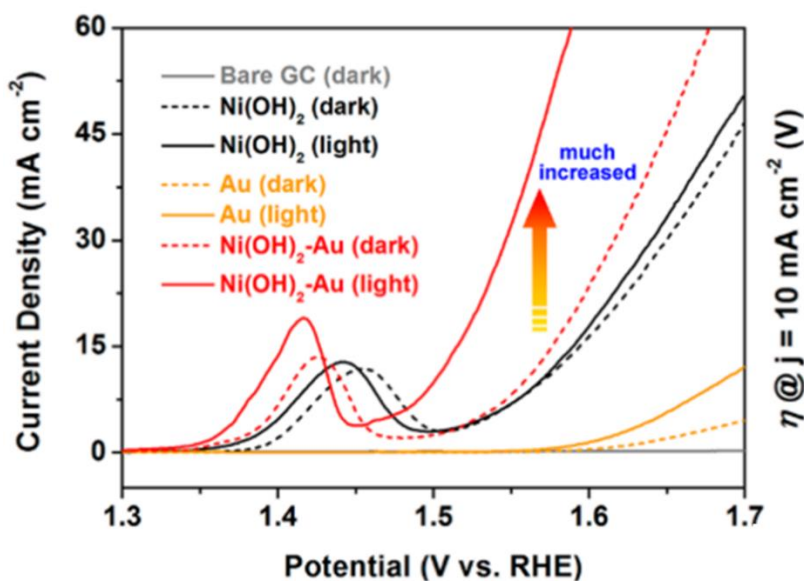
Figure 12. OER polarization curves of Ni(OH) 2 -Au hybrid catalyst and control samples measured in 0.1 M KOH electrolyte with and without light irradiation (523 nm laser). 77
