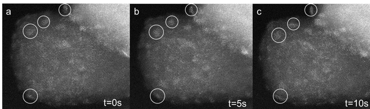
Figure 10. Snapshots acquired by TEM of STO-Pt 10 at.% at (a) t=0 , (b) t=5 s and (c) t=10 s.
