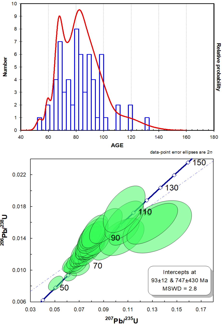
Figure 1. Probability density plot and Wetherill Concordia diagram for sample PB1.
