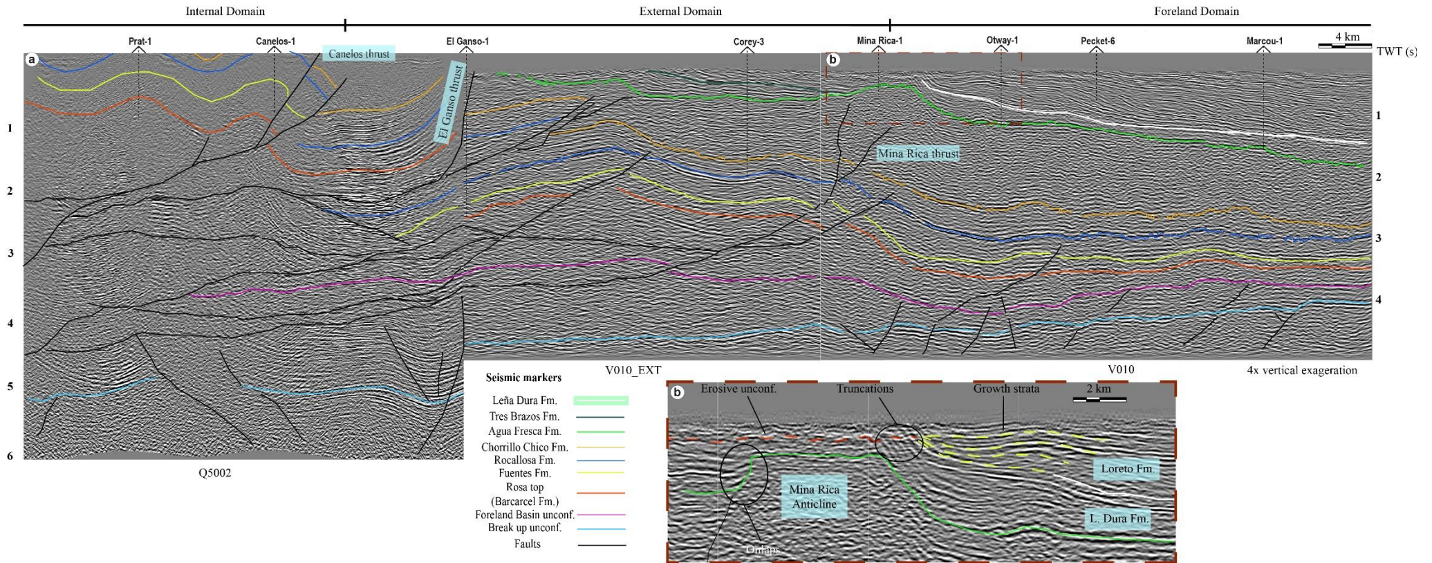
Figure 4. (a) Structural interpretation of the regional seismic profile of Fig. 3. Note structural duplex in the deepest part of the internal domain involving the Erezcano, Canal Bertrand and Latorre formations. (b) Structural and seismostratigraphic interpretation of the Mina Rica anticline, evidencing the syntectonic nature of the late Eocene Loreto Formation. Uninterpreted seismic lines at the end of this chapter.
