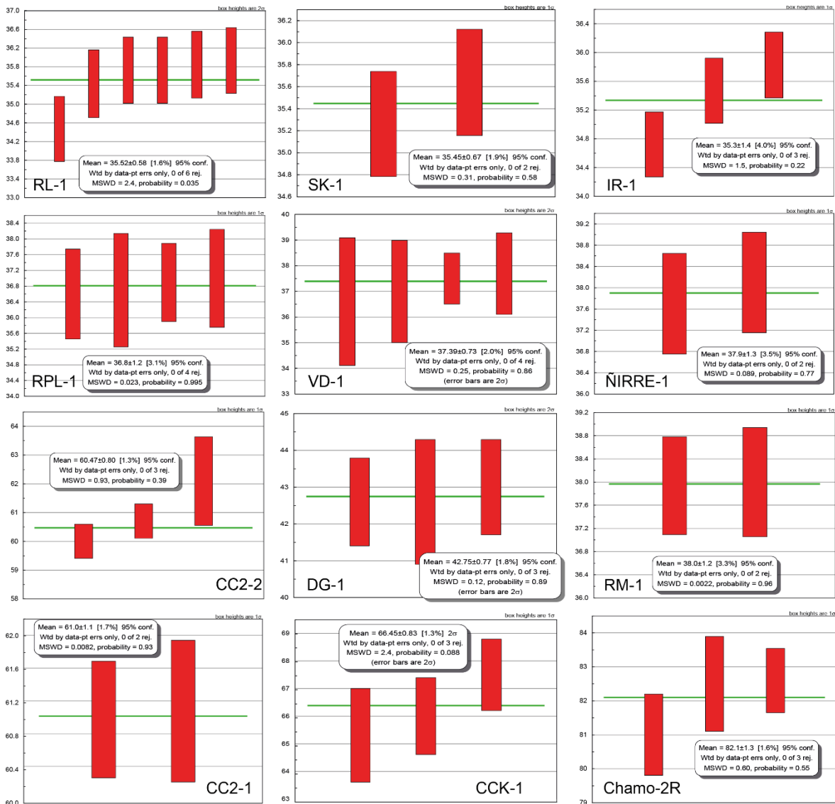
Figure 4. Weighted mean ages plots showing calculated MDA's for the new 21 detrital zircon samples (excluding TBD-H1, CC2-3, and CC1 samples for which was employed YSG1σ metric and TB1 which does not yield near-depositional zircon ages). Individual zircon age uncertainty (error bars at 1σ or 2σ) is indicated on the upper right side of each panel. MSWD = mean squared weighted deviation.
