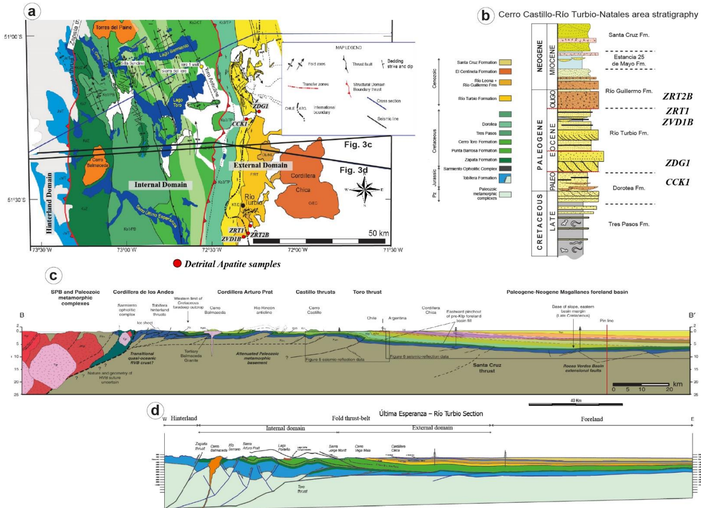
Figure 2. (a) Geological map and distribution of detrital apatite samples in the Cerro Castillo-Río Turbio-Natales study area. (b) Stratigraphic position of detrital apatite samples. (c) Regional structural basin configuration model of Fosdick et al., 2011. (d) Structural configuration model of Ghigliione et al., 2014.
