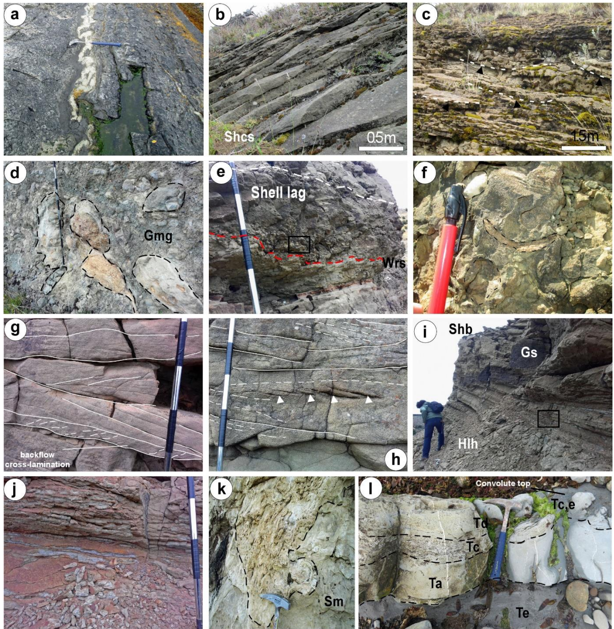
Figure 4. (a) Slump structures in the Fuentes Formation. (b) Amalgamated beds of hummocky and swaley cross-stratification of FA4. (c) Swaley cross-stratification in FA4. (d) Example of mudstone/sandstone blocks in FA7. (e) Shell lag and wave ravinement surface (Wrs) on the fluvial channels marking the start of TST in section Cerro Pelario. (f) Close-up of shells and bivalve moulds. (g) Herringbone and bidirectional cross-stratification in estuary deposits (FA8), section Sierra Dorotea. (h) Tangential, cross-bedding with reactivation surfaces and tidal bundles. (i) Example of low-angle inclined heterolithic units overlain by tidal creek channels in FA8b. (j) Close-up of heterolithic facies. (k) Plan view of contorted bedding in the Chorrillo Chico Formation in section Rio Blanco. (l) Bouma sequence in turbidite deposits of the FA9. Jacob's staff divisions each 10 cm.
