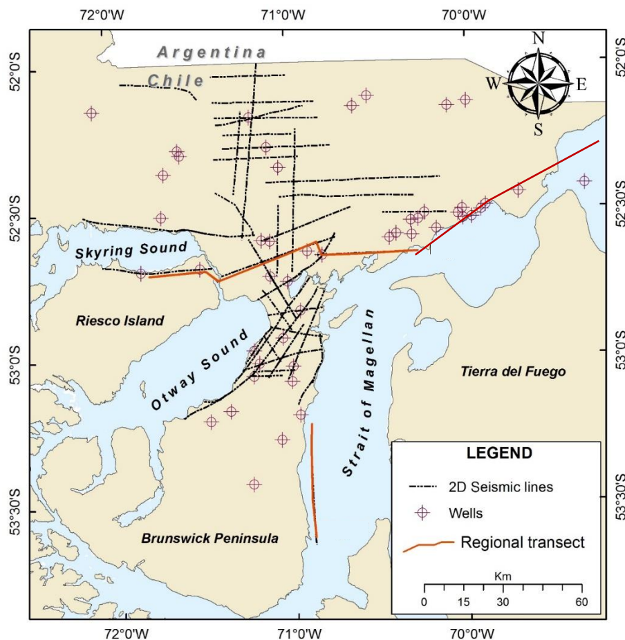
Figure 1. Geographic distribution of 2D seismic lines and exploratory wells (courtesy of ENAP) in the study area.
