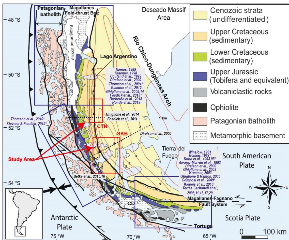
Figure 1. Morphotectonic setting of the Southern Patagonian orogenic wedge and Magallanes-Austral foreland basin. Red isopach lines are the depth to top-Tobífera Formation (Late Jurassic). Blue boxes are areas that concentrate most of previous structural and thermochronological (references with asterisks) studies. Red boxes are study areas, enlarged in Figs. 2 (CTN: Cerro Castillo-Río Turbio-Natales area) and 3 (SKB: Skyring Sound-
