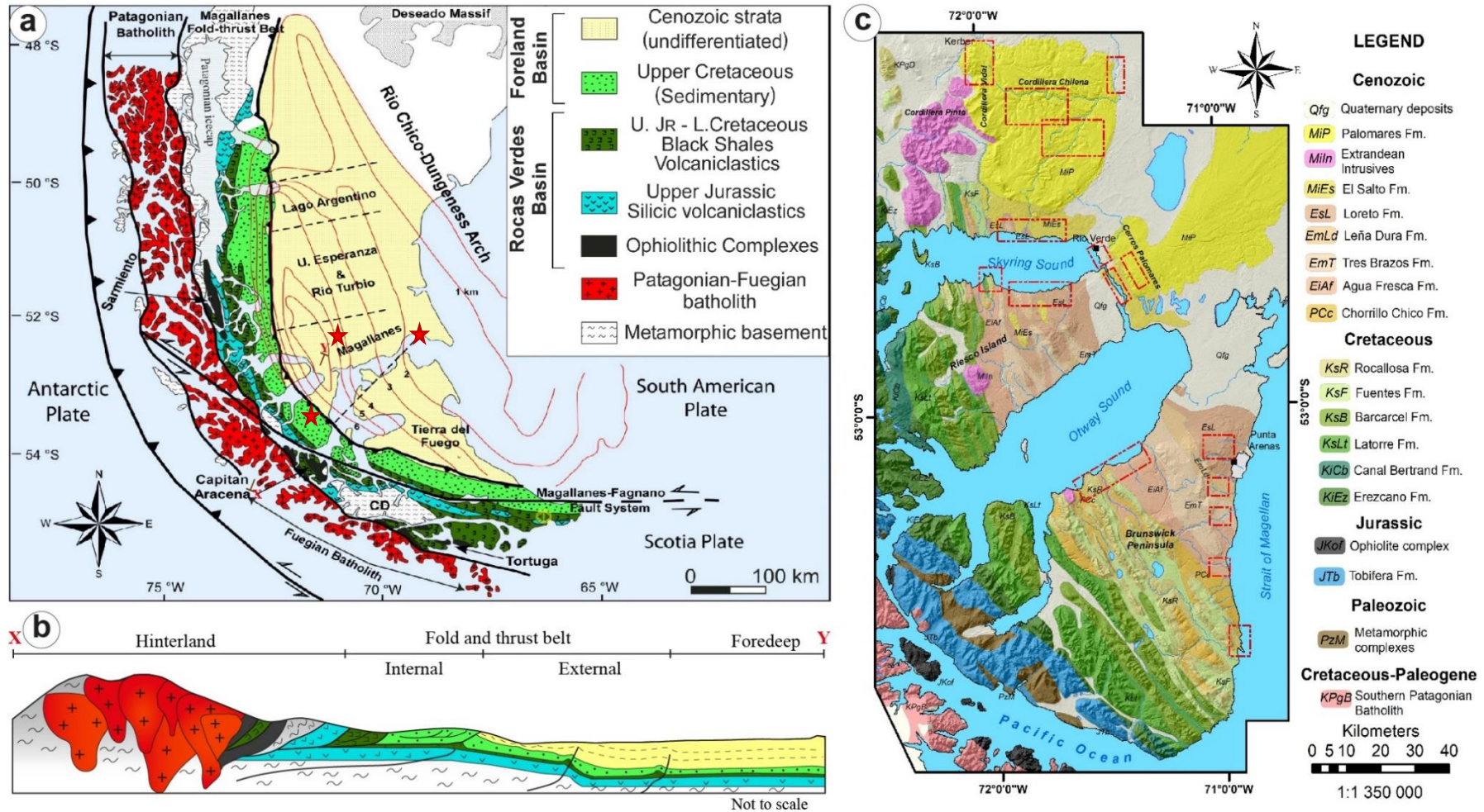
Figure 1. (a) The morphotectonic setting of the Magallanes-Austral foreland basin (modified from Rivera et al., 2020). Red stars for highlight position of subsidence curves in Fig. 9. Red isopach lines are the depth to top-Tobífera Formation (Late Jurassic). (b) A schematic structural transect of the orogenic wedge and foreland showing the location of different potential source terranes. (c) Simplified geologic map of the study area showing the stratigraphic sections (red boxes).
