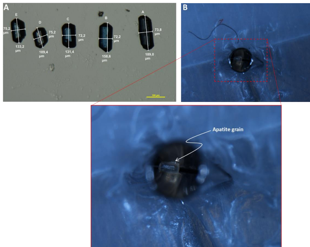
Figure 6. A. Selection and measurement of 5 aliquots of the best apatites crystals. B. Packing into a platinum capsule to posterior degassing phase. Experimental protocol conducted at the GET lab.
