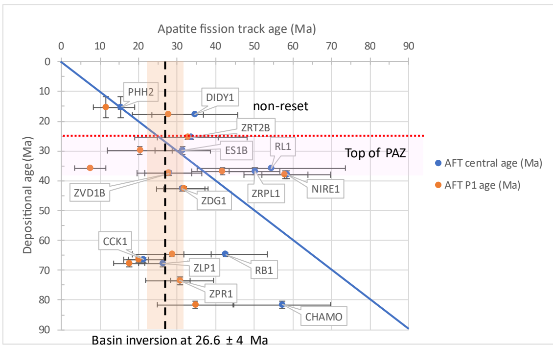
Figure 10. Biplot of AFT ages versus Depositional ages from studied samples. The blue line represents similar AFT and MDA (ratio 1:1).
