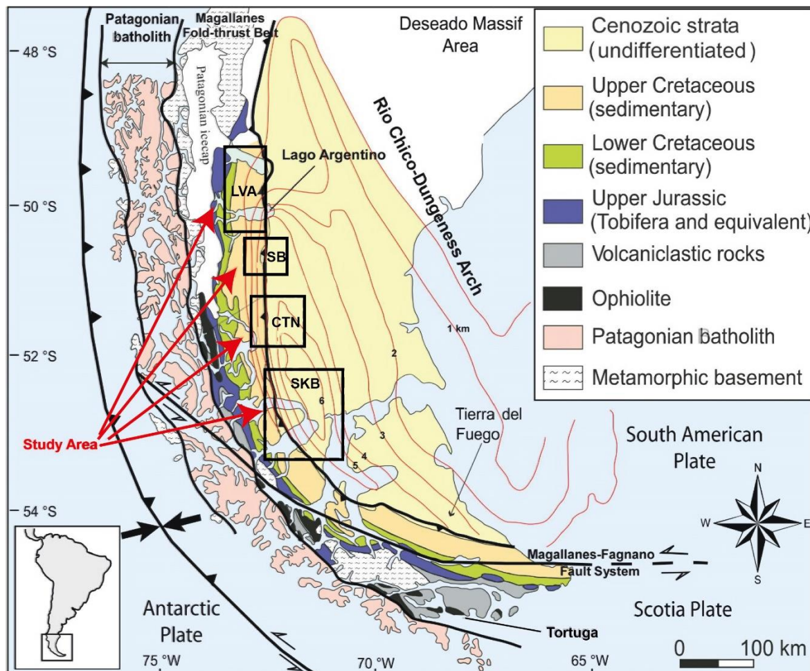
Figure 1. The morphotectonic setting of the Magallanes-Austral foreland basin (modified from Fildani et al., 2008). Contours indicate foreland sediment thickness (after Ghigliione et al., 2009). The black boxes indicate the location of the study areas.
