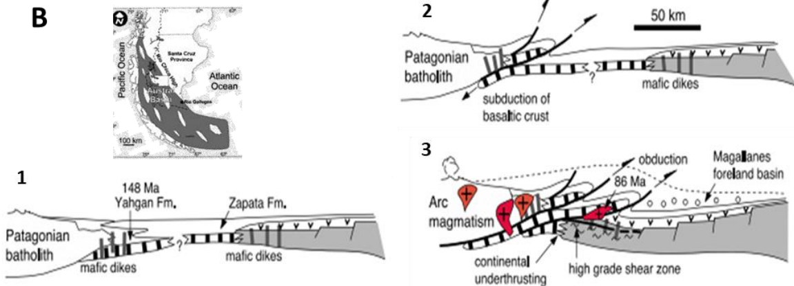
Figure 5. A. Simplified morphotectonic map of the Magallanes-Austral Basin. The black dashed-line box indicates the location of the study areas (see details in Fig. 6). Red isopach lines are the depth to top-Tobífera Formation (Late Jurassic). B. Geographic distribution of the Rocas Verdes Basin and schematic representation of different closure stages (1=final basin stage; 2= westward underthrusting of oceanic crust; 3= obduction and foreland basin formation) during the Late Cretaceous (modified from Klepeis et al., 2010).
