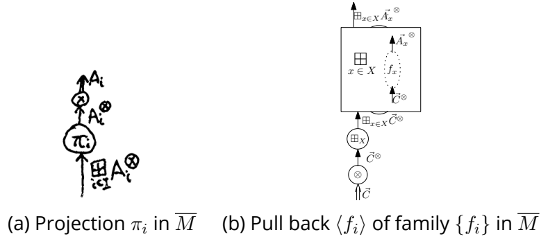
Figure 4.10: Product in \overline{M}
