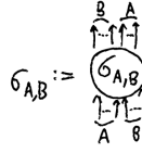
Figure 4.4: Definition of \sigma_{\vec{A}, \vec{B}}
