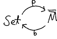
Figure 4.17: Adjunction for !-comonad
