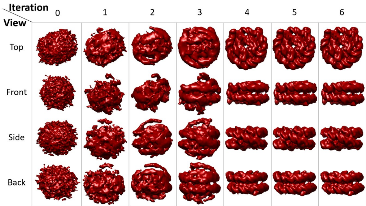
Figure 47 Subtomogram averaging applied to the synthetic nucleosome subtomograms. A reference-free alignment was performed using Fast Rotational Matching
