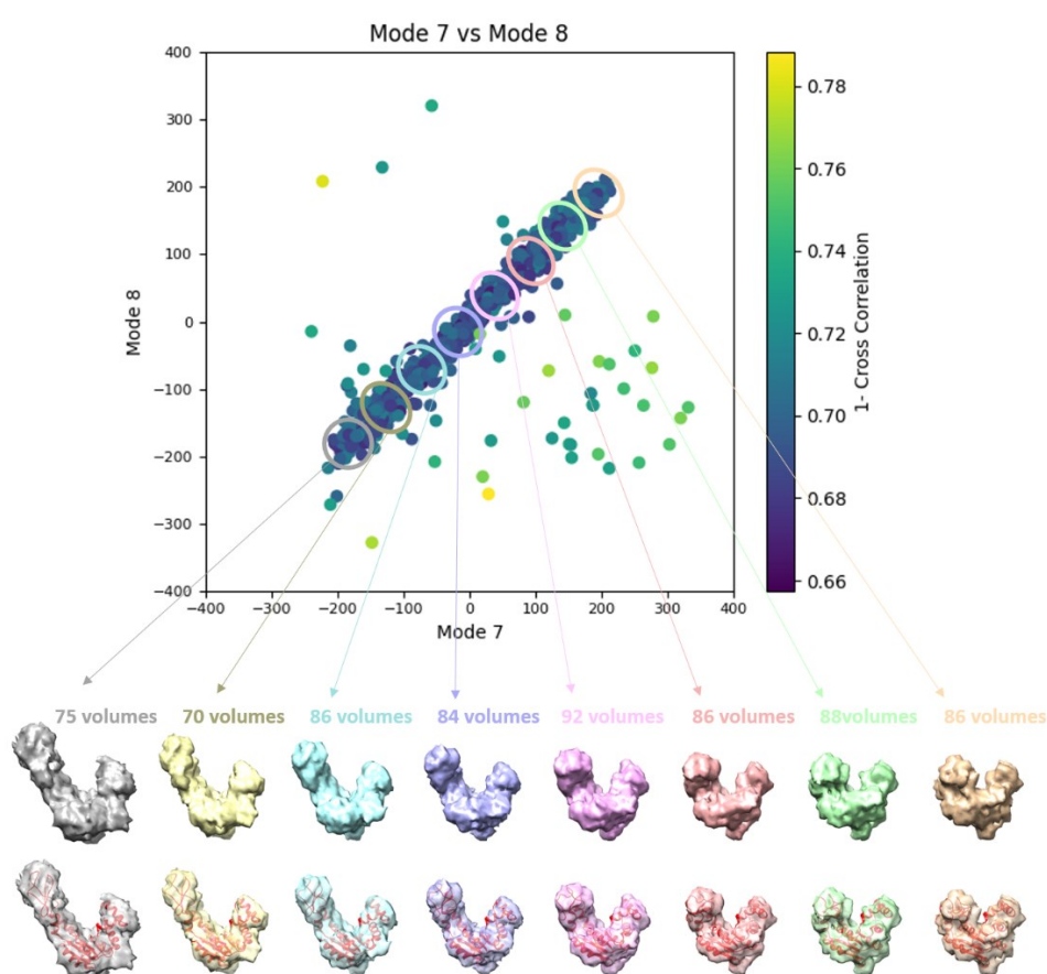
Figure 40 Averages of eight groups (enclosed by ellipses) of subtomograms identified from the output of the 3D-to-3D elastic and rigid-body alignment module of HEMNMA-3D with “Continuous” dataset, using the atomic structure (chain A of PDB:4AKE) and its normal modes to estimate the conformational parameters (normal-mode amplitudes) and rigid-body parameters (orientation and shift) of the molecules in the input synthetic subtomograms. Subtomograms are represented by points, and close points represent similar conformations. The numbers of volumes written above the shown subtomogram averages are the numbers of synthetic subtomograms used for computing these subtomogram averages (the numbers of points enclosed by the corresponding ellipses). On the bottom, the subtomogram averages are shown at 50% transparency along with the corresponding theoretical centroid deformed atomic structure (in red).
