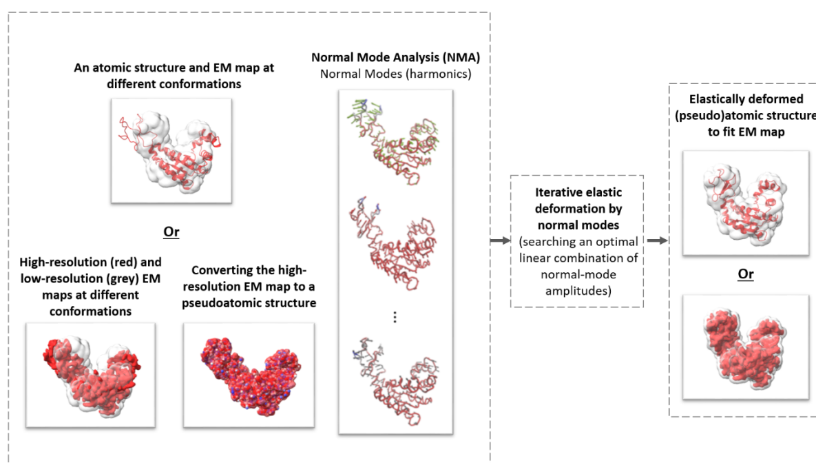
Figure 23 The general scheme of elastic deforming of a reference structure (atomic or pseudoatomic) using normal modes to fit a density map (e.g., an EM map or a subtomogram average).
