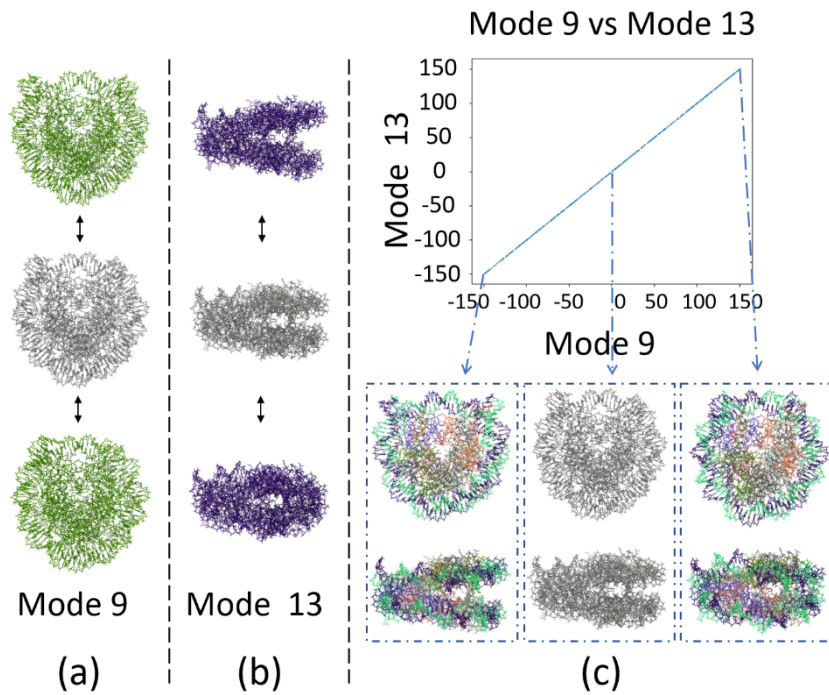
Figure 45 Synthesized combined breathing and gaping motions of the nucleosome (PDB 3w98 structure): (a) nucleosome breathing motion, (b) nucleosome gaping motion, (c) generated ground-truth conformational distribution (top) comprising 1000 synthetic nucleosome shape variants obtained by a linear combination of modes 9 and 13, with a linear dependence between the normal-mode amplitudes (blue points in the plot), and 3 representative shapes (bottom) corresponding to the two ends and the middle of the conformational distribution.
