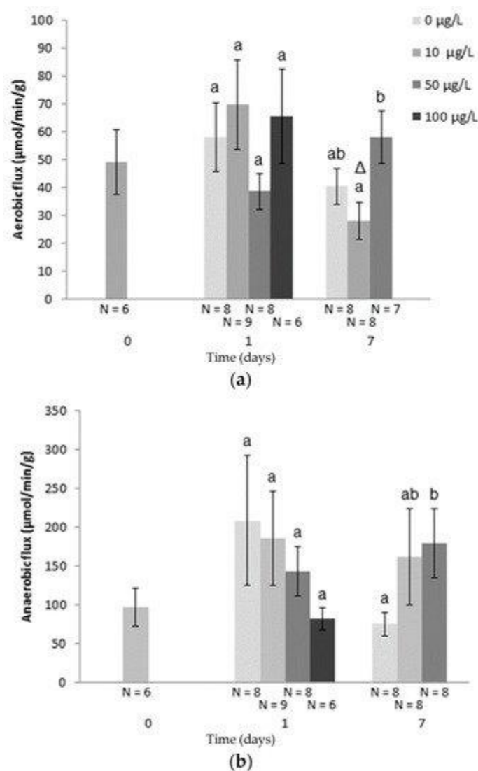
Figure 1. (a) Aerobic flux ( \mu\text{mol/min/g} ) and (b) anaerobic flux ( \mu\text{mol/min/g} ) in white muscle of juvenile roach during Cu exposure. Bars represent S.E. Different letters indicate significant differences for the same time point. \Delta indicates significant differences for the same concentration among individual samples at T1 and T7.
