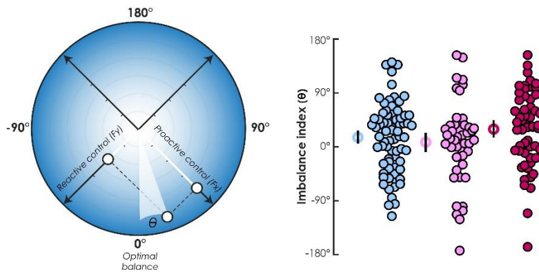
Figure 6. Left panel: circular projection of the resultant vector of predictive (i.e., belief) and reactive (i.e., PE+) control forces. 0^\circ represents the optimum balance between these two orthogonal forces. The angle of the resultant force indicates imbalance toward either predictive ( \theta > 0^\circ ) or reactive ( \theta < 0^\circ ) control. The right panel shows the distribution of this imbalance index for each of the three groups. Error bars represents 95% bootstrapped CI of the mean.
