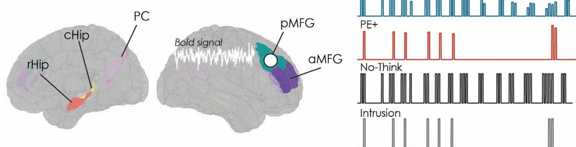
Figure 3. DCM models. (A) Families expressing different hypotheses on the involvement of intrusion beliefs and PE+ computations in modulation of the coupling between control regions (anterior and posterior middle frontal gyrus, MFG) and memory target regions, including the rostral hippocampus (rHIP), caudal hippocampus (cHIP), and precuneus (PC). It should be noted that null models were also estimated, but are not shown here. (B) Pathways capturing the seven possible connections between control and target regions. (C) Left panel shows the regions of interest used for DCM analysis. Right panel provides an illustration of the modularity inputs influencing the connectivity between brain regions.
