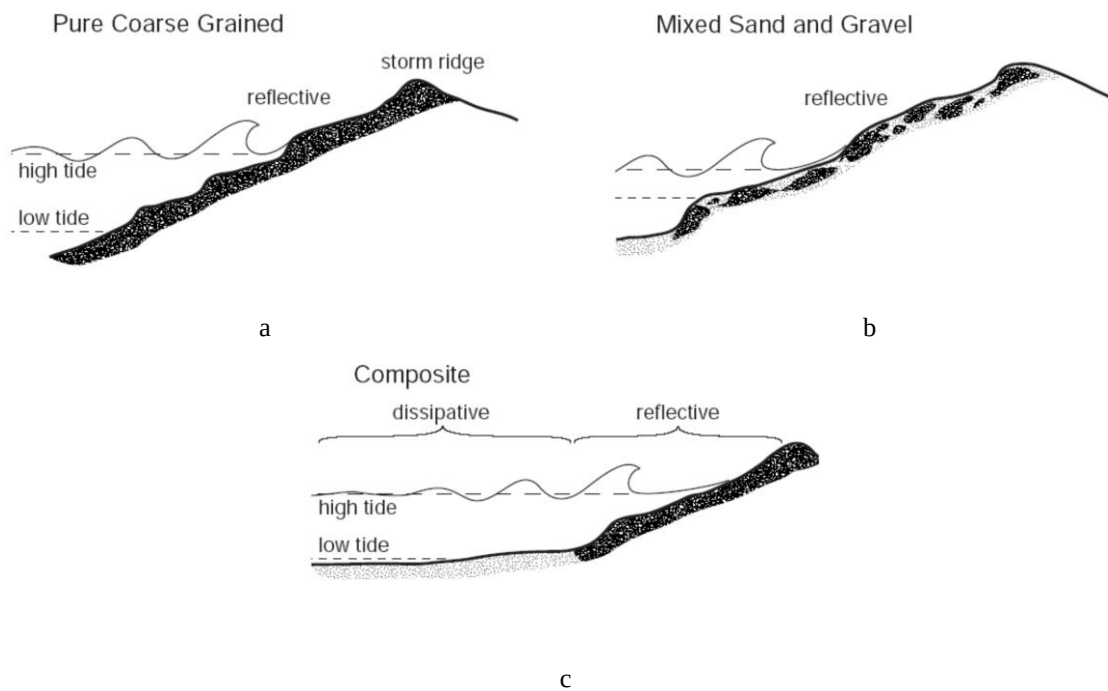
Figure 5 – Main types of gravel beaches according to the classification of Jennings and Shulmeister (2002) modified after Napier City Council (2007)
