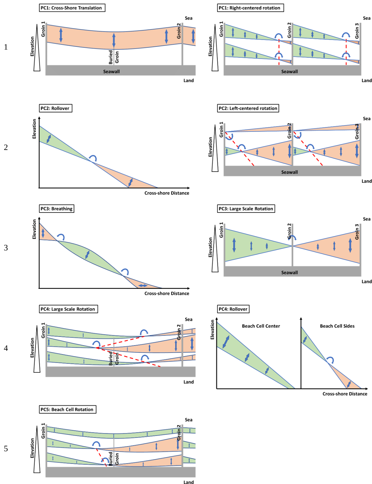
Figure 61 - Conceptual model of the isolated mechanisms of beach morphological variability in Etretat (left) and Hautot-sur-Mer (right), associated with their corresponding principal component (PC).
