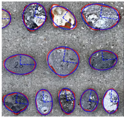
Figure 33 - Comparison between sediment particles' shape as detected with Mask R-CNN (red) and the ellipse fitted around this shape (blue). The ellipses' major and minor axes are displayed as dashed blue lines.
