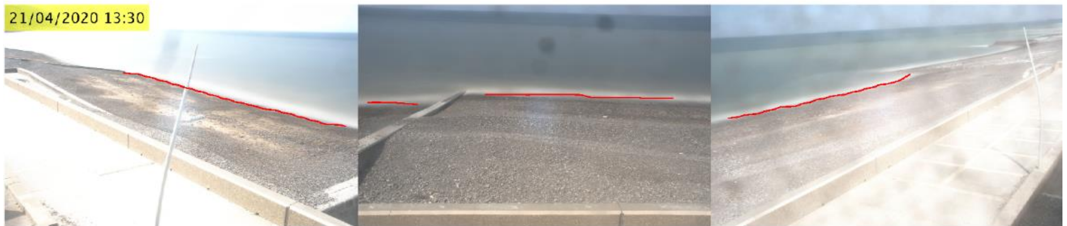
Figure 50 - Example detected waterlines on the 3 cameras of the Hautot-sur-Mer's VMS
