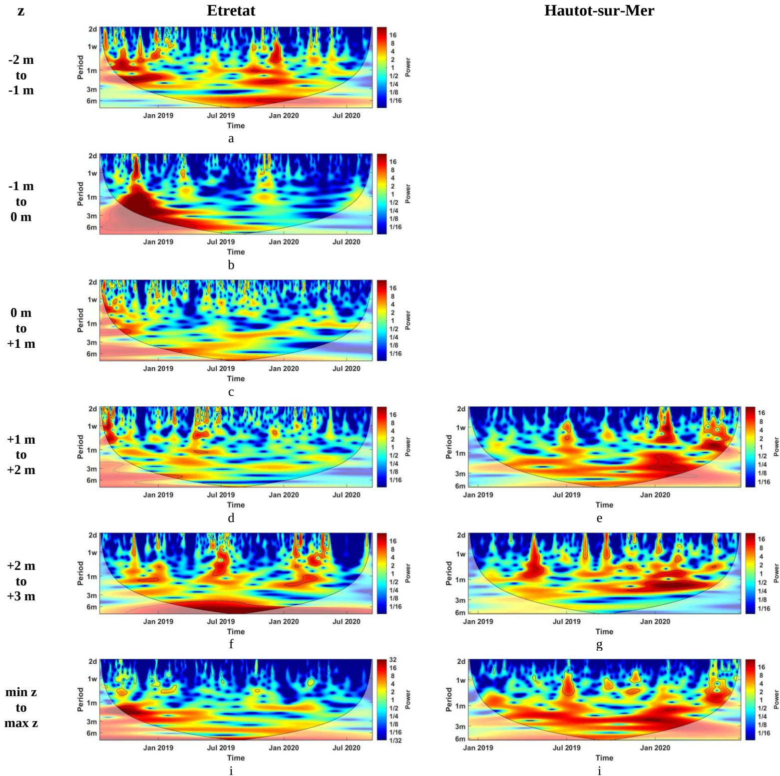
Figure 74 - Wavelet spectrums of beach slope (BS) between various elevations (z) in Etretat (left) and Hautot-sur-Mer (right)
