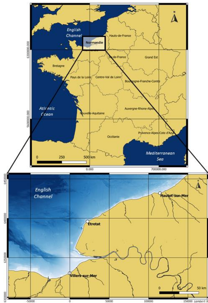
Figure 22 - Location map of Villers-sur-Mer, Etretat and Hautot-sur-Mer, in Normandy, France
