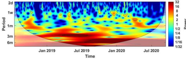
Figure 75 - Wavelet spectrums of the temporal eigenfunctions C_k(t) resulting from the EOF analysis applied to a dataset of 3D daily shoreline position in Etretat (left) and Hautot-sur-Mer (right). Each row corresponds to a specific principal component (PC).
