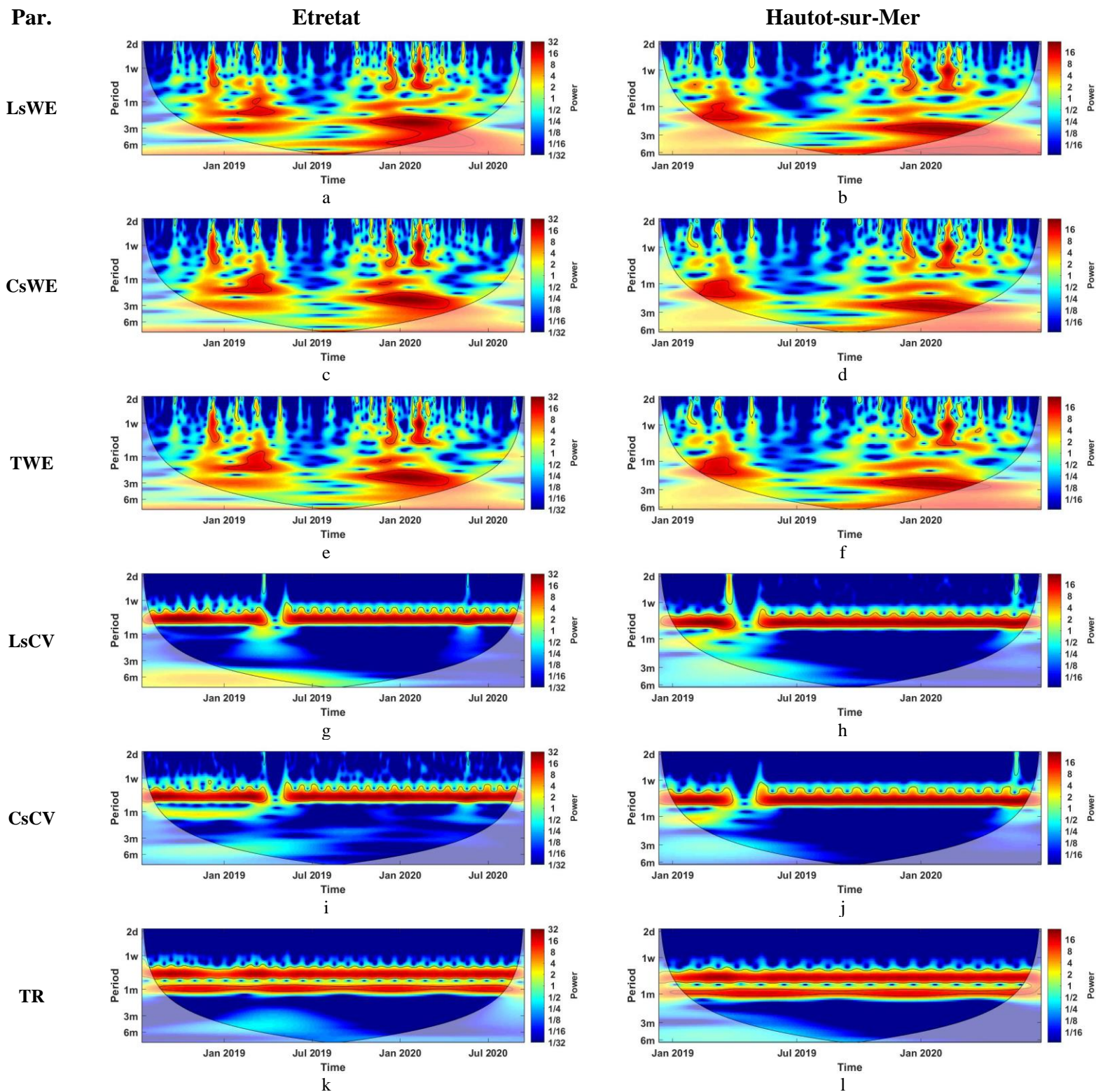
Figure 76 - Wavelet spectrums of hydrodynamic parameters in Etretat (left) and Hautot-sur-Mer (right). Parameters include longshore wave energy (LsWE) (a, b), cross-shore wave energy (CsWE) (c, d), total wave energy (TWE) (e, f), longshore current velocity (LsCV) (g, h), cross-shore current velocity (CsCV) (i, j), tidal range (TR) (k, l).
