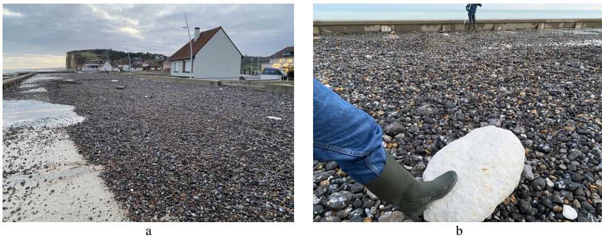
Figure 20 - Washover sediment found on top of the seawall of Hautot-sur-Mer after Storm Ciara on 2020/02/14 (Credit: A. Soloy, 2020)
