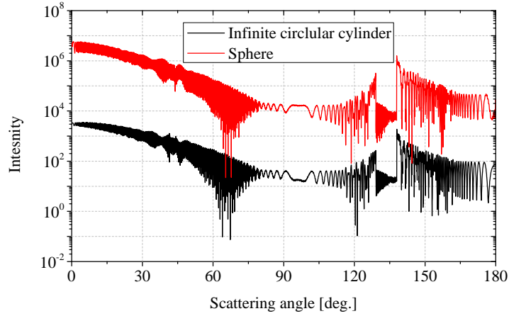
Figure 2.12 – Comparison the scattering diagrams of a sphere and infinite circular cylinder. The incident plane wave with wavelength \lambda = 0.6328 \mu\text{m} is in perpendicular polarization. The radius of particle and its refractive index are a = 100 \mu\text{m} and m = 1.333 .
