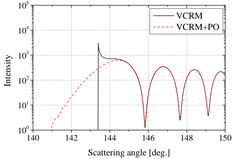
Figure 5.7 – Scatting diagrams of an infinite elliptical cylinder in the rainbow region, same parameters with Figure (5.6) except a = 100 \mu\text{m} , b = 95 \mu\text{m} .
