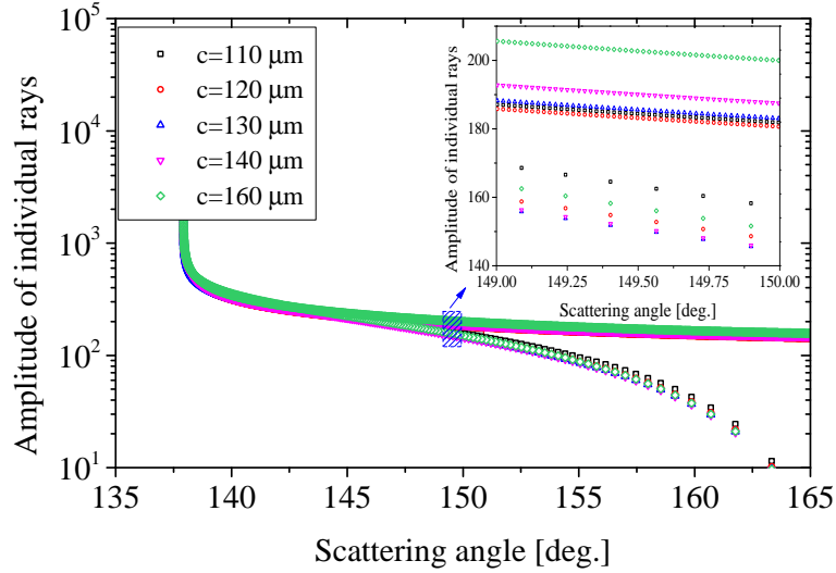
Figure 5.16 – Amplitude of the individual rays p = 2 of an prolate ellipsoid near rainbow. Same parameters as in Figure 5.13.
