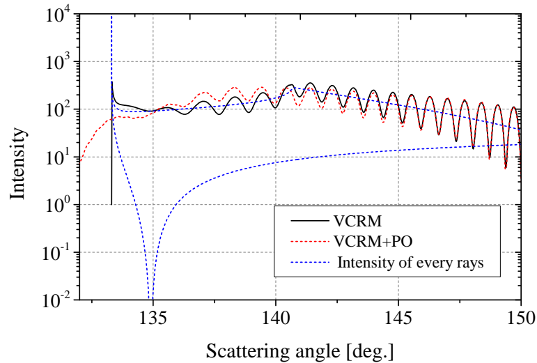
Figure 5.8 – Scatting diagrams of an elliptical cylinder near rainbow region with particle size in a = 95 \mu\text{m} , b = 100 \mu\text{m} and wave in parallel polarization for p = 2 .
