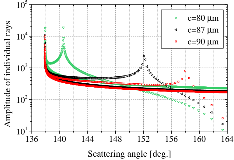
Figure 5.19 – The scattering field of an oblate spheroid near rainbow region, same parameters as in Figure 5.17.
