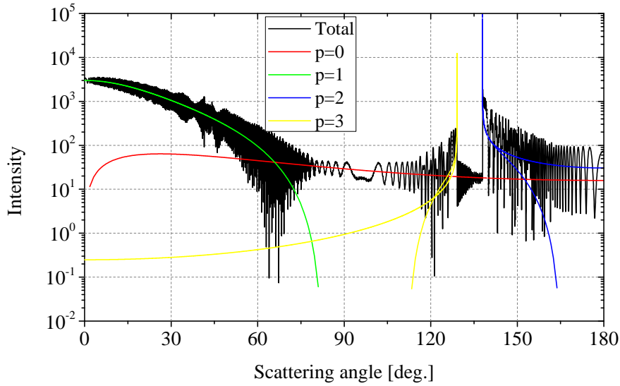
Figure 2.10 – Scattering diagrams of an infinite circular cylinder. The incident plane wave with wavelength \lambda = 0.6328 \mu\text{m} is in perpendicular polarization. The radius of particle and its refractive index are a = 100 \mu\text{m} and m = 1.333 .
