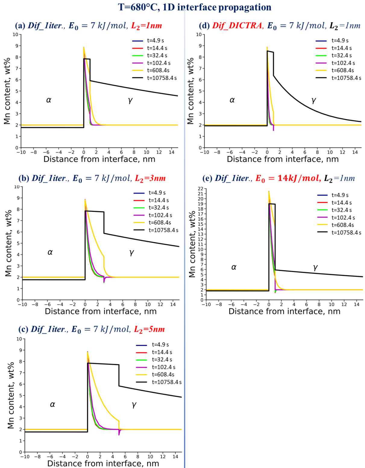
Figure 5.15. Mn profiles simulated at T=680^\circ\text{C} with variable velocity considering “1D” interface propagation using ‘Huin’ model with different diffusion coefficients ( Dif\_iter and Dif\_DICTRA ), binding energy values (7 and 14 kJ/mol) and thicknesses of the interfacial zone (1 nm, 3 nm and 5 nm).
