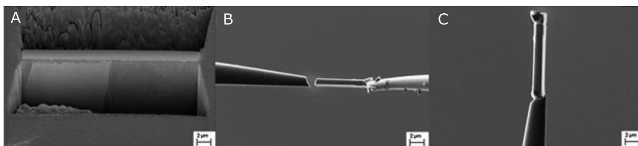
Figure 2.12. Site-specific lift-out for interface analysis on austenitic steel: (A) SEM image of the milled wall perpendicular to previously selected interface; (B) specimen mounting parallel to a support tip; (C) specimen mounted on the support tip, ready for annular milling [112].
