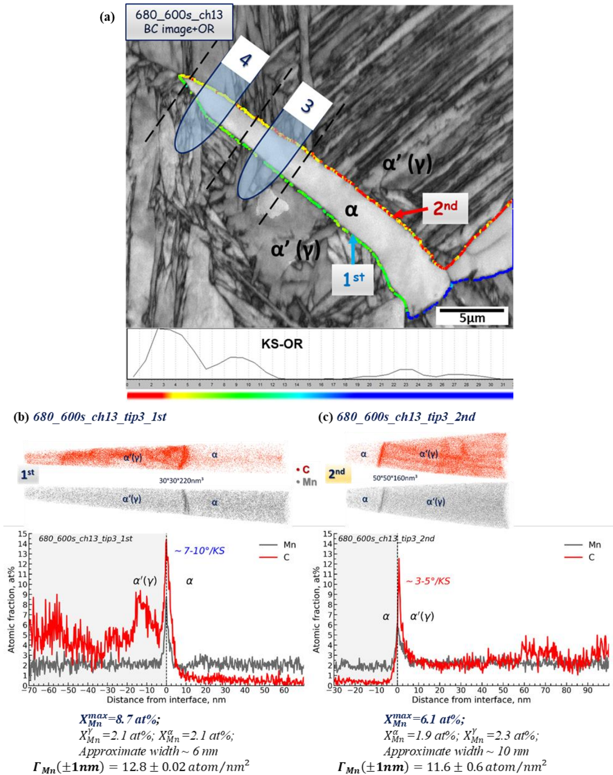
Figure 3.26. (a) IQ map of selected ROIs with the thin allotriomorph ferrite grains formed after isothermal holding at 680°C during 600s (680_600s_ch13). Colors at \alpha' ( \gamma )/ \alpha interfaces represent the orientation relation between ferrite and prior austenite at 680 °C. It is expressed as the orientation difference with respect to the KS orientation relationship. 3D reconstructions and concentration profiles of C and Mn atoms across the 1 st . (b), and 2 nd (c) \alpha/\gamma interfaces of tip3.
