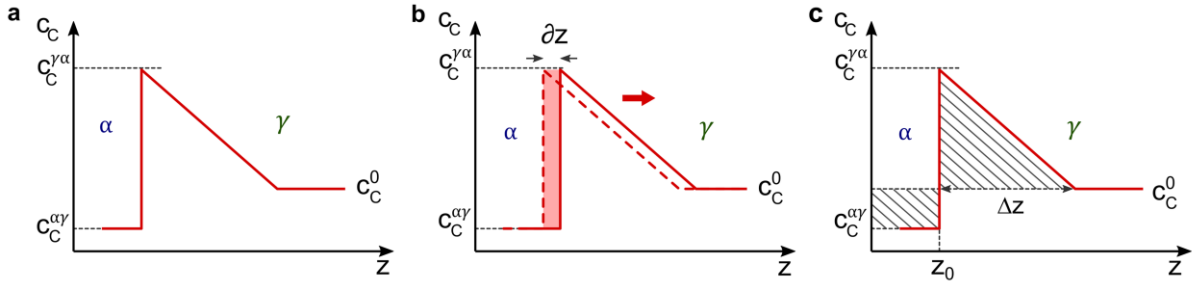
Figure 1.10. The evolution of carbon concentration profile at the \gamma/\alpha interface during the diffusion-controlled mode of phase transformation.
