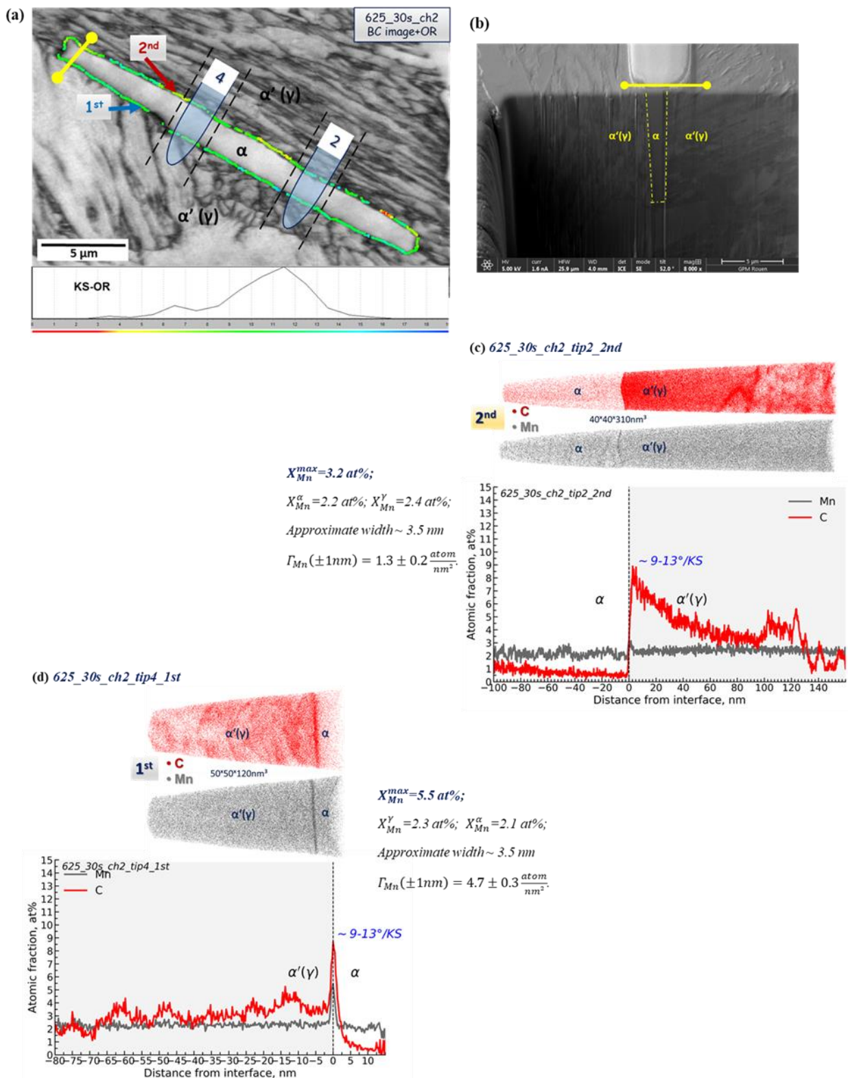
Figure 3.14. (a) IQ map of the selected region with the allotriomorph ferrite formed after isothermal holding at 625°C during 30s ( 625_30s_ch2 ). Colors represent the orientation difference with respect to KS-OR of the initial ferrite–austenite orientation relationships at 625 °C. (c) 3D reconstructions and concentration profiles of C and Mn atoms across the 2 nd interface of tip2 and. (e) across the 1 st interface of tip4.
