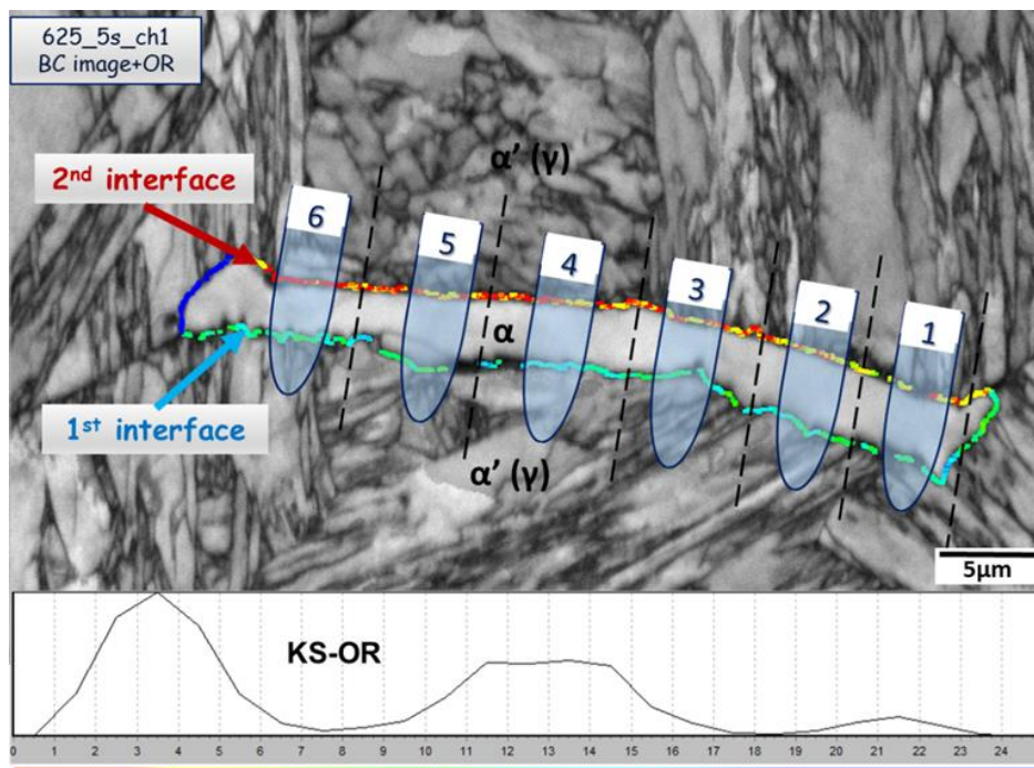
Figure 3.6. IQ maps of the selected region with an allotriomorph ferrite formed at the prior austenite grain boundary after isothermal holding at 625°C during 5s. Colors at \alpha'(\gamma)/\alpha interfaces represent the orientation relation between ferrite and former austenite at 625°C, expressed as the orientation difference with respect to KS-OR.
