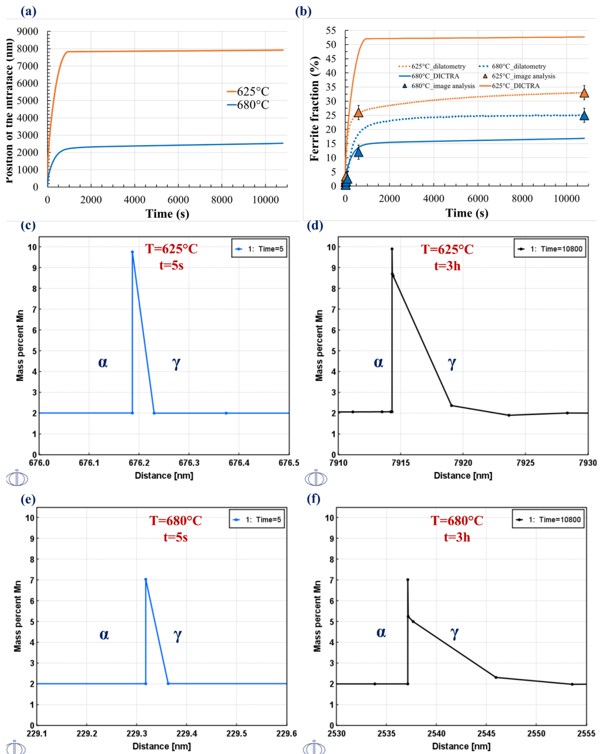
Figure 5.3. The results of DICTRA calculation for the Fe-C-Mn model alloy with the nominal composition of 0.17 wt% C and 2.0 wt% Mn: (a) temporal evolution of the ferrite/austenite interface position, (b) predicted and measured ferrite growth kinetics, (c-d) and (e-f) Mn profiles predicted by DICTRA at 5s and 3h of transformation at 625°C and 680°C, respectively.
