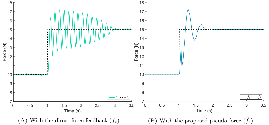
FIGURE 3.18: Response to 5N steps with \lambda = 10.5 \text{ mm.s}^{-1}.\text{N}^{-1} .
