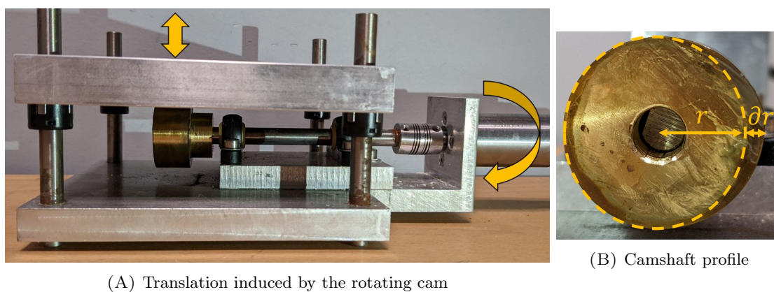
FIGURE 2.10: Breathing simulator made from a motor, a camshaft, rods, and bearings.
