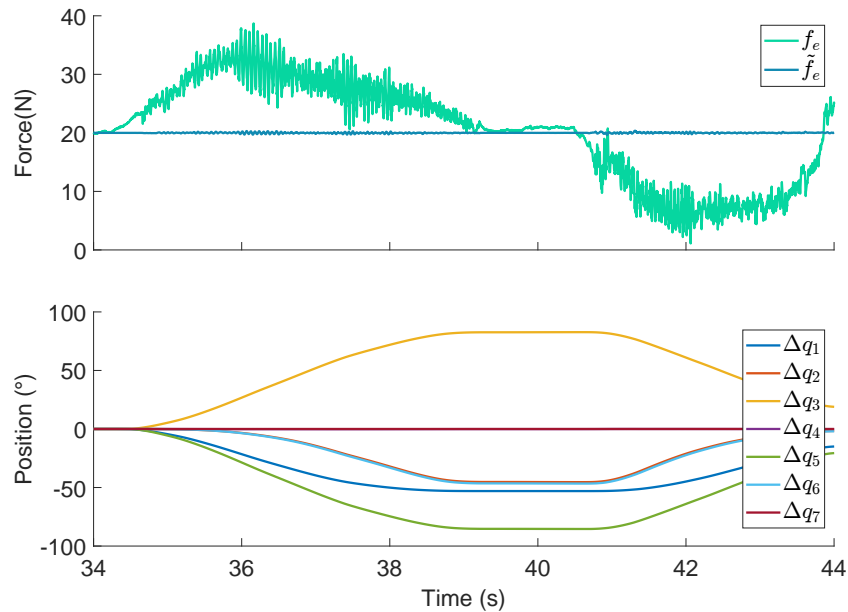
FIGURE 3.12: Controlling a distal force while a null-space motion is imposed by a human agent applying forces on the robot intermediate bodies
