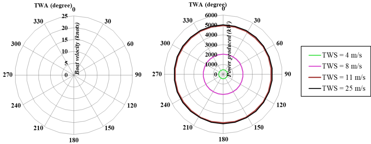
Figure 26 Zero-velocity (left) and wind turbine power production (right) polar contains data of true wind angle (TWA) and true wind speed (TWS) loaded in QtVIm for 5 MW wind turbine capacity factor assessment
