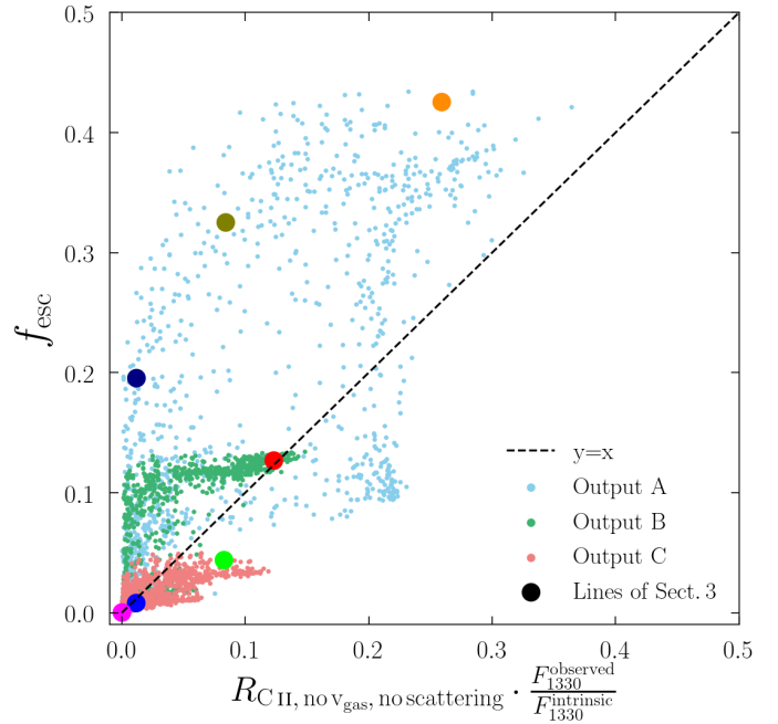
Fig. 19. As in the left panel of Fig. 15, but omitting scattering and setting gas velocity to zero.
