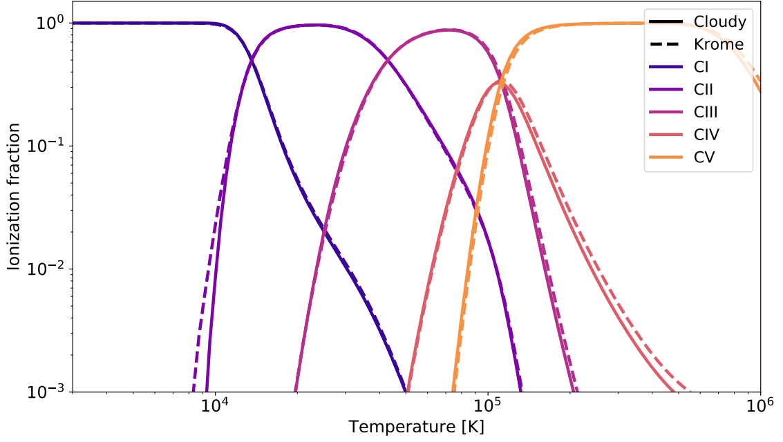
Figure 3.7: Same as Figure 3.6 but showing carbon ionisation fractions.
