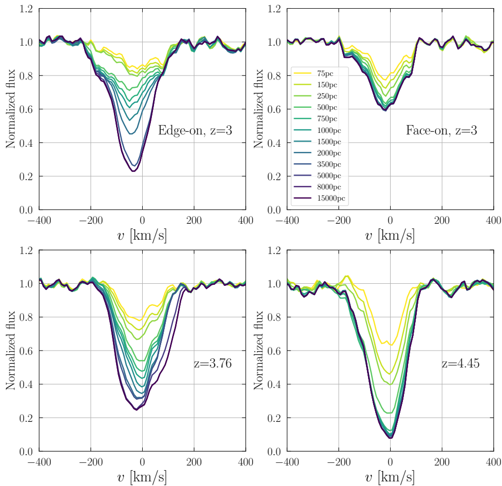
Figure 6.10: Fe II \lambda 2586 spectra of the galaxy from the zoom simulation, including the evolution of the line with radius. The radius of propagation of photons around their source is increased from 75 pc to the full virial radius, as in fiducial spectra. The top two panels show spectra of the last snapshot, at redshift 3; the left one with a direction of observation parallel to the disk and the right one perpendicular. The bottom two panels are spectra at higher redshifts. The bottom left is chosen to have an equivalent width and centroid velocity as close to the median values as possible. The bottom right one was selected randomly over 71 snapshots with 110 directions of observations for each.
