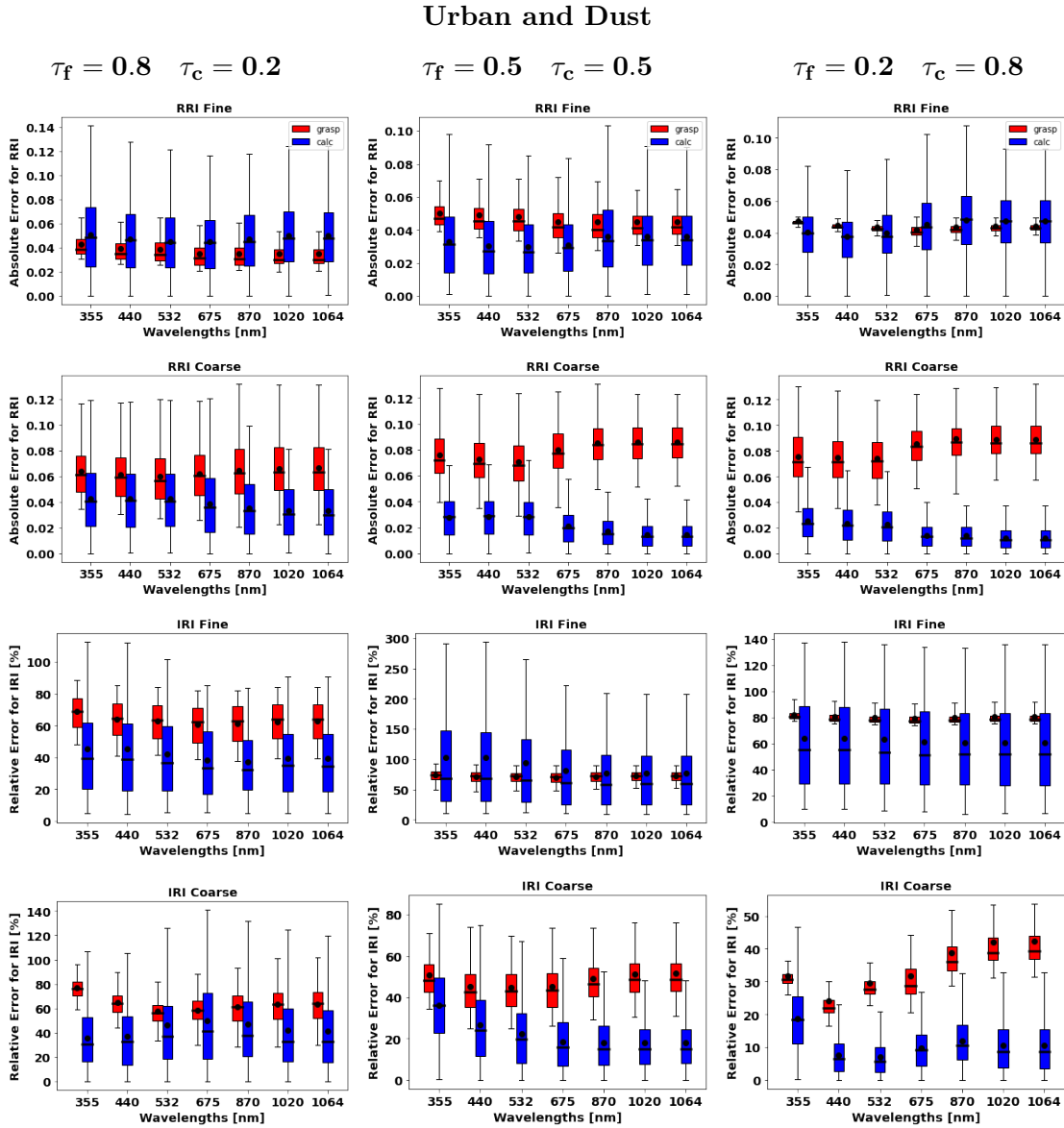
Figure 4.13: The comparison of estimated and actual error distributions for spectrally dependent aerosol parameters retrieved from measurements by sun/sky photometer simulated and lidar for a mixture of Urban-Dust aerosol. The distributions were obtained using 300 realizations of added random errors. The median values of the errors are shown by a line in the boxplot along with the 25 – 75 th percentiles indicate by a box and 5 – 95 th percentiles indicated using whiskers. The red color shows the error estimates provided by GRASP and the blue shows the calculated actual errors (Eq. 4.1).
