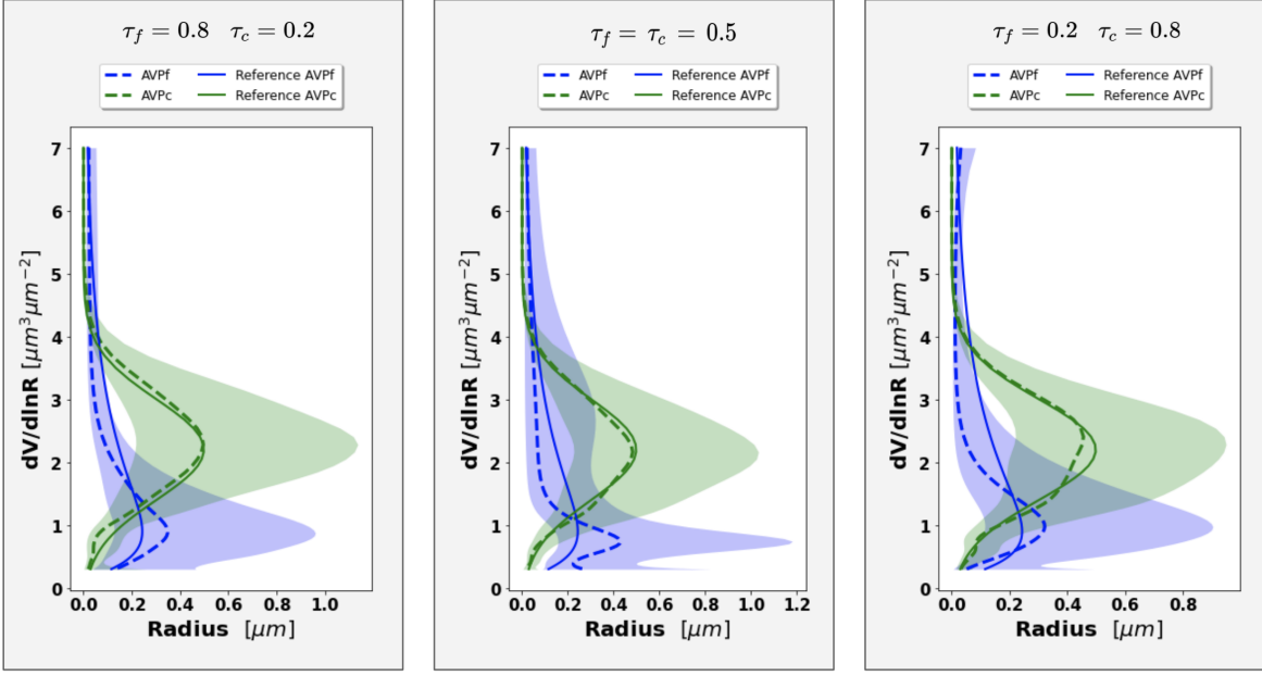
Figure 4.33: Aerosol vertical profiles (AVP) from simulated sun/sky photometer and lidar data with assumed random noise and bias in AOD, radiances and lidar simulated data for BB-Dust for \tau(440) = 1.0 . Retrievals after adding positive bias +0.01 in AOD, +5\% in RAD and +0.2 , +0.15 and 0.1 for each lidar wavelength: 355\text{ nm} , 532\text{ nm} and 1064\text{ nm} respectively. The solid lines are the simulated properties (SD, RRI, IRI, SSA and LR), the dashed lines are the retrieved parameters. The shaded area indicates total errors estimated by GRASP algorithm.
