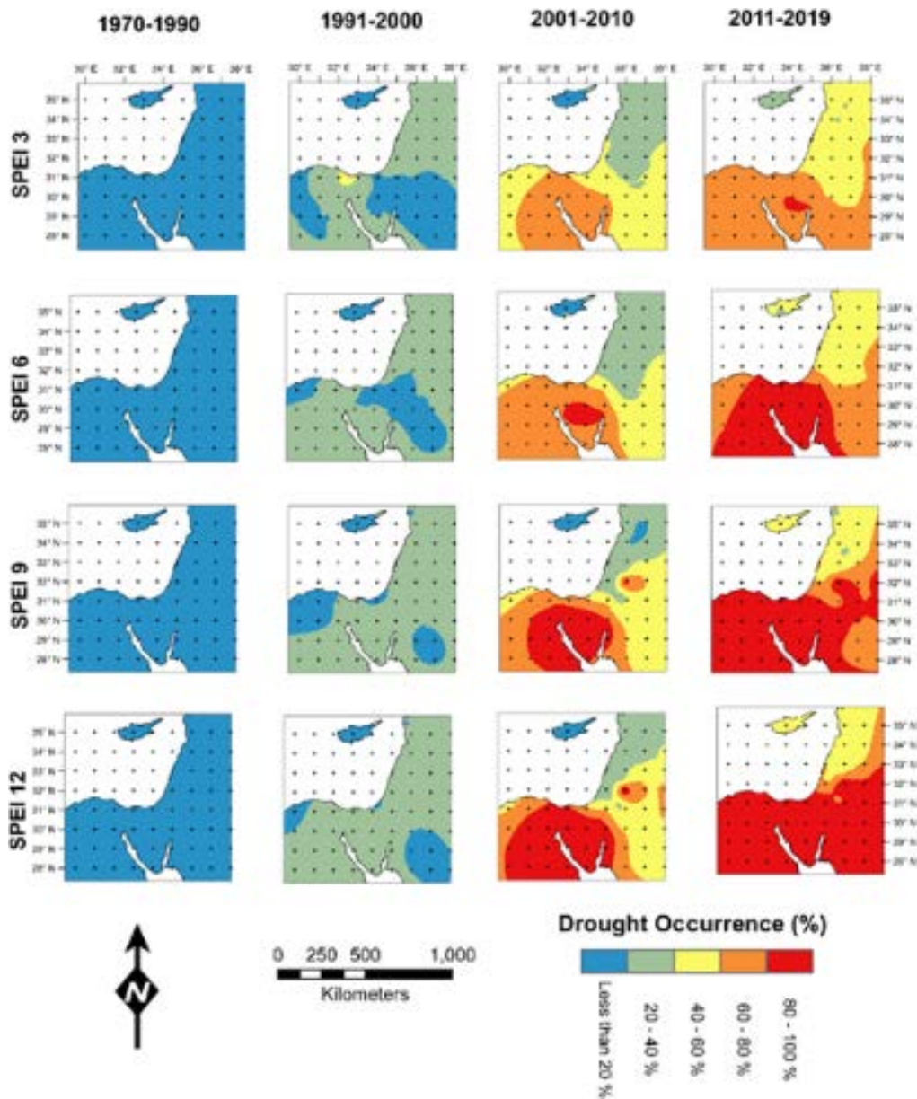
Figure 2.10. Drought occurrence in the MENA
