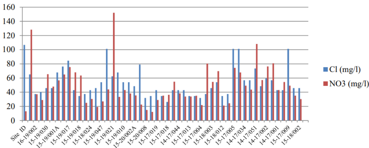
Figure 2.8. Average annual concentrations of \text{NO}_3 and Cl in groundwater wells in Tulkarm and Qalqiliya
