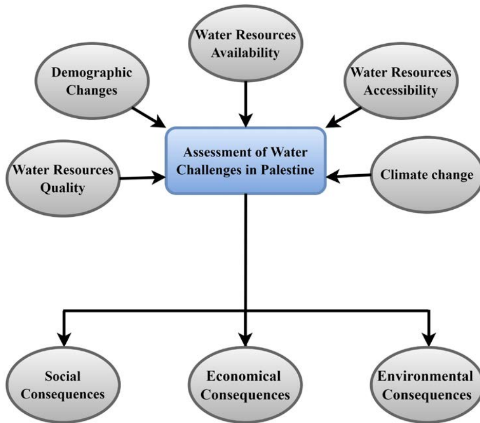
Figure 2.2. Assessment of water challenges in Palestine
