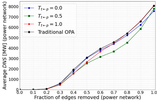
Fig. 7. Megawatts of demand not supplied within the external power network for different values of T_{t \leftarrow p} and a traditional OPA model. 95% confidence intervals are shown.
