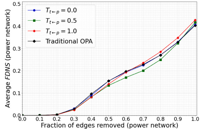
Fig. 8. Fraction of demand not supplied within the external power network for different values of T_{t \leftarrow p} and a traditional OPA model. 95% confidence intervals are shown.
