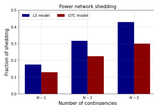
Fig. 2. Average load shedding in the power network.
