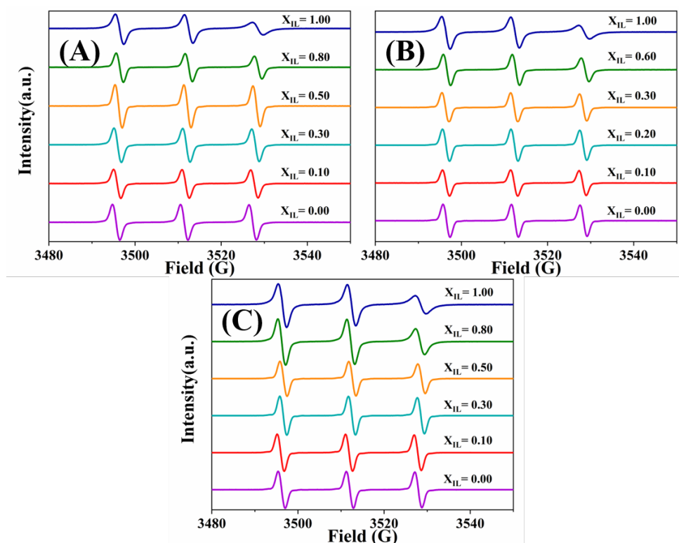
Figure C2: EPR signal of TEMPO in (A) BmimPF 6 -ACN, (B) BmimPF 6 - \gamma -BL and (C) BmimPF 6 -PC mixtures
