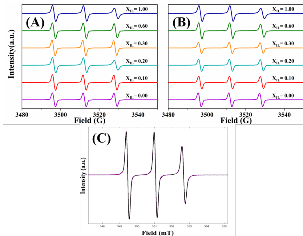
Figure C1: EPR signal of TEMPO in (A) BmimBF 4 - \gamma -BL, (B) BmimBF 4 -PC mixtures and (C) Experimental (Black) and fitted (Pink) spectra of TEMPO in pure BmimBF 4
