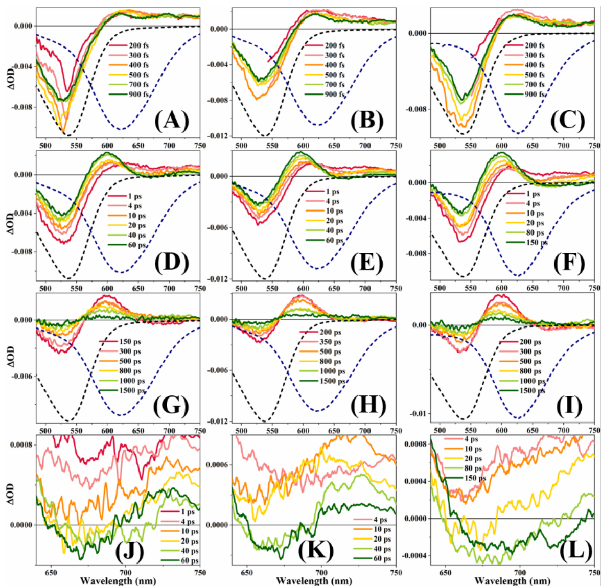
Figure B66: Transient Absorption spectra of D205 in BmimTFSI-ACN [(A), (D), (G), (J)], in BmimTFSI- \gamma -BL [(B), (E), (H), (K)] and in BmimTFSI-PC [(C), (F), (I), (L)] mixtures ( X_{IL}=0.80 ). [(A), (B), (C)] short timescale, [(D), (E), (F)] middle timescale, [(G), (H), (I)] long timescale and [(J), (K), (L)] solvation timescale. Dashed spectra are steady state absorption (black) and emission (blue) spectra.
