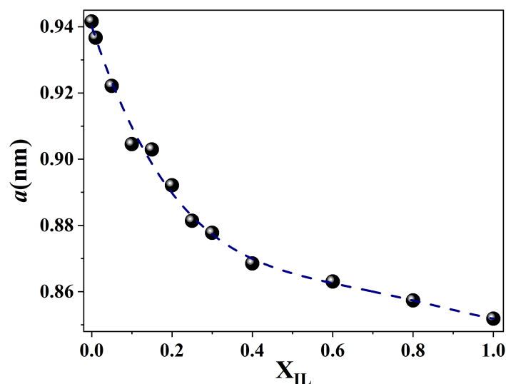
Figure 3.8: Radius of first solvation sphere in BmimBF 4 -ACN mixtures using TEMPO as a probe.
