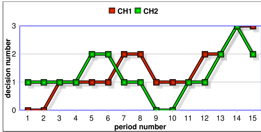
Figure 3.10: Variation of decision-making at the sink during periods, \mathcal{T} = 100 , \mathcal{V} = 5 , C = 10 .
