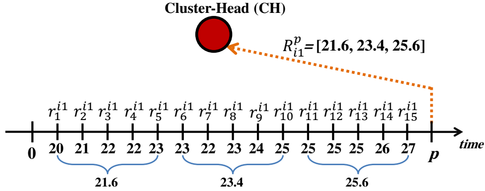
Figure 3.1: Illustrative example for divide-and-conquer algorithm.
