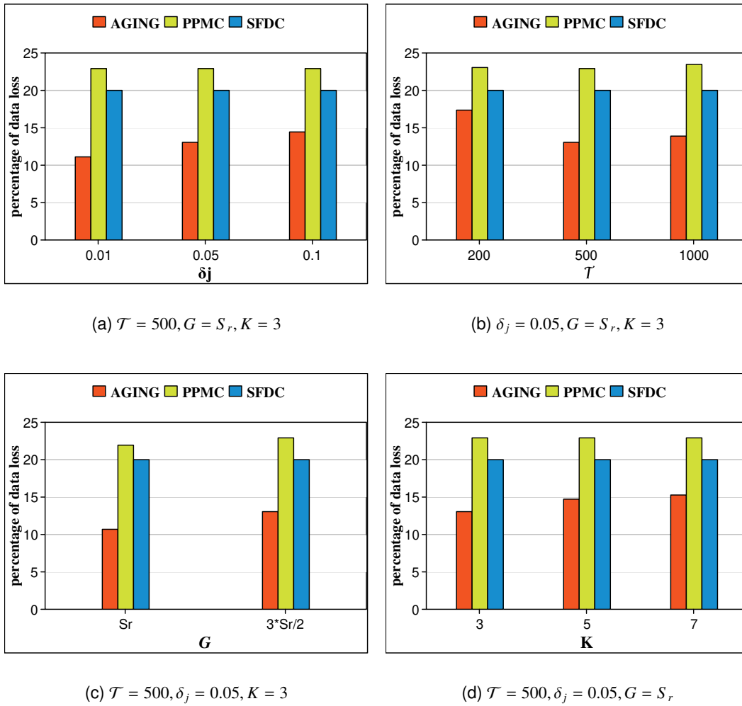
Figure 5.5: Percentage of data loss after applying scheduling strategies.
