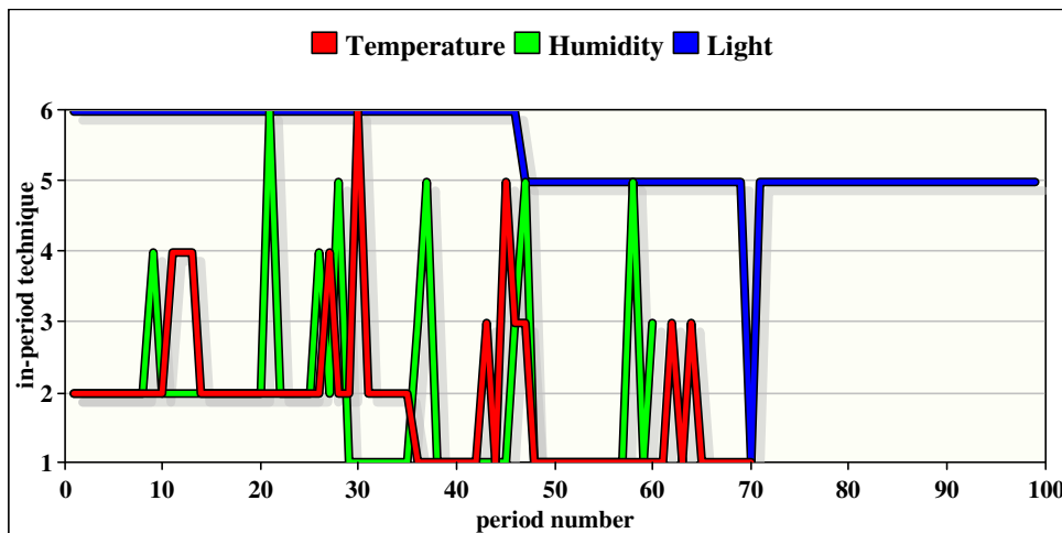
Figure 4.3: Variation of the in-period decision made by the sensor at each round, \mathcal{T} = 50 , \epsilon = 0.1 , \rho = 0.5 , d = 5 .
