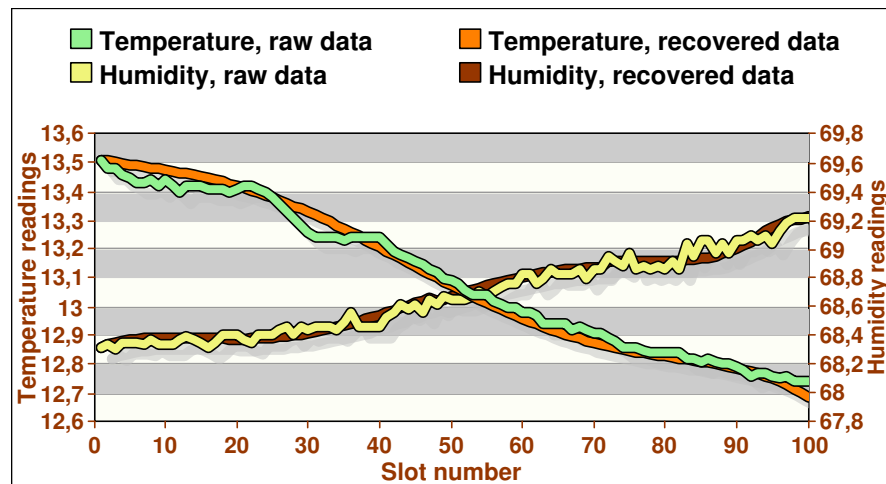
Figure 2.6: Comparison between raw and recovered data, d = 6 , \mathcal{T} = 100 .
