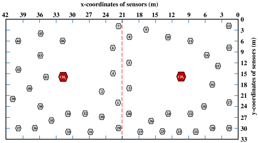
Figure 3.5: Distribution of sensor nodes and CHs in the Intel Lab.
