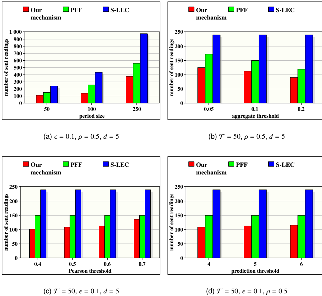
Figure 4.5: Number of readings sent from each sensor to the CH.
