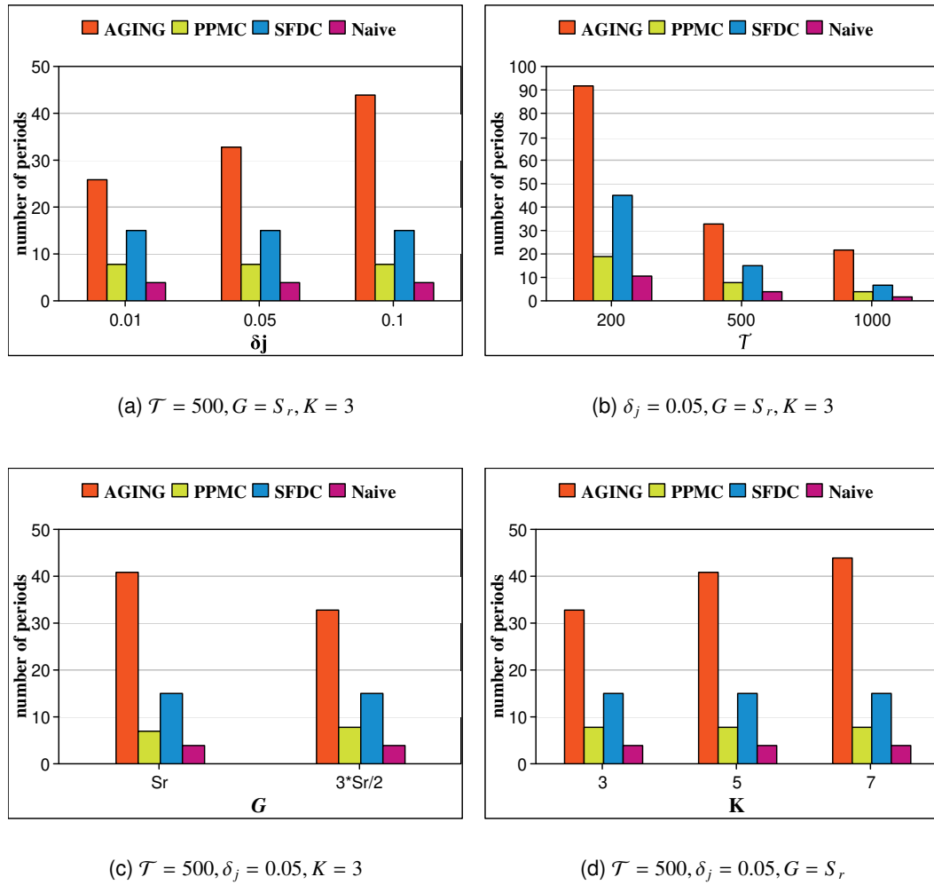
Figure 5.4: Average lifetime of each node.
