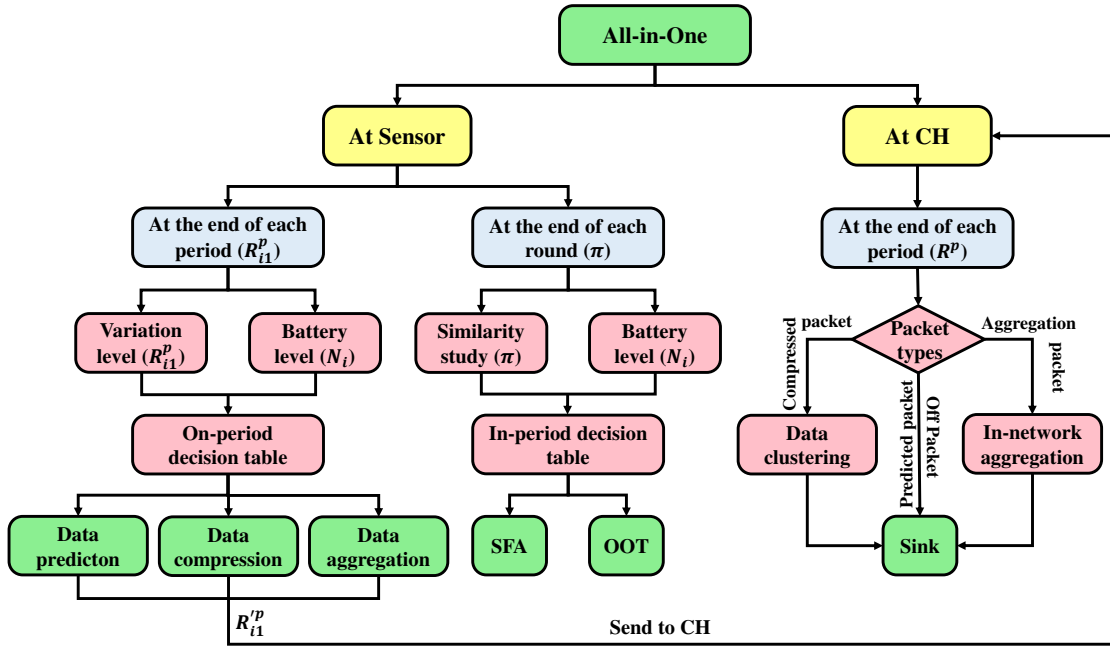
Figure 4.1: Flow diagram of All-in-One mechanism.
