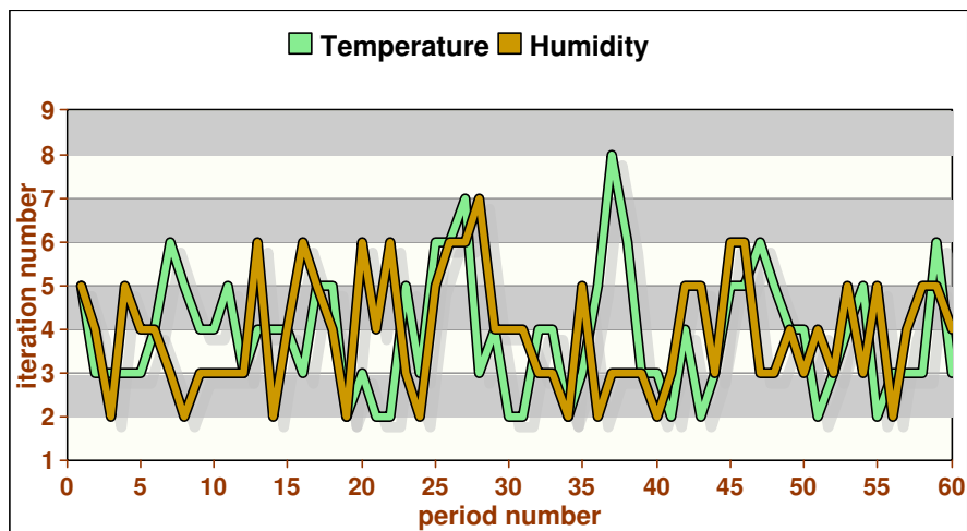
Figure 2.7: Number of iterations in applying PK-means, \mathcal{T} = 100 , d = 6 , K = 3 .
