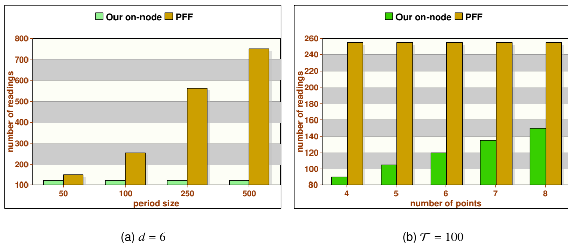
Figure 2.3: Number of readings periodically sent to the CH.
