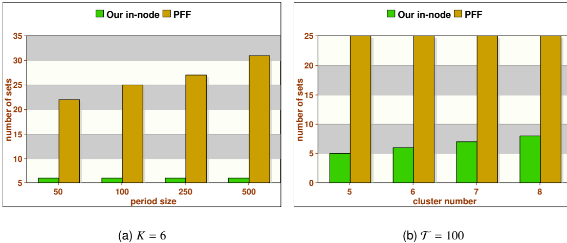
Figure 2.4: Periodic number of sets sent to the sink, d = 6 .
