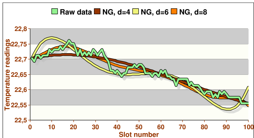
Figure 2.2: Comparison between raw and Newton Gregory generated data, \mathcal{T} = 100
