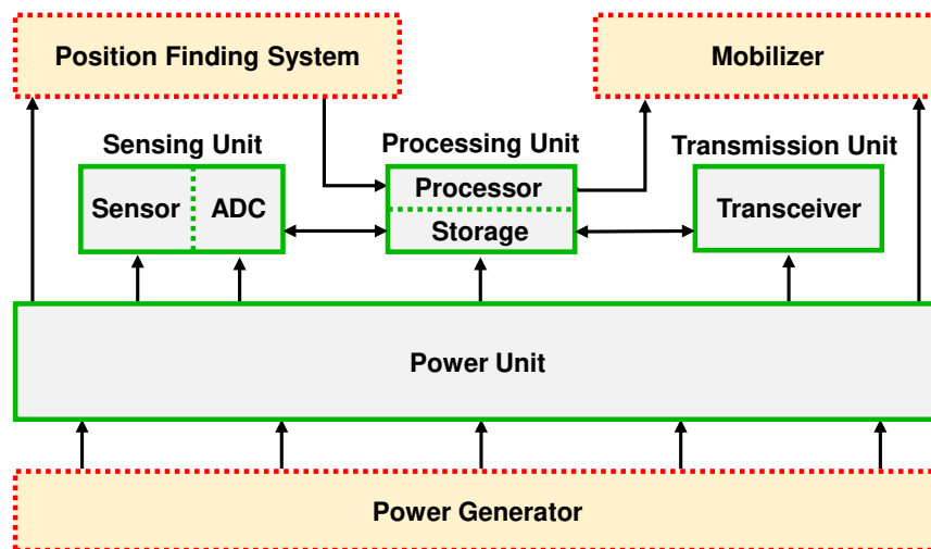
Figure 1.1: Sensor node architecture.
