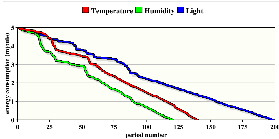
Figure 4.6: Remaining energy in a sensor in function of the period progress, \mathcal{T} = 50 , \epsilon = 0.1 , \rho = 0.5 , d = 5 .
