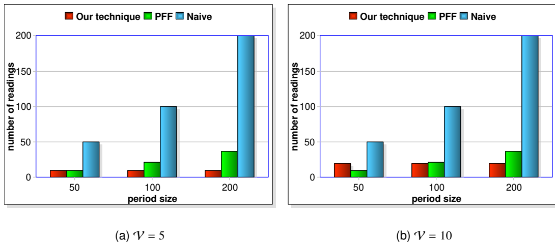
Figure 3.6: Number of periodic readings sent from each sensor to the CH.
