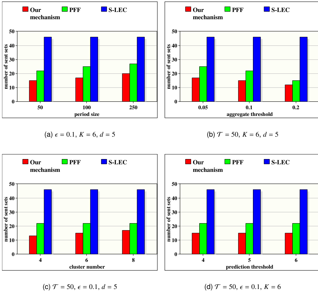
Figure 4.8: Number of sets sent periodically from the CH to the sink.
