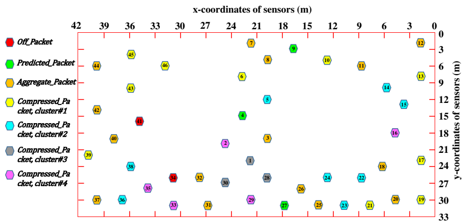
Figure 4.9: Illustrative example of packet types received by the CH during a period and after applying K-means over the compressed packets, K = 4 .
