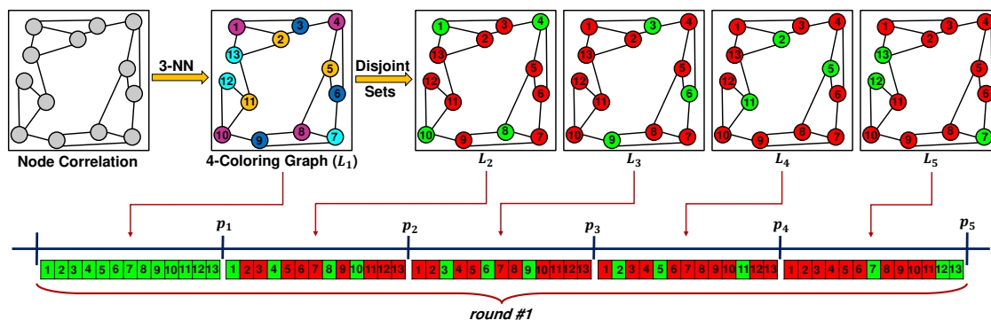
Figure 5.2: Illustrative example of node correlation and scheduling.
