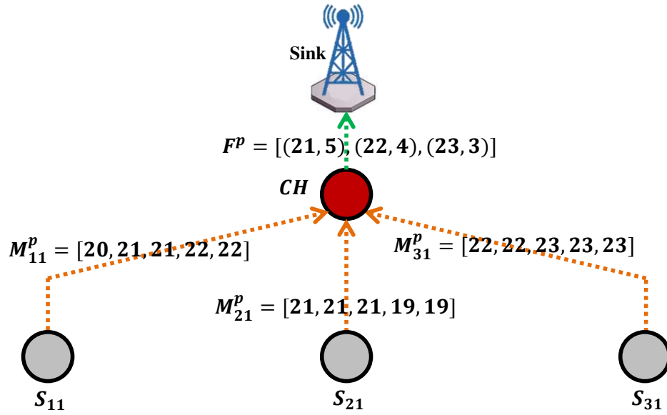
Figure 3.2: Illustrative example for support-confidence algorithm.
