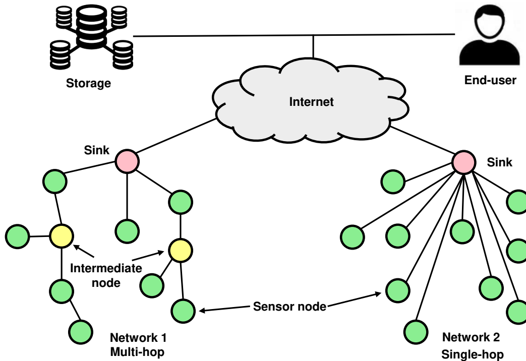
Figure 1.2: Typical sensing-based networks: single-hop vs and multi-hop communication.
