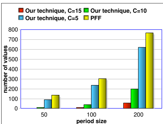
(c) CH_2, \mathcal{V} = 5
