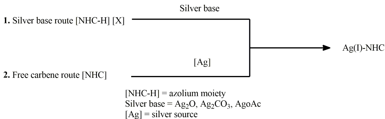
Scheme 1.1 Summary of the most common synthetic pathway for metal-carbene complexes 51
