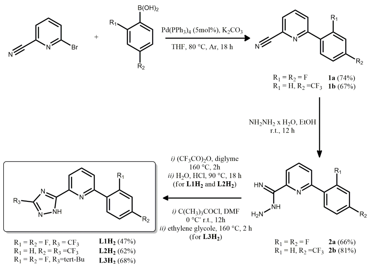
Scheme 5. Synthetic procedure for the triazolyl derivative ligands \text{L1H}_2 , \text{L2H}_2 and \text{L3H}_2 .
