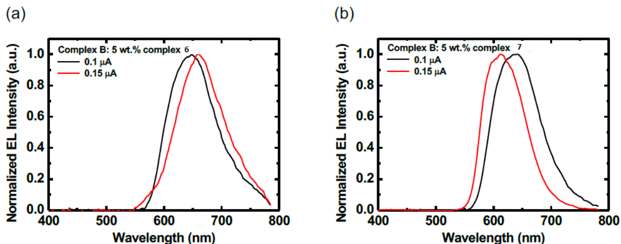
Figure 4.17 EL spectra of the host-guest LECs based on host complex B doped with 5 wt.% guest complex (a) 6 and (b) 7 under constant currents of 0.1 (black trace) and 0.15 \mu\text{A} (red trace).
