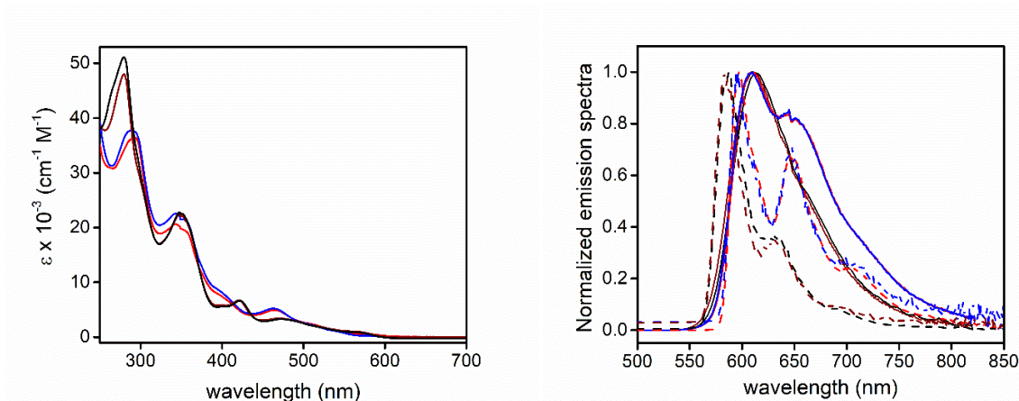
Figure 8. Electronic absorption ( left ) and emission spectra ( right ) for 4 (red trace), 5 (blue trace), 6 (dark red trace) and 7 (black trace) in dichloromethane at concentration of 3.0 \times 10^{-5} M in degassed condition (solid traces) and in 2-MeTHF glassy matrix at 77 K (dashed traces). Samples were excited at \lambda_{\text{exc}} = 420, 460 and 480 nm for compound 4,5,6 and 7 , respectively.
