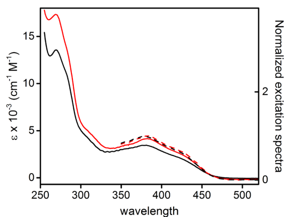
Figure ES2.13 Electronic absorption (solid line) and normalized excitation spectra (dashed line) of complex Re1 (black traces) and Re2 (red traces) in degassed \text{CH}_2\text{Cl}_2 solution at a concentration of 2 \times 10^{-5} \text{ M} at room temperature. Excitation spectra were recorded setting emission at \lambda_{\text{em}} = 660 \text{ nm} .
