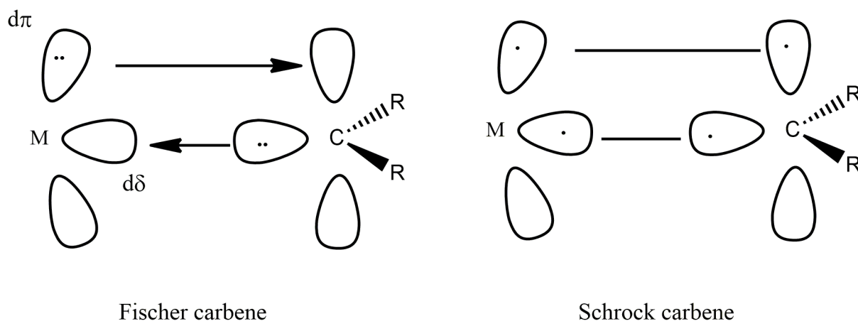
Figure 1.6 Schematic bonding representation of Fischer- and Schrock-type of carbenes.
