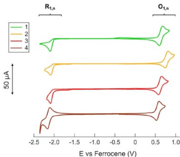
Figure 4.14. Background-subtracted cyclic voltammograms of 1 mm solutions of 1–4 in acetone/0.1 M TBAPF 6 at 0.2 Vs -1 for O 1,1–4 and R 1,1–4 processes.
