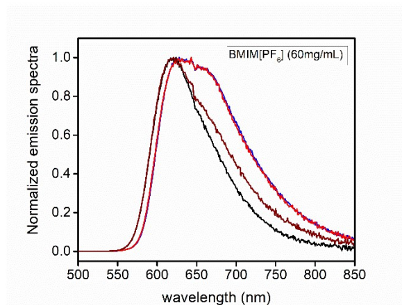
Figure 4.13 Emission spectra of spin-coated BMIM[PF 6 ] (20 wt.%) complex (80 wt.%) at total concentration of 60 mg mL -1 in acetonitrile for samples of 4 (red trace), 5 (blue trace), 6 (black trace) and 7 (dark red trace) upon \lambda_{exc} = 450 nm.
