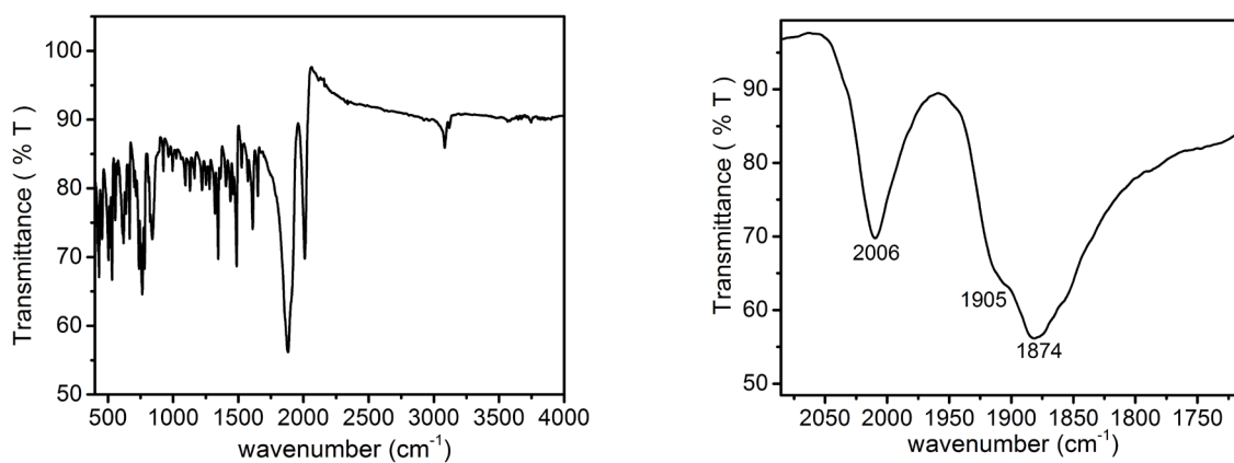
Figure ES2.9 FT-ATR-IR spectra obtained for complex Re1 in solid state as neat powder in the region 4000 – 400 \text{cm}^{-1} ( left box ) and enlarged spectrum in the \nu_{\text{CO}} = \text{C}\equiv\text{O} region 2085 – 1711 \text{cm}^{-1} ( right box ).
