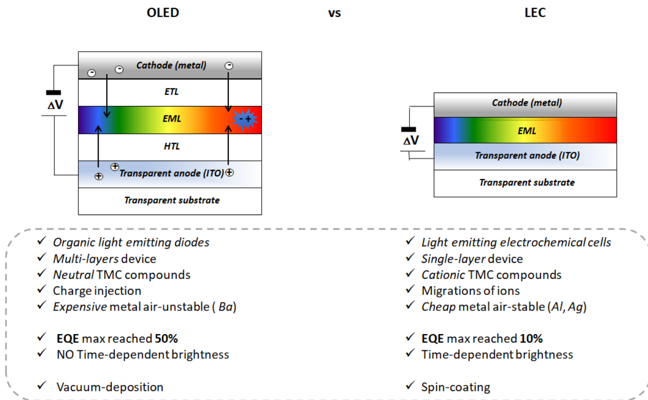
Figure 1.17 Layers structures and comparison between OLED and LEC performances.
