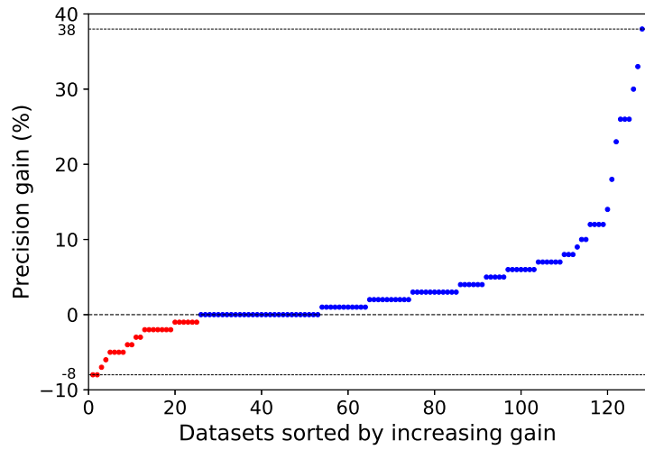
(a) Precision gain for ASAX_GSSE
