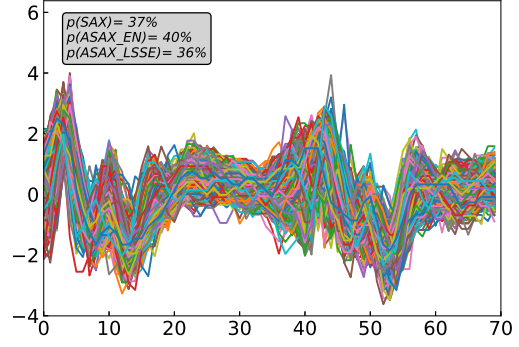
(h) SonyAIBORobotSurface1
