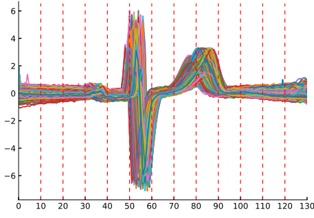
(a) SAX (PAA) segmentation on D , with 13 segments
