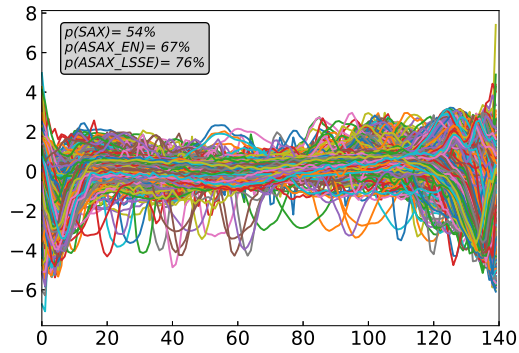
(c) ECG5000
