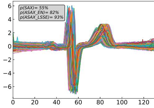
(a) ECGFiveDays
