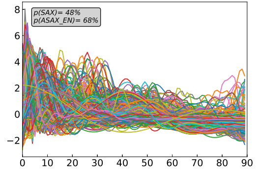
(b) MedicalImages
