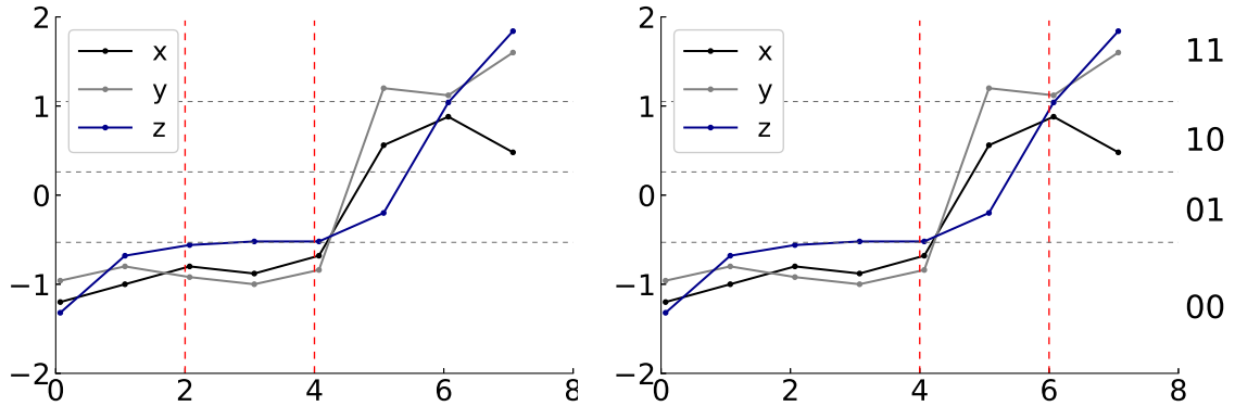
(a) Scenario 1 of ASAX_EN segmentation with 3 segments (b) Scenario 2 of ASAX_EN segmentation with 3 segments
