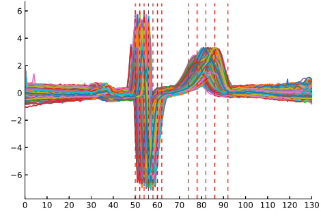
(b) ASAX_LSSE segmentation on D , with 13 segments
