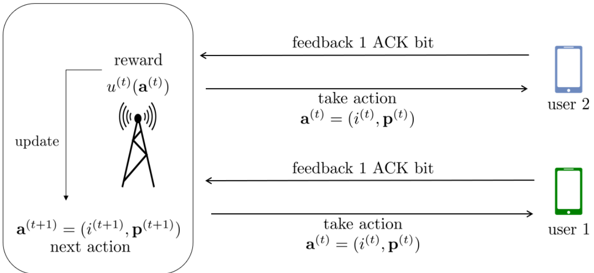
Figure 5.1: Multi-armed bandits adaptive policy.
