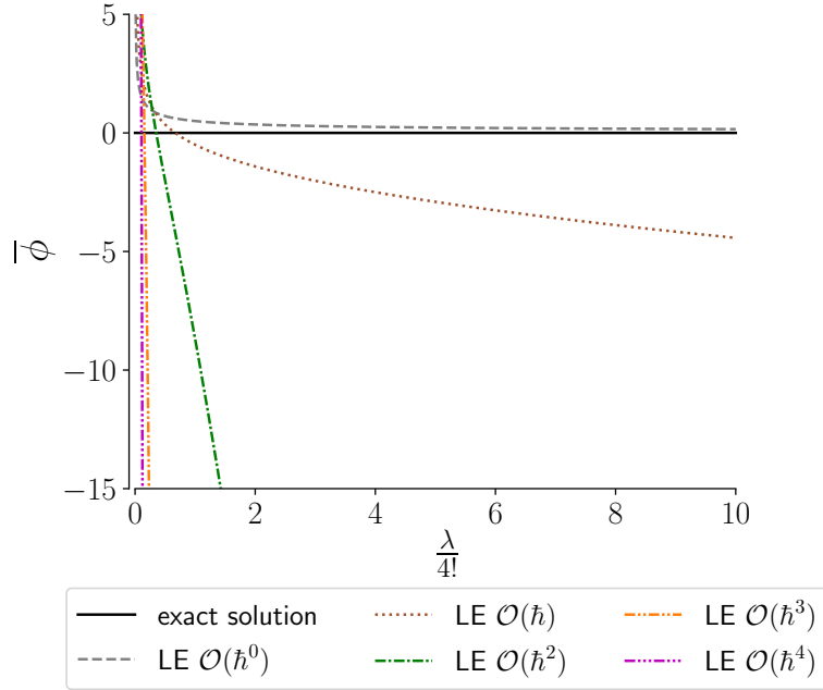
Figure 3.3: 1-point correlation function \vec{\phi} (defined from (3.98) and (3.99)) calculated at \hbar = 1 , m^2 = -1 and N = 1 ( \mathcal{R}e(\lambda) > 0 and \mathcal{I}m(\lambda) = 0 ) from the first orders of the original (and mixed) LE(s) as a function of the coupling constant \lambda/4! . Note that, at N = 1 , \vec{\phi} coincides with \bar{\phi} \equiv \left| \vec{\phi} \right| .
