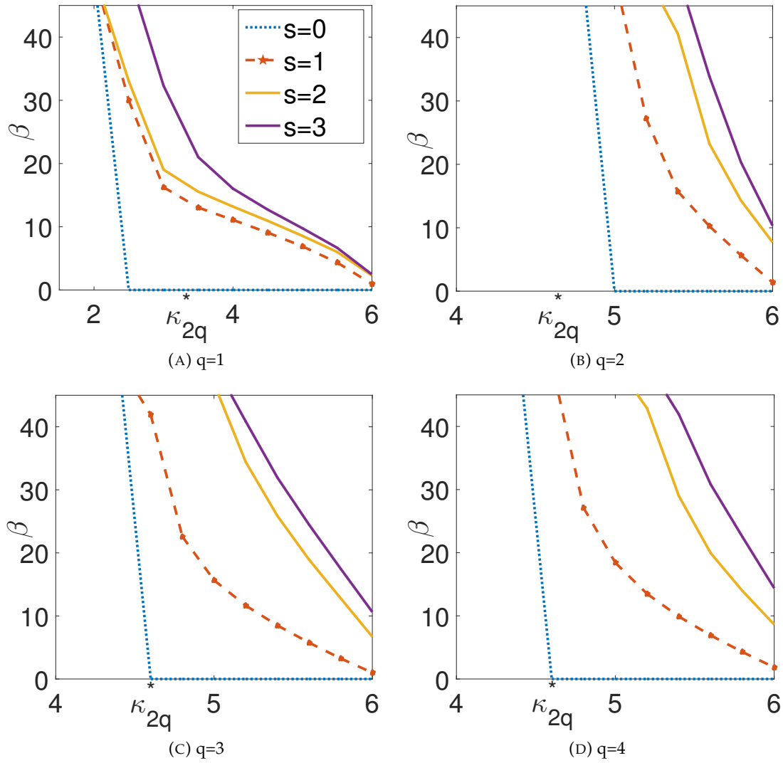
FIGURE 4.2: Example 3: Maximum allowed velocities of parameters \beta for increasing values of \kappa_{2q}^* and different degrees s on the parameter vector. Every figure is traced for a fixed degree q of state vector.
